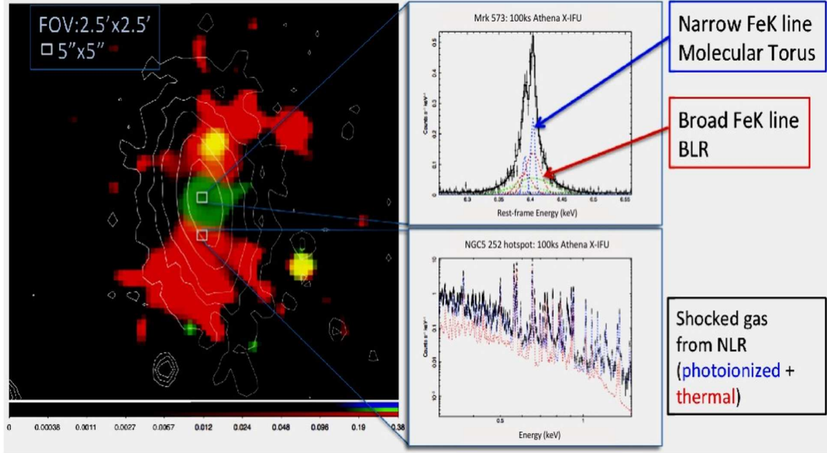
Figure 3: Left : Athena simulated color-coded image of the nearby Seyfert 2 galaxy NGC 5252 (from the Chandra image in Dadina et al. 2010). The soft X-rays are known to trace the [OIII] ionization cones forming a biconical outflow/illumination pattern driven by the AGN which impacts all over the host galaxy (DSS optical contours indicated in white). Right-top : Athena X-IFU simulated spectrum of the Fe K emission line assuming the sum of a broad plus a narrow line component, from the BLR and molecular torus respectively. Right-bottom : Athena X-IFU simulated spectrum of a part of the plume of ionized emission south of the nucleus and attributed to 25% of shock (thermal) emission plus 75% of photoionized emission. Adapted from Cappi et al. (2013).
