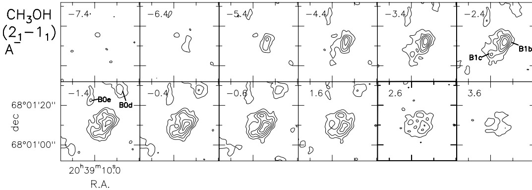
Figure 6. Channel map of the B1 clump of the L1157 outflow in the CH 3 OH (2 1 –1 1 )A – at 96.582 GHz. The thick box points out the ambient velocity emission. First level is 0.01 \text{ Jy beam}^{-1} ( 3\sigma ), level steps are 0.015 \text{ Jy beam}^{-1} .
