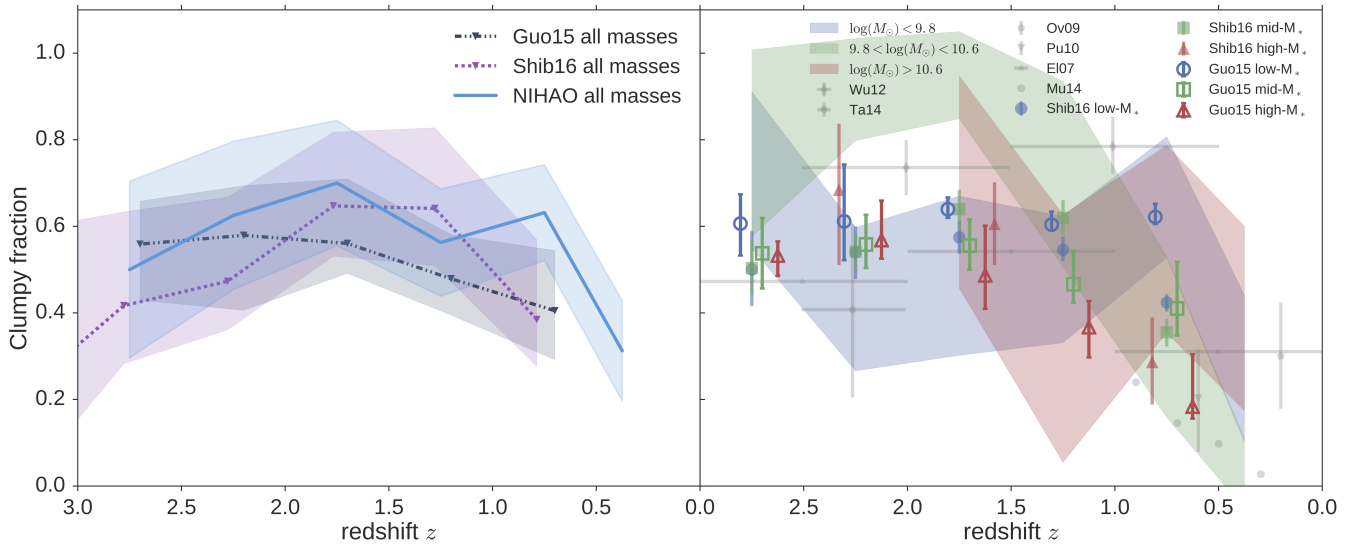
Figure 6. Evolution of the fraction of galaxies with at least one observed off-center clump. The left panel shows the evolution of the clumpy fraction for the whole NIHAO sample (blue line) compared to observations from Guo et al. (2015) (black dash-dotted line) and Shibuya et al. (2016) (purple dotted line). The shaded band shows the 1\sigma scatter. The right panel shows the evolution of the clumpy fraction splitted into different mass bins. Colored bands show the result for our simulations, colored open symbols show the according values from Guo et al. (2015) and colored filled symbols show the results from Shibuya et al. (2016). Grey open symbols show results from other observational studies: diamonds for Wuyts et al. (2012), squares are from Tadaki et al. (2014), pentagons are from Overzier et al. (2009), inverse triangles from Puech (2010), stars from Elmegreen et al. (2007) and dots from Murata et al. (2014).
