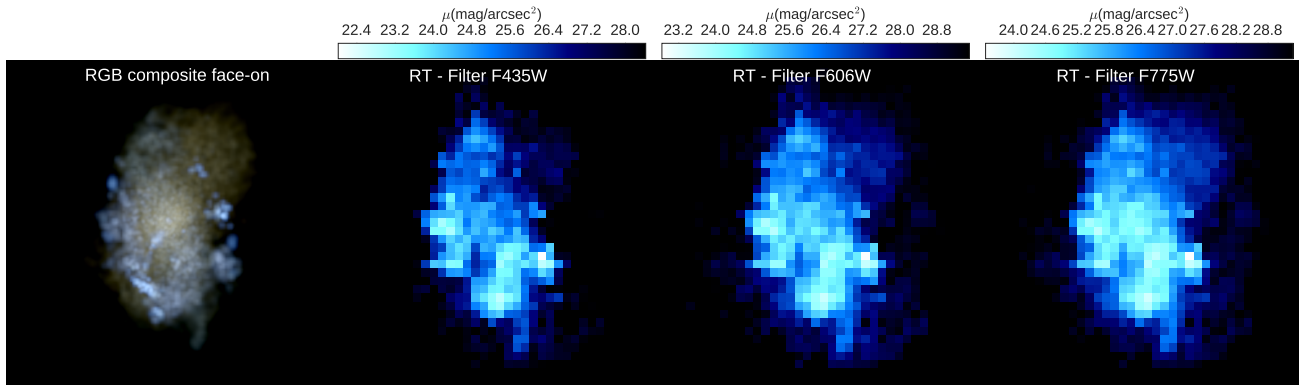
Figure 3. RGB image (left panel) and radiative transfer (RT) maps in different filters. The second panel shows the map of the F435W filter, the third panel shows the F606W image and the most right panel shows the F775W filter. Image sizes are 20 x 20 kpc.
