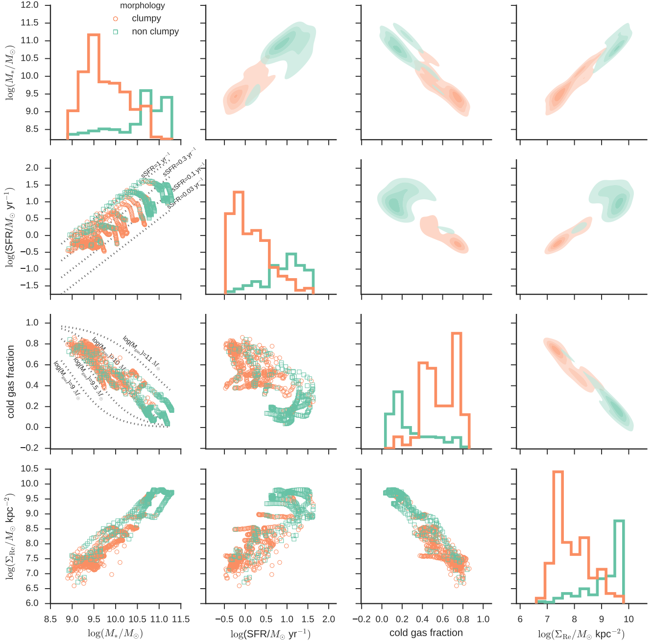
Figure 10. Properties of host galaxies and their correlation with clumpy morphology for all galaxies and all redshifts in our sample. We show correlations of stellar mass (left column), SFR (second column), cold gas fraction (third column) and the mean surface density within the half mass radius (right column) with each of the other quantities and distinguish clumpy from non-clumpy galaxies. Red colored points and lines show galaxies with a clumpy morphology (at least one off center clump) and green squares/lines show non clumpy galaxies. The lower left triangle shows all snapshots for all galaxies with single dots while the upper right triangle shows a kernel-density estimation of the point distribution. The diagonal shows the marginal histogram of the property of the given column.
