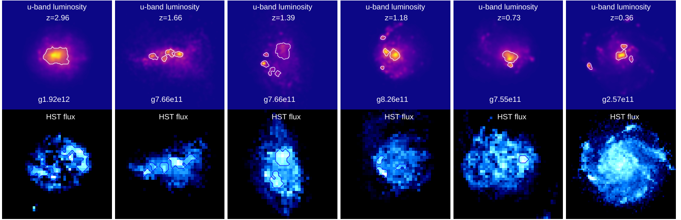
Figure 5. Comparison between clumps in the rest frame u-band luminosity maps (upper panels) and clumps in the radiative transfer (RT) images (lower panels). For the RT images the galaxies were redshifted to the proper redshift of the snapshot and observed in the same filter bands as the observations by Guo et al. (2015) accounting for dust absorption, scattering and cosmological redshift. For galaxies in the redshift range 3 < z < 2 we selected the F775W filter, for 2 < z < 1 we selected F606W and for z < 1 we selected F435W, where the redshift of each panel is indicated in the u-band maps.
