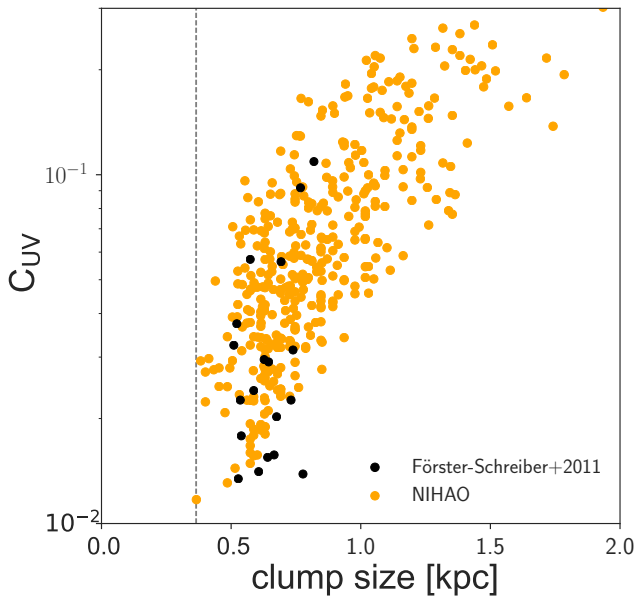
Figure 7. Clump contribution to the rest-frame dust attenuated UV light of galaxies as a function of clump size for the NIHAO sample (orange dots) and observations from Förster Schreiber et al. (2011) (black dots). The gray dashed line indicates the lower limit on clump sizes set by our clump finding procedure.
