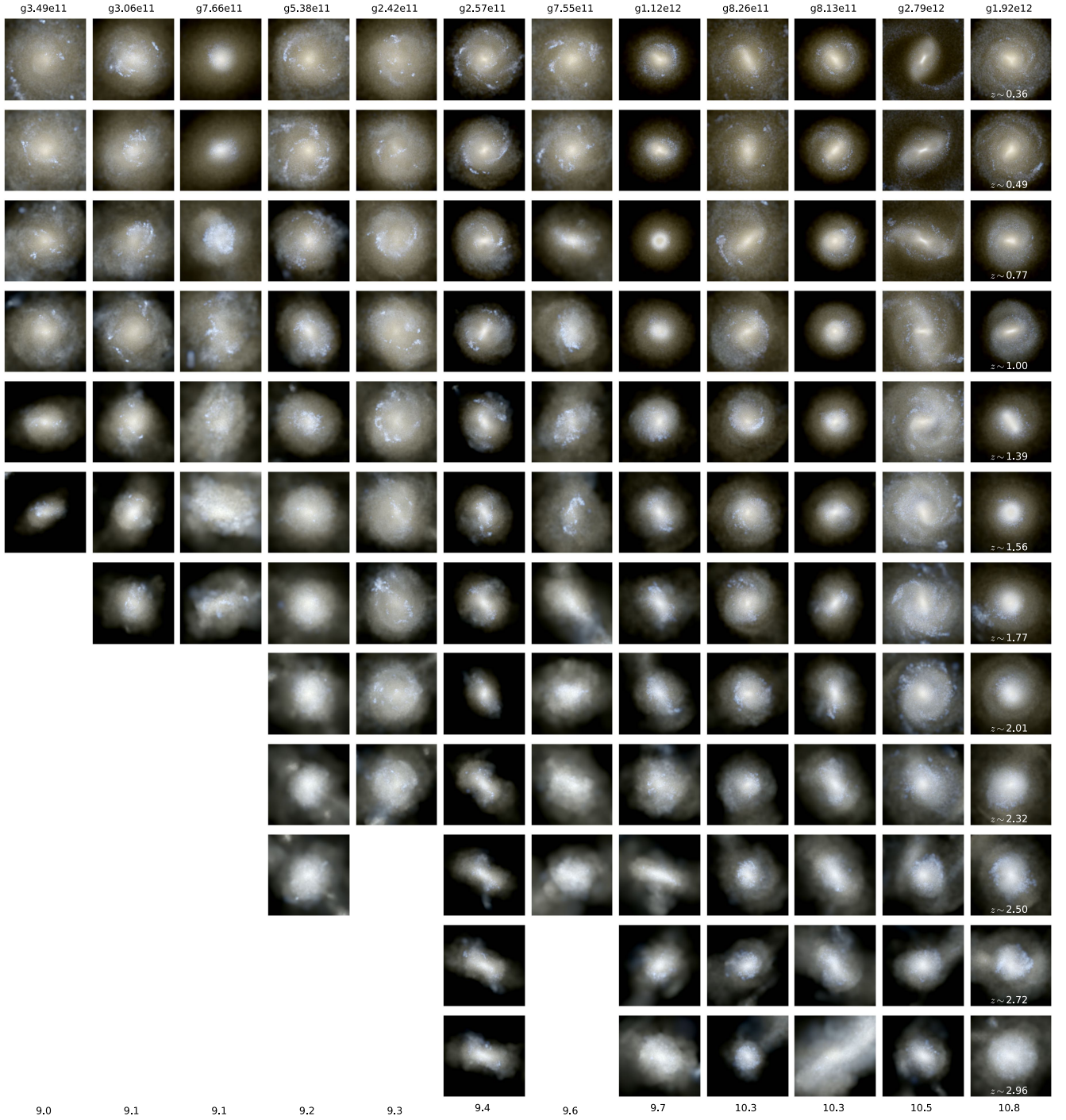
Figure A5. Impression of RGB composite images. From left to right: increasing stellar mass mass at redshift 0, from bottom to top increasing time.
