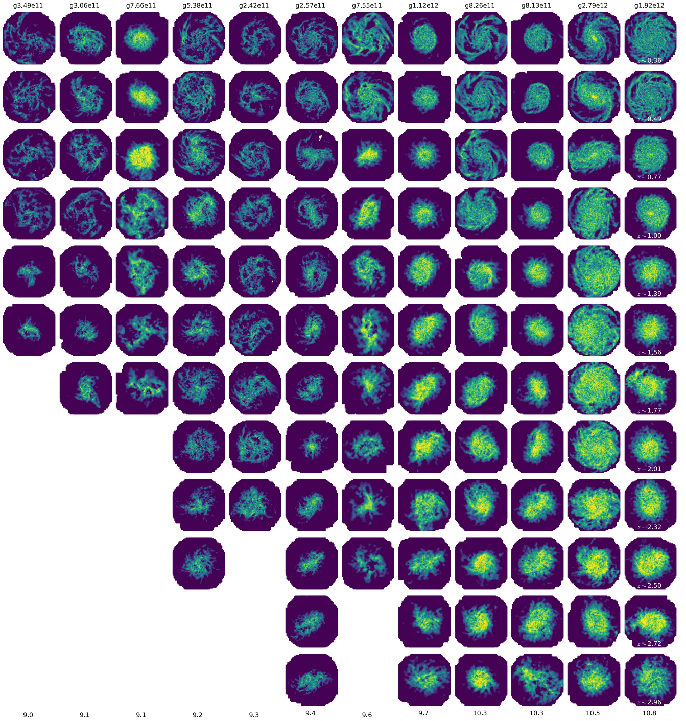
Figure A4. Impression of the cold gas surface density. From left to right: increasing stellar mass mass at redshift 0, from bottom to top increasing time. Lower bounds of gas surface densities are set to 10M_{\odot} \text{ pc}^{-2} and maximum values are set to 300M_{\odot} \text{ pc}^{-2}
