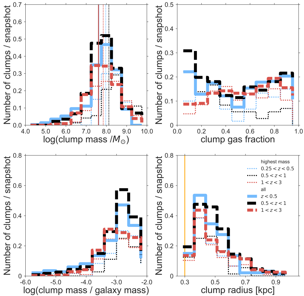
Figure 9. Clump properties for three different redshift bins ( z < 0.5 , 0.5 < z < 1 , 1 < z < 3 ) for u-band selected clumps. The top left panel shows the total clump mass, the top right shows the clump gas fraction, the bottom left panel shows the clump mass as a fraction of galaxy mass and the bottom right panel shows the clumps effective radii with the solid vertical orange line indicating the lower limit of clump sizes set by our selection criteria. Thick dashed lines show the results for the whole galaxy sample while thin dotted lines show results for only the 6 most massive galaxies. The colored solid lines in the top left panel show the median mass of clumps in the whole sample and the dotted lines show the median mass of clumps for the most massive galaxies.
