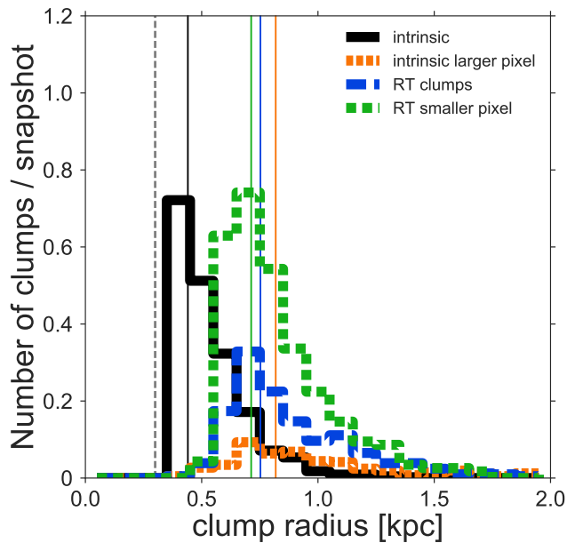
Figure A3. Comparison of clump sizes for intrinsic clumps and clumps in the RT runs for different pixel scales. The black line shows our fiducial intrinsic clump selection, the orange line shows clump sizes for intrinsic clump selection with the HST pixel scale, the blue line shows clump sizes from our fiducial clump selection in the RT run and the green line shows clump sizes for RT runs with doubled resolution (half the pixel scale of HST). The colored vertical lines show the according median clump sizes and the vertical gray dashed line shows our resolution limit on clump sizes.
