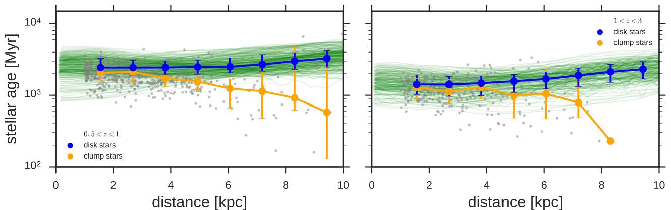
Figure 15. Mean mass weighted stellar ages of individual clumps (grey dots) and the underlying disc stars (green lines) as a function of radius in two different redshift bins. The left panel shows the mean mass weighted stellar ages in the redshift range 0.5 < z < 1 and the right panel shows the stellar ages for the redshift range 1 < z < 3 . The yellow dots show the median stellar age of individual clumps as a function of distance from the galaxy center and the blue dots show the median age of stars in the disc. The error bars show the 16th and 84th percentile.
