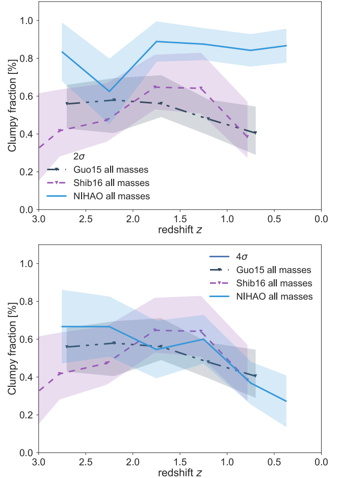
Figure A2. Evolution of the fraction of galaxies with at least one observed off-center clump for a selection threshold of 2\sigma (upper panel) and 4\sigma (lower panel). Both panels show the evolution of the clumpy fraction for the whole NIHAO sample (blue line) compared to observations from Guo et al. (2015) (black dash-dotted line) and Shibuya et al. (2016) (purple dotted line). The shaded band shows the 1\sigma scatter.
