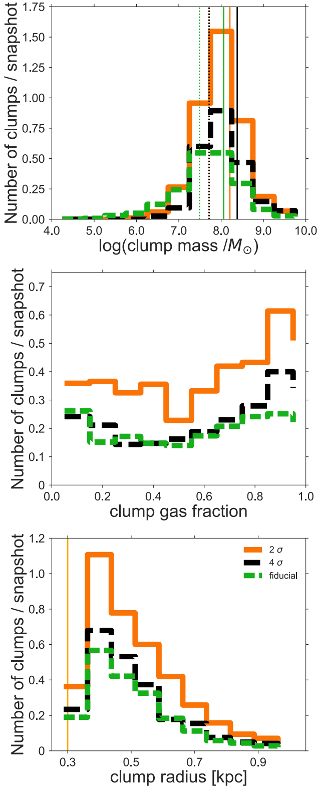
Figure A1. Clump properties for three different clump selection thresholds ( 2\sigma , 3\sigma , 4\sigma ) for u-band selected clumps. The top left panel shows the total clump mass, the middle panel shows the clump gas fraction and the bottom left panel shows the clumps effective radii with the solid vertical orange line indicating the lower limit of clump sizes set by our selection criteria. The colored solid lines in the top left panel show the median mass of clumps and the dotted lines show the mean mass of clumps.
