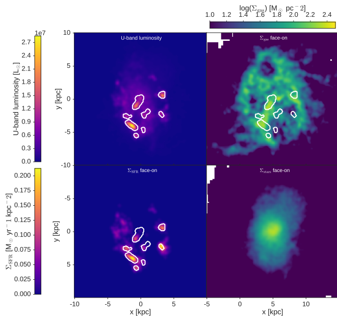
Figure 13. Face-on maps of u-band luminosity (upper left), SFR surface density (lower left), cold gas surface density (upper right) and stellar mass surface density maps (lower right). The stellar mass surface density map is extremely smooth. White contours show again the clumps selected in the u-band luminosity map.
