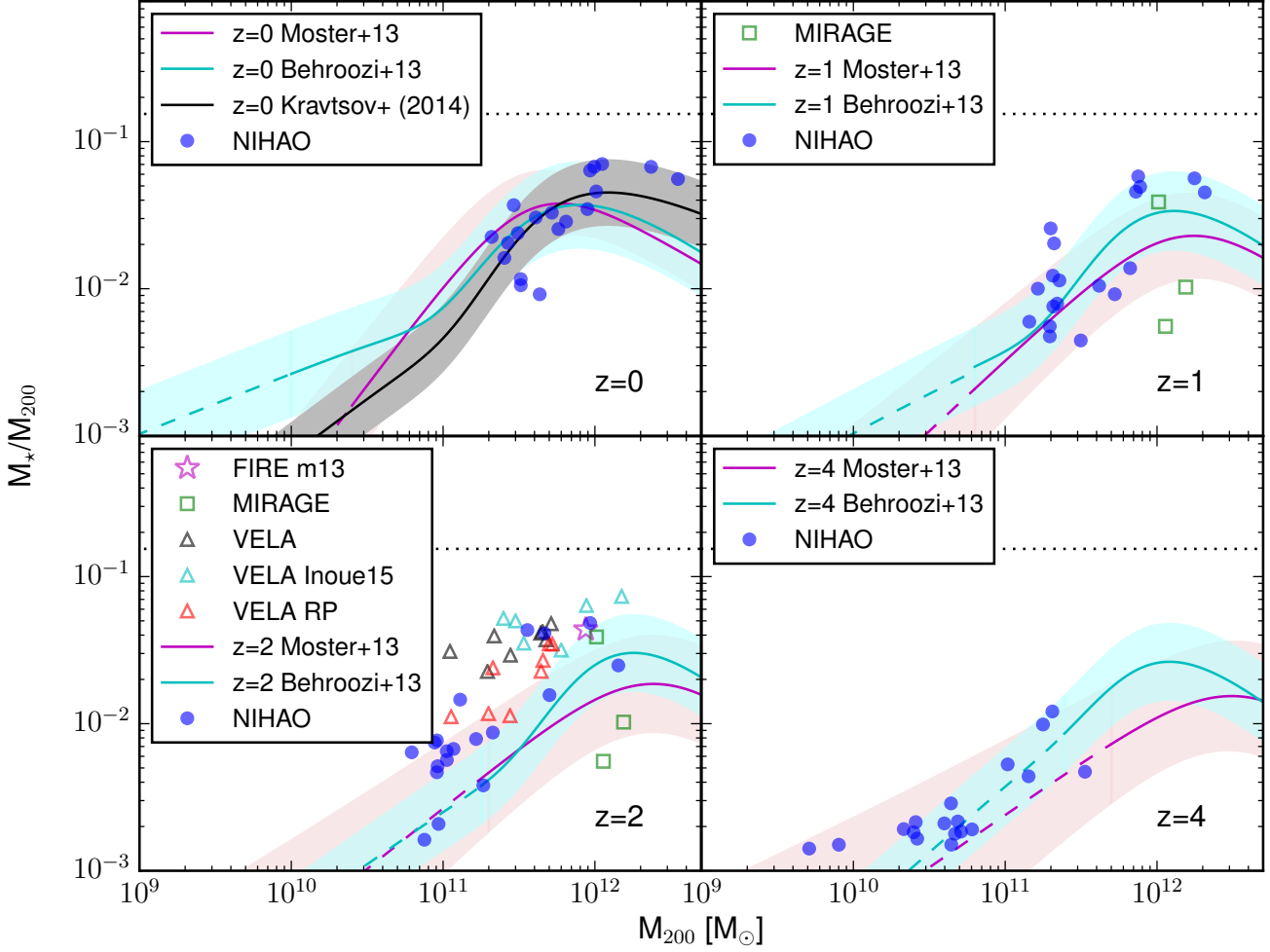
Figure 1. Evolution of the Stellar mass vs. halo mass relation for the selection of hosts. Redshift z = 0 (top left), z = 1 (top right), z = 2 (bottom left), and z = 4 (bottom right). For all redshifts shown the simulations agree well with constraints from halo abundance matching (Moster et al. 2013; Behroozi et al. 2013; Kravtsov et al. 2014). Where the relations are extrapolated into mass scales without observational constraints the lines are shown in dashed line style.
