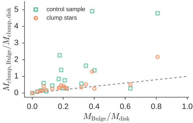
Figure 17. Contribution of clump stars to the bulge and to the disc at redshift 0. Shown is the ratio of stellar mass from clumps in the bulge and in the disc as a function of bulge to disc ratio. The red dots show the result for stellar mass from clumps while the green squares show a control sample of disc stars chosen to have the same size and radius as the clumps stars.
