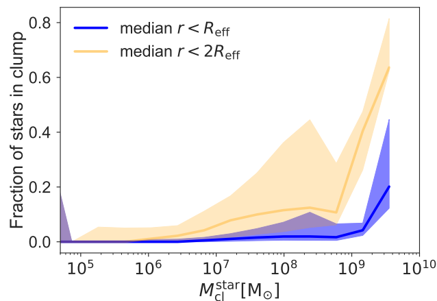
Figure 14. Fraction of clump stars still close together after 200 Myr. For every identified clump we show the fraction of clump stars still close together in the following snapshot. The blue line shows the median fraction of clump stars still within a region of 1R_{\text{eff}} around the clump’s center of mass while the yellow line shows the median fraction of clump stars still within 2R_{\text{eff}} .
