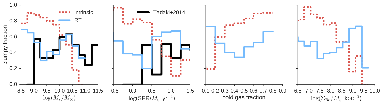
Figure 11. The fraction of clumpy galaxies as a function of host galaxy parameters for intrinsic and observed clumps in comparison to observations from Tadaki et al. (2014). From left to right we show the clumpy fraction as a function of stellar mass M_{\text{star}} , SFR, cold gas fraction and the mean surface density within the half mass radius.
