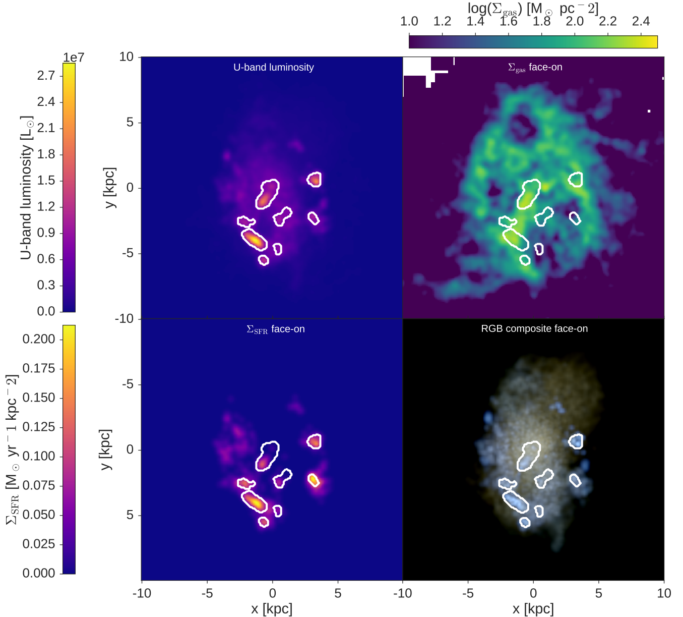
Figure 4. Face-on maps of intrinsic u-band luminosity (upper left), SFR surface density (lower left), cold gas surface density (upper right), and RGB stellar composite (lower right). The white contours show the clumps selected in the intrinsic u-band luminosity map.
