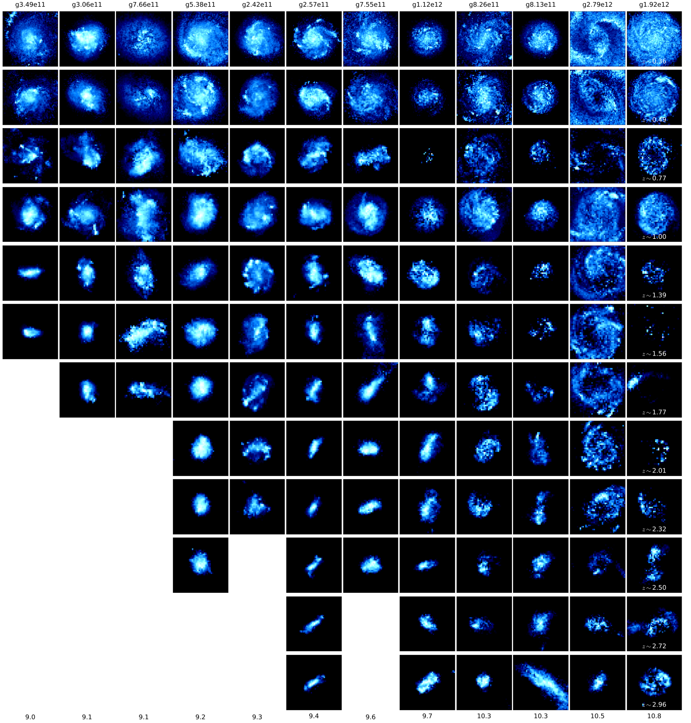
Figure A6. Impression of the outcome of the RT runs. From left to right: increasing stellar mass at redshift 0, from bottom to top increasing time. For snapshots in the redshift range 3 > z > 2 we select the F775W filter, for 2 > z > 1 we select the F606W filter and for z < 1 we select the F435W filter to detect clumps. This filter selection roughly corresponds to the rest frame UV at these redshifts (Guo et al. 2015).
