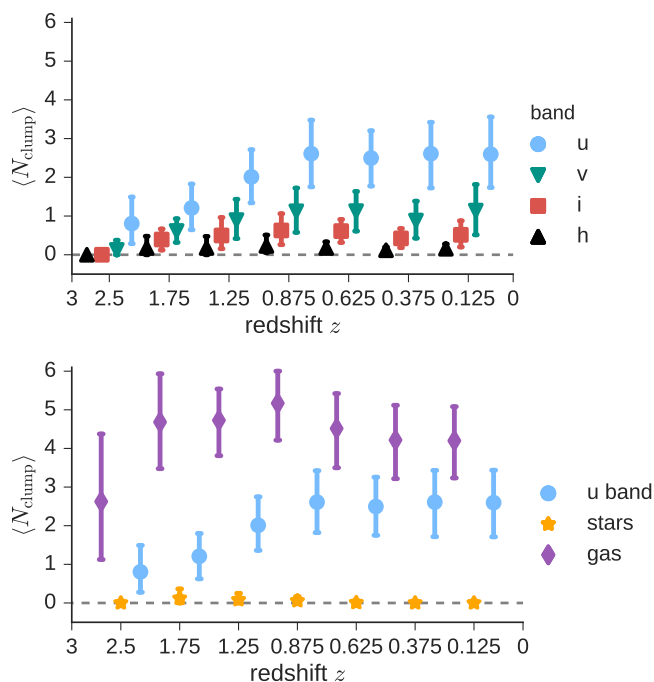
Figure 12. Mean number of clumps per galaxy for clumps selected in different wavelength bands. The upper panel shows the mean number of clumps for clump selected in the u-band (blue dots), the v-band (green lower triangles), the i-band (red squares) and the h-band (black upper triangles). The lower panel shows a comparison of the mean number of clumps selected in the u-band (blue dots) with clumps selected in the gas surface density maps (purple diamonds) and the stellar surface density maps (orange stars). The points are slightly offset to avoid overlap.
