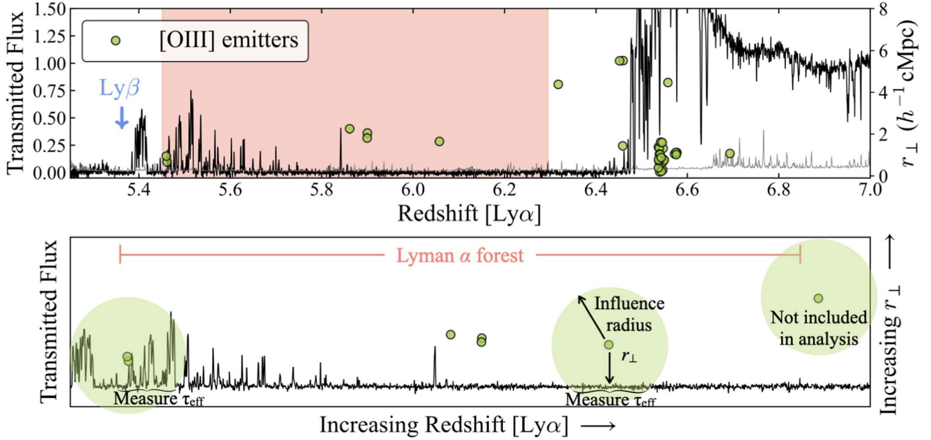
Figure 4. Top—The transmitted spectrum of an ASPIRE quasar J0226+0302. The redshift range of the \text{Ly}\alpha used in the analysis is displayed in the red-shaded region. The location of the \text{Ly}\beta emission line is marked by the blue downward arrow. The spatial locations of the [O III] emitters identified in each quasar field are denoted by the yellow-green-filled circles in terms of the [O III] emitter redshift z_{[\text{O III}]} and the transverse distance r_{\perp} between the [O III] emitter and the central quasar. Bottom—An illustrative figure for measuring the IGM transmission around the [O III] emitters within the \text{Ly}\alpha forest of J0226+0302. For each [O III] emitter identified in the quasar field, we put a sphere of a certain radius (“influence radius”) centered at the [O III] emitter. For better visualization, we only show the spheres of three [O III] emitters and the size of the sphere is only for illustrative purposes, not to scale. For an [O III] emitter of which the sphere intersects the \text{Ly}\alpha forest, we assume that the [O III] emitter is able to “influence” the \text{Ly}\alpha forest.
