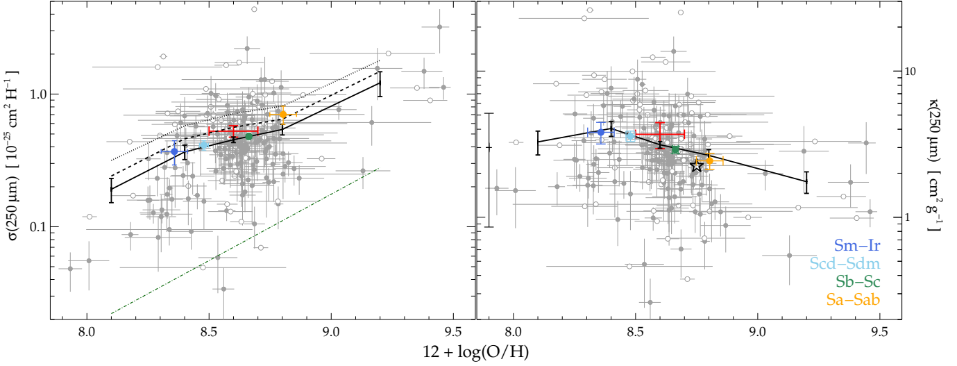
Fig. 5. Absorption cross section per H atom \sigma(250\mu\text{m}) (left panel) and per dust mass \kappa(250\mu\text{m}) (right panel) as a function of the metallicity. The two panels show individual measurements as grey dots, with the same convention for open and filled symbols as in Fig. 2. The mean (and its standard deviation) of the quantity of the y-axis for the five metallicity bins defined in Fig. 3 (black error bars connected by a solid line) is shown, and the same, but for the four morphology bins (coloured dots with error bars). We also plot the HeViCS MW estimate of Table 1 (red error bars). Left panel: we also show the mean for each metallicity bin, when the dust temperature is derived with \beta = 1.8 (dashed line) and 2.0 (dotted line), and the slope for a linear dependence of \kappa(250\mu\text{m}) on O/H (green dot-dashed line, arbitrary scale; Eqs. (4) and (5)). Right panel: the black error bar at the left shows the uncertainty in ((D/H)/(O/H))_{\text{MW}} . The star indicates the value derived from C16 after rescaling it to the assumptions of this work (see text for details).
