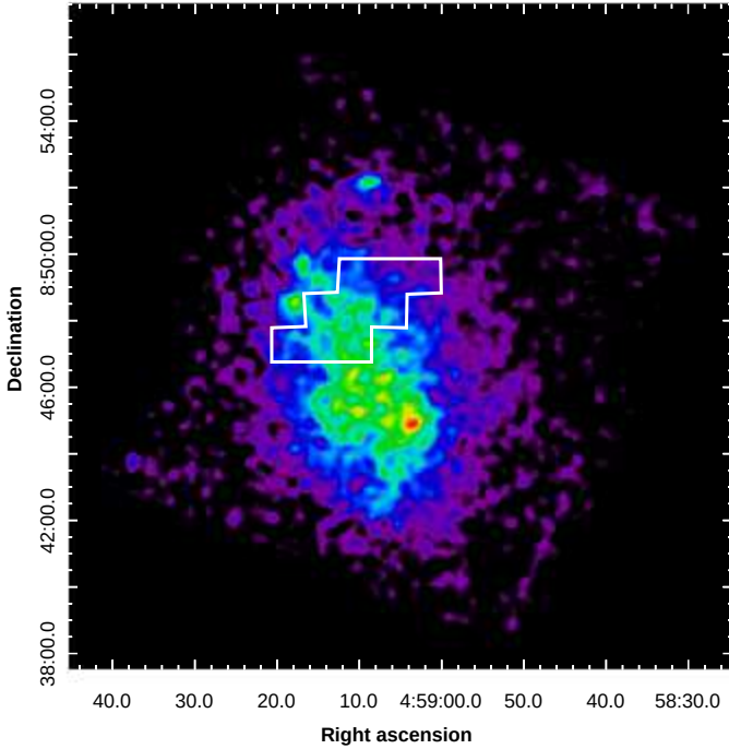
Fig. 14. Grid cells where the radio-halo emission is maximum (see text), overlaid on the NuSTAR 3–10 keV image of A523.
