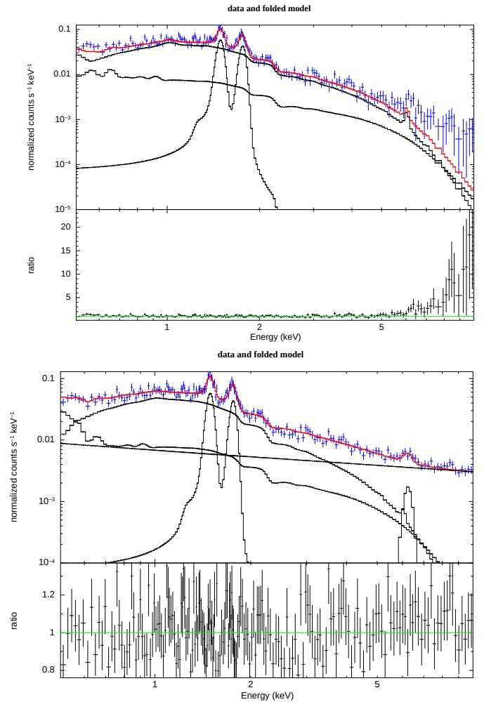
Fig. A.1. Spectral fit for the 6th annulus and for only the MOS1 instrument, performed with two different methods. Top panel: background subtraction of the ESAS-produced background spectrum. Bottom panel: using the QPB model obtained from FWC observations, obtained as described in this section. In red we show the total best-fit model. Lower panels show the data to total model ratio.
