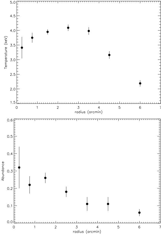
Fig. 5. Mean temperature (top panel) and abundance (bottom panel) radial profiles. The best-fit parameters are plot in function of the mean radius for each annulus, expressed in arcmin.
