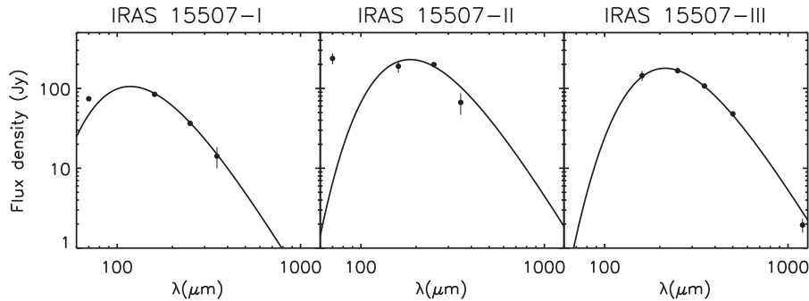
Figure 4. SEDs of the three cores observed with Herschel . The continuous lines are the best-fitting modified black bodies described in Section 3.1. The flux at 70\mu\text{m} is plotted but was not considered for the fit.
