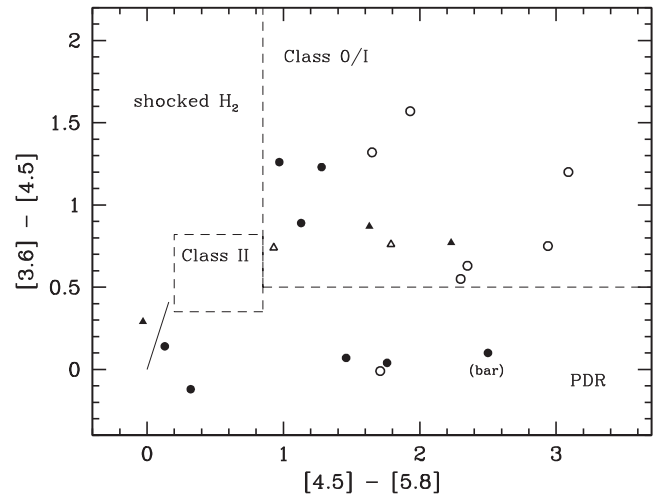
Figure 9. [3.6] - [4.5] versus [4.5] - [5.8] diagram of all sources measured in the three IRAC bands. The symbols used for sources in and outside regions CI 1, R1 and R2 are the same as in Fig. 8. The dashed rectangles mark the loci of the Class II and Class 0/I sources and the labels ‘shocked \text{H}_2 ’ and ‘PDR’ mark, respectively, the areas occupied by shocked regions emitting molecular hydrogen lines and PAH-emission-dominated photodissociation regions (Ybarra et al. 2014). The continuous line is the reddening vector (Flaherty et al. 2007).
