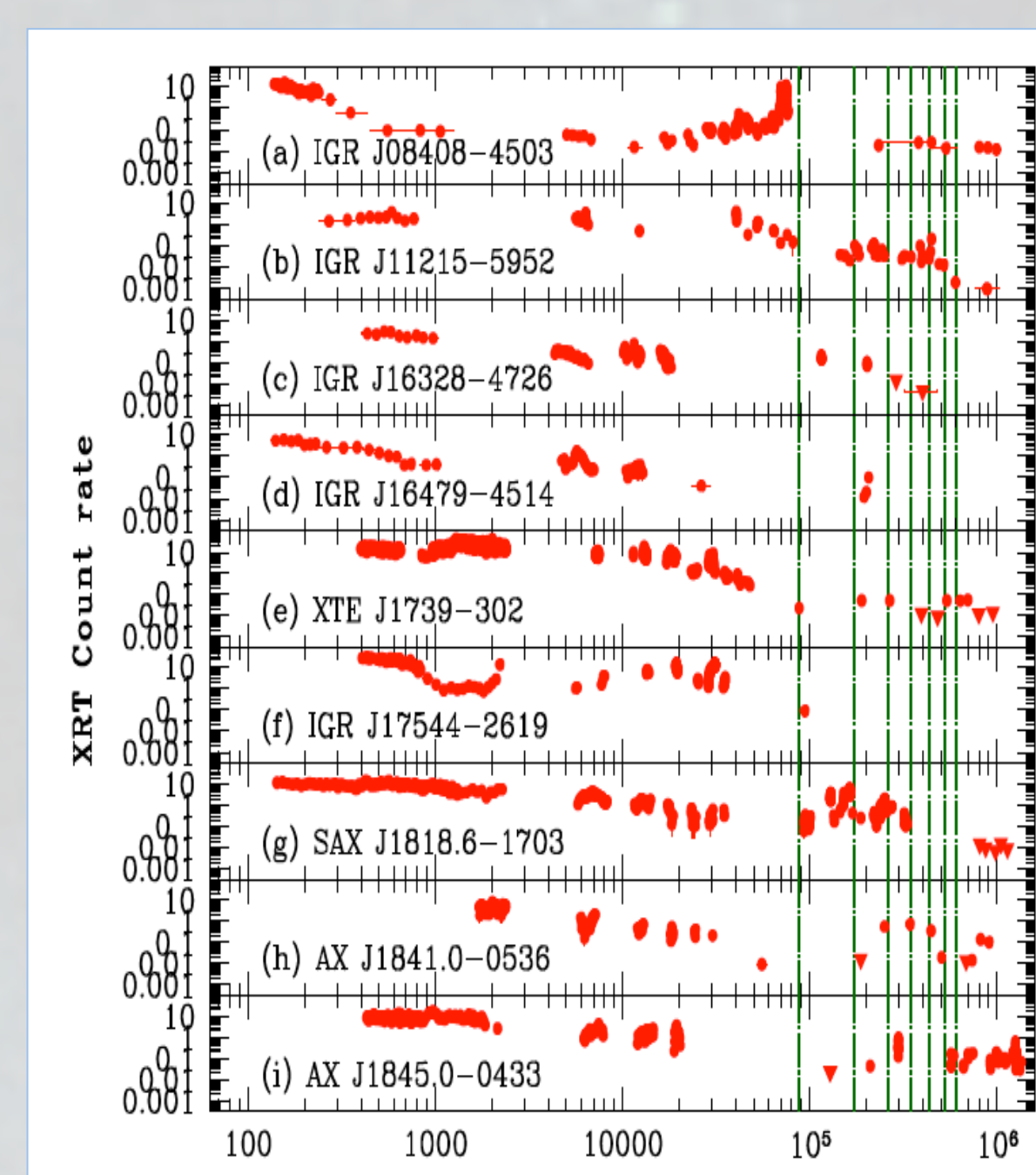
Fig. 3: Light curves of the most outstanding outbursts of SFXTs followed by Swift /XRT with starting times referred to their respective BAT triggers (IGR J11215–5952 and IGR J16418–4532 did not trigger the BAT, so data are referred to the start of the observation). Points denote detections, triangles 3- \sigma upper limits. Vertical dashed lines mark 1 day time intervals up to a week.
