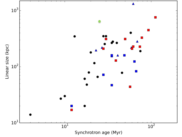
Figure 7. Linear size as a function of the synchrotron age for the sample of low-luminosity radio galaxies in Parma et al. 1999. We added the values for MaxBCG J199, whose age being a lower limit is indicated by a green circle. Squares represent FR-I sources, triangles FR-II sources, and circles sources whose classification is not clear. The colour represents the spectral type: red for type 1, blue for type 2, black for sources whose spectral classification is not clear.
