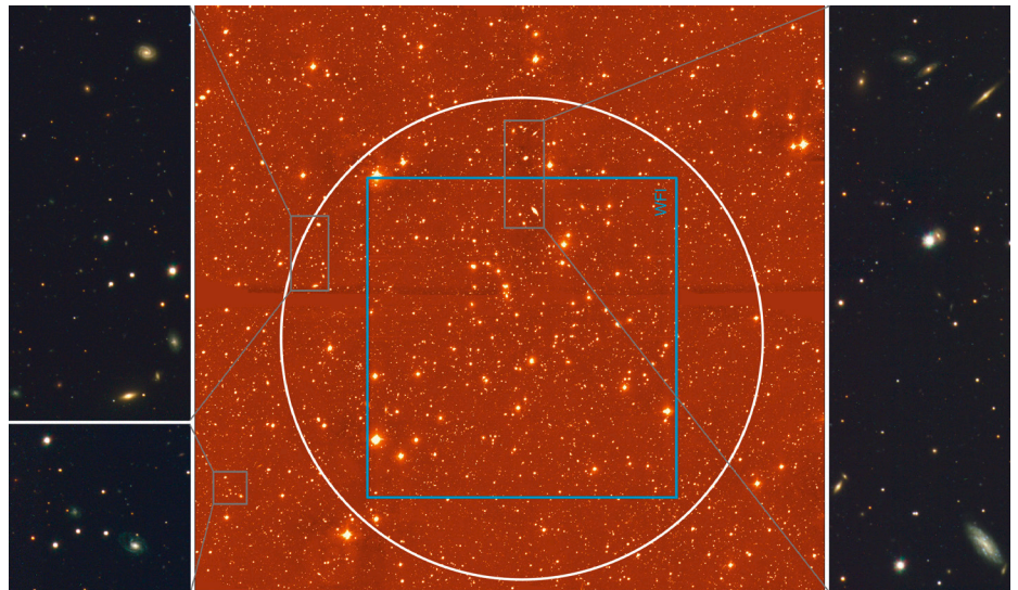
Figure 2. 1 by 1 degree V -band OmegaCAM image of cluster A2399. The FoV of WINGS imaging obtained with WFI is shown for comparison (grey square). The circle shows the radius ( R_{200} ) of the cluster. The colour images zooming into three selected areas were obtained by combining OmegaWINGS u -, B - and V -band images.
