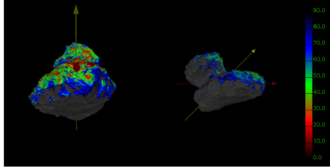
Fig. 3. Sun incidence angle (red: 0°, blue: 90°) at the time of outburst on 12 March 2015 07:13:08. Left side: projection approximately corresponding to the image geometry, Sun upwards. The whole foot of the big lobe of the nucleus is in shadow (incidence angle > 90°) including the possible jet source regions. Right side: side view, red arrow indicates direction to the observer, yellow arrow direction to the Sun.
