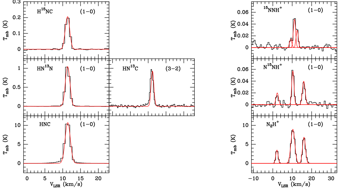
Figure 10. HNC, \text{N}_2\text{H}^+ and their isotopologues observed spectra. Gaussian fits to the lines are superimposed to the spectra. The temperature scale is main beam temperature.
