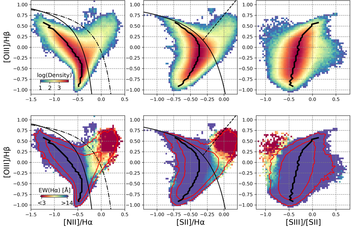
Figure 2. BPT diagrams for the single spaxels in MaNGA, plotting [\text{O III}]\lambda 5007/\text{H}\beta versus either [\text{N II}]\lambda 6584/\text{H}\alpha ([N II]-BPT, left), [\text{S II}]\lambda 6717,31/\text{H}\alpha ([S II]-BPT, center), or [\text{S III}]\lambda 9069,9531/[\text{S II}]\lambda 6717,31 ([S III]-BPT, right). The upper panels show the density of points, while the lower panels show the median \text{EW}(\text{H}\alpha) in each bin from 3\text{ \AA} (red points) to 14\text{ \AA} (blue points). The separation lines are from Kauffmann et al. (2003) and Kewley et al. (2001). The thick, black line shows the median line ratios for the star-forming galaxies in bins of [\text{O III}]\lambda 5007/\text{H}\beta . Spaxels are selected from all MaNGA galaxies included in DR15 Aguado et al. (2019) and with \text{S/N} > 5 on the required emission lines in each diagram. Fluxes are obtained from the publicly-available maps generated by the MaNGA data analysis pipeline (Belfiore et al. 2019; Westfall et al. 2019). AGN hosts, defined as MaNGA galaxies where the spectrum extracted from a 3 arcsec aperture around the galaxy centre falls in the AGN corner of the [S II]-BPT diagram according to the demarcation lines of Kewley et al. (2006), are removed.
