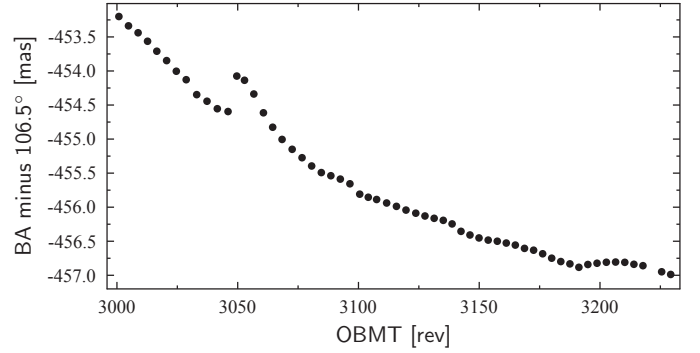
Fig. 23. Long-term trend of the ODAS-derived basic angle (BA) over two months of mission time. The ODAS determines the mean angular location of each CCD in each field of view with micro-arcsecond precision every day (the basic-angle oscillations shown in e.g. Fig. 19 are averaged out in the process), from which an absolute basic angle can be derived (the BAM performs only relative angular measurements). The plot reveals a harmless general gradient of the order of 1–2 mas per month, which corresponds to a relative movement of the edges of the main mirrors of the two telescopes by just a few nanometers per month. This trend is presumably due to seasonal temperature variations (caused by the eccentricity of the Earth orbit; the levelling-off of the curve at right coincides with the approach to the perihelion) and to ageing of materials in the space environment. The obvious jump and subsequent relaxation is caused by a thermal disturbance due to an unplanned 17-h switch-off of the onboard payload data handling unit on November 29, 2015. Some of the smaller wiggles in the curve can also be traced to variable onboard conditions, such as e.g. a varying star density on the sky scanned by Gaia .
