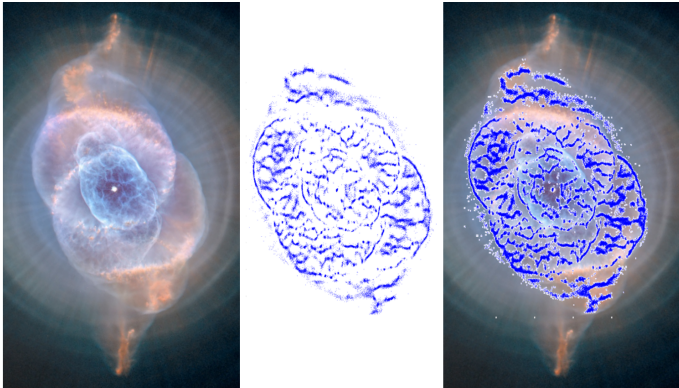
Fig. 14. Cat's Eye planetary nebula (NGC 6543) observed with the Hubble Space Telescope (left image) and as Gaia detections (the 84 000 blue points in middle and right images). (Credit: photo: NASA/ESA/HEIC/The Hubble Heritage Team/STScI/AURA.)
