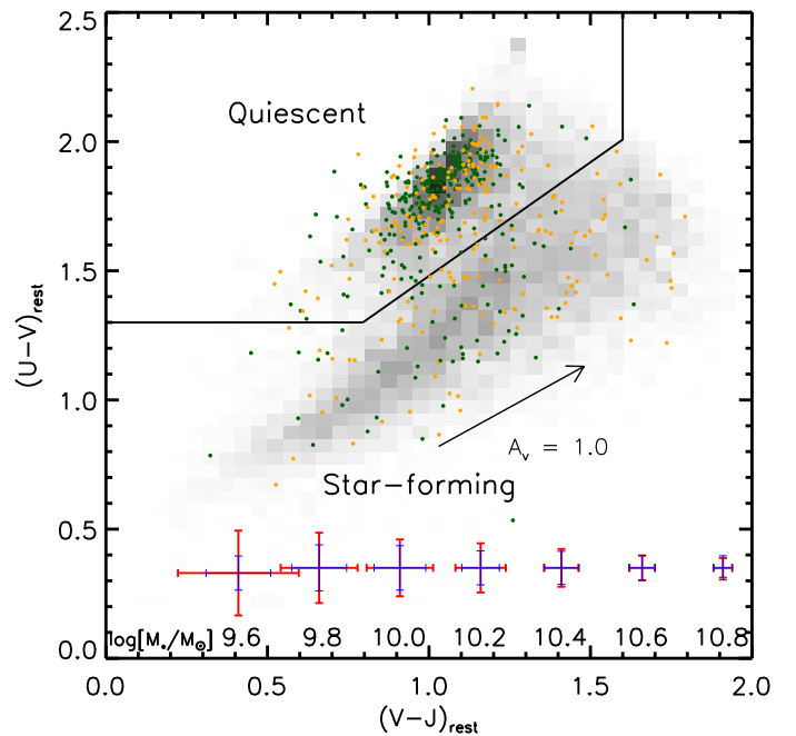
Fig. 2. Rest-frame U - V vs. V - J diagram for galaxies compiled from all clusters, with stellar masses M_\star \geq 10^{10} M_\odot and within projected R \leq 1000 kpc. Green: spectroscopic cluster members with |\Delta z_{\text{spec}}| \leq 0.02 . Orange: photometric cluster members with |\Delta z_{\text{phot}}| \leq 0.08 . Grey distribution: UltraVISTA field galaxies with redshifts 1.0 < z < 1.4 in the same mass range. The error bars present typical uncertainties at the depth of our photometry for different stellar masses, and separately for quiescent (red) and star-forming (blue) galaxies.
