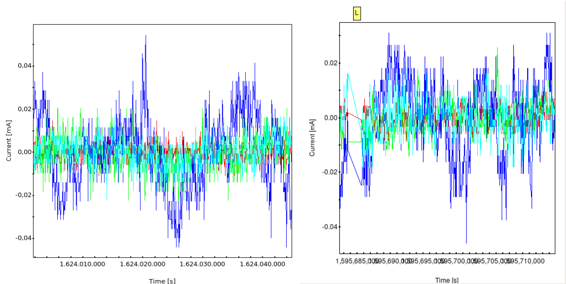
Figure 4 – Feed 18 FEM Id S2 (red), Id S1 (green), Id M1 (blue), and Id M2 (cyan). Left panel: CPV stability check. Right panel CSL test XXX_0203
