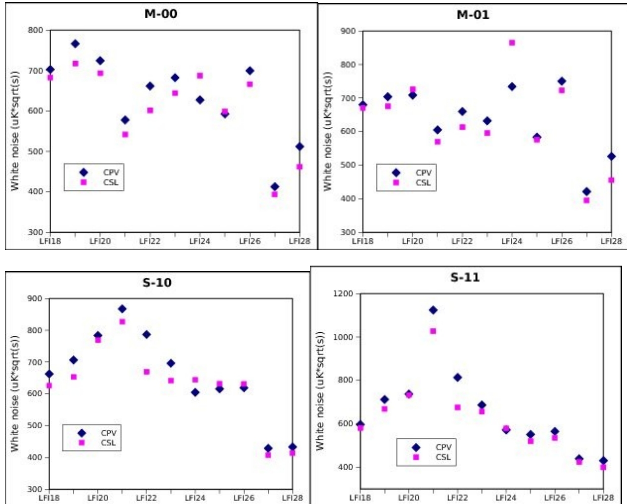
Fig 11 – Comparison of calibrated white noise between CPV and CSL with the instrument set at CSL optimal biases and reference load at \sim 20 K
