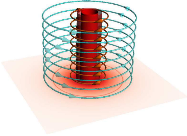
Figure 1. Contour rendering of the density showing the plasma column at t = 0 for the PB equilibrium. A slice of the density (pseudocolour rendering) on the xy plane ( z = -1 ) is superimposed, showing the maximum of \rho at r_1 (see text). The red and blue circles show magnetic field lines of opposite polarity for B_\phi .
