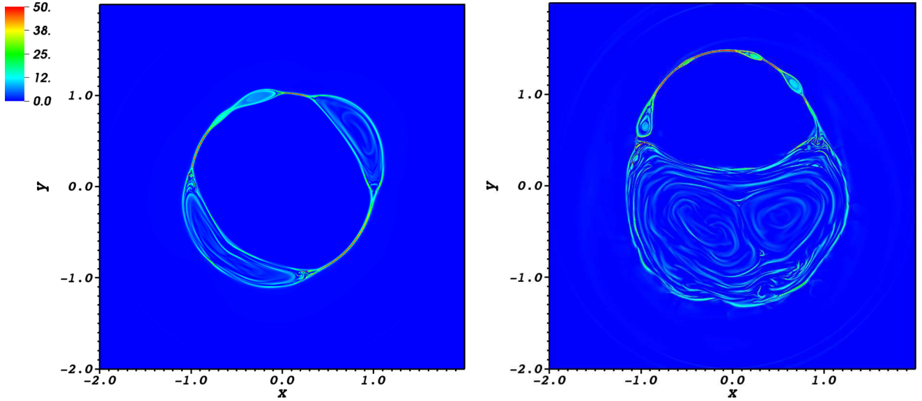
Figure 4. Pseudocolour rendering of the current density J_z for case 2D with S = 1.0 \times 10^5 at t \approx 2.5 t_A (left) and t \approx 4.8 t_A (right). We note the formation of multiple plasmoids and small-sized current sheets due to secondary tearing instability, in a manner similar to the ‘plasmoid turbulence’ described in Loureiro et al. (2012).
