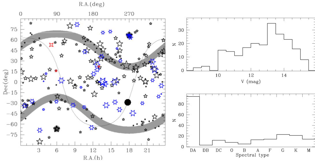
Figure 3: Gaia external calibration sources (SPSS) distribution of their positions on the sky (left), magnitude (right top panel) and spectral type (right bottom panel), extracted from [3]. In the left panel, the Galactic plane and center are marked with a dotted line and a black circle, respectively. The Ecliptic poles are marked as two grey circles, and two shaded stripes corresponding to the ecliptic latitude \pm 45^\circ where Gaia is observing more often.
