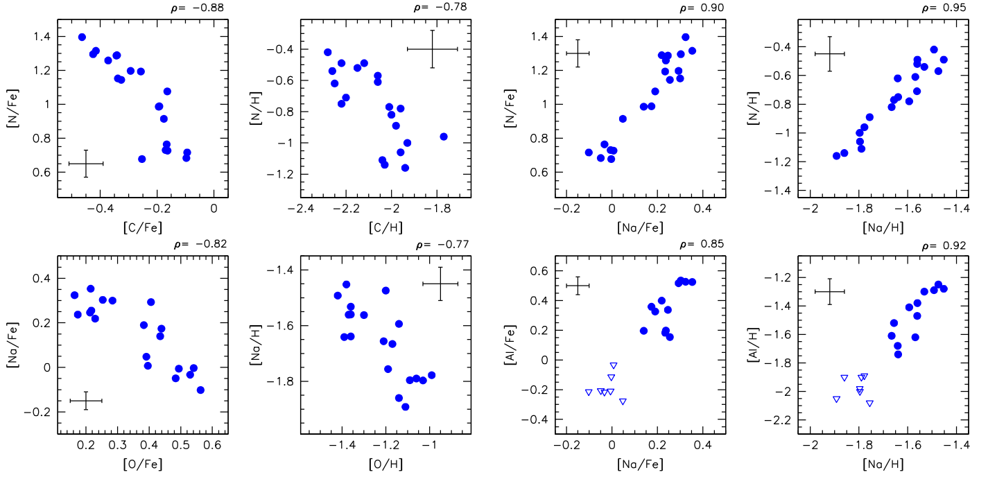
Figure 2. Light element abundances measured for the investigated AGB stars. All abundance ratios are shown normalized both to iron and to hydrogen. The typical error bars of the measured abundances and the the Spearman rank coefficients of every correlation are marked in each panel. In the bottom right panels the empty triangles mark the stars for which only upper limits to [Al/Fe] have been derived.
