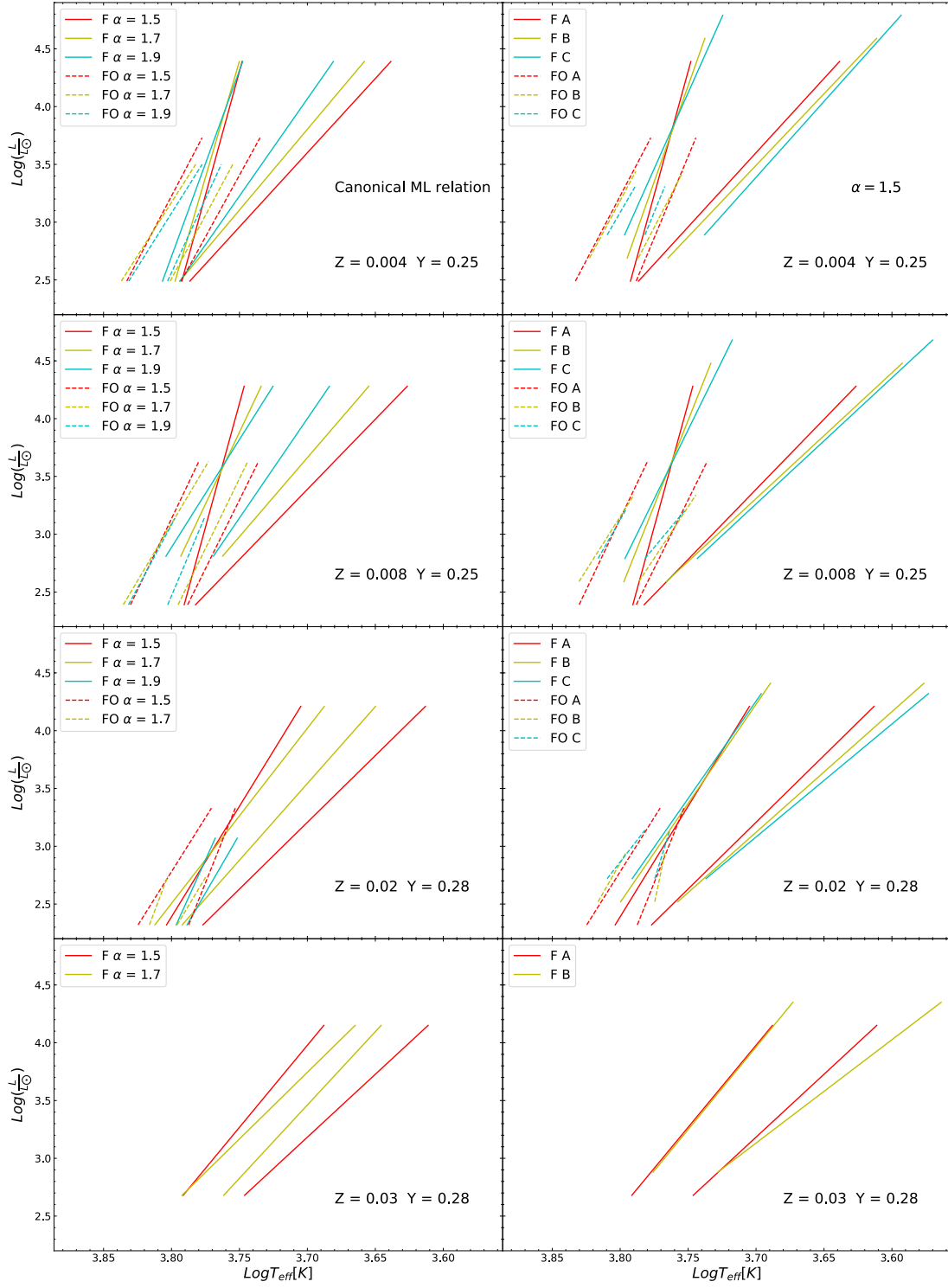
Figure 8. The F and FO instability strips for Z = 0.004 \ Y = 0.25 , Z = 0.008 \ Y = 0.25 , Z = 0.02 \ Y = 0.28 and Z = 0.03 \ Y = 0.28 pulsators at a fixed case A ML relation for the various assumptions about the superadiabatic convective efficiency (left panels) and at a fixed mixing length parameter \alpha_{ml} = 1.5 for the assumed A, B, C ML relations (right panels).
