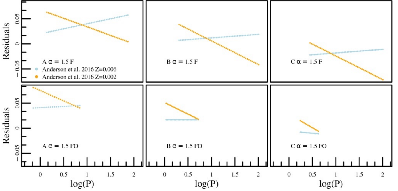
Figure 6. As in Fig 5, but subtracting the PR relations for Z=0.006 and Z=0.002 provided by Anderson et al. (2016) , from the one obtained in this work for Z=0.004 and \alpha_{ml} = 1.5 , as a function of the pulsational period. The top and bottom panels show the results for the F and FO-mode pulsators, respectively. The left panels contain the results for the canonical case A while the central and right panels contain the results for the noncanonical cases B and C, respectively. In each panel, the residuals for Z=0.006 and Z = 0.002 are plotted using light blue and orange dots, respectively.
