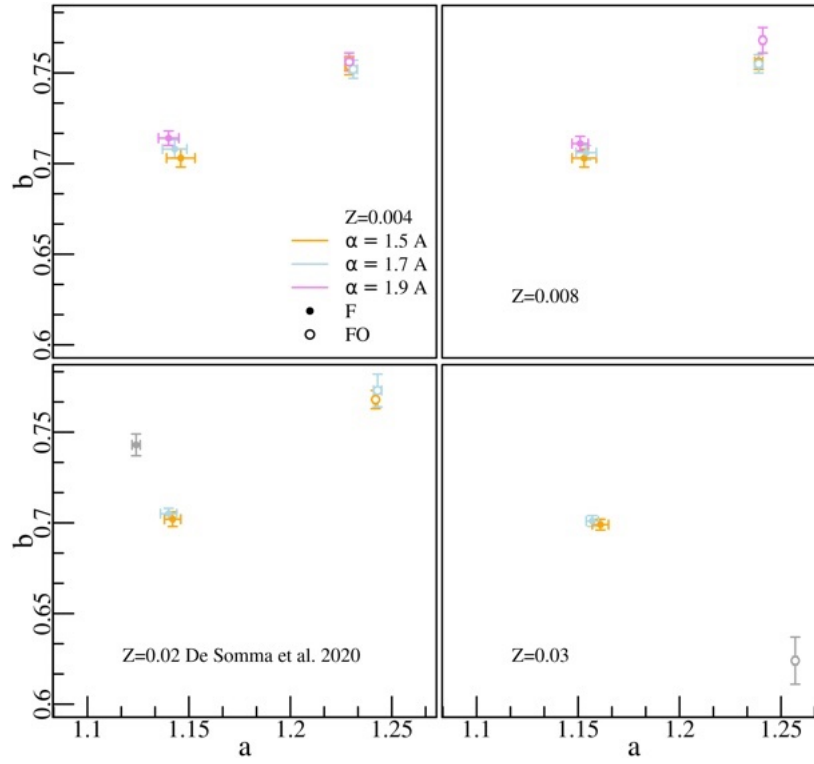
Figure 2. The intercept ( a ) and the slope ( b ) of the fitted canonical F and FO mode PR relations for Z = 0.004 Y = 0.25 , Z = 0.008 Y = 0.25 , Z = 0.02 Y = 0.28 (taken from De Somma et al. (2020b)) and Z = 0.03 Y = 0.28 as a function of the mixing length parameter (see text and labels for more details).
