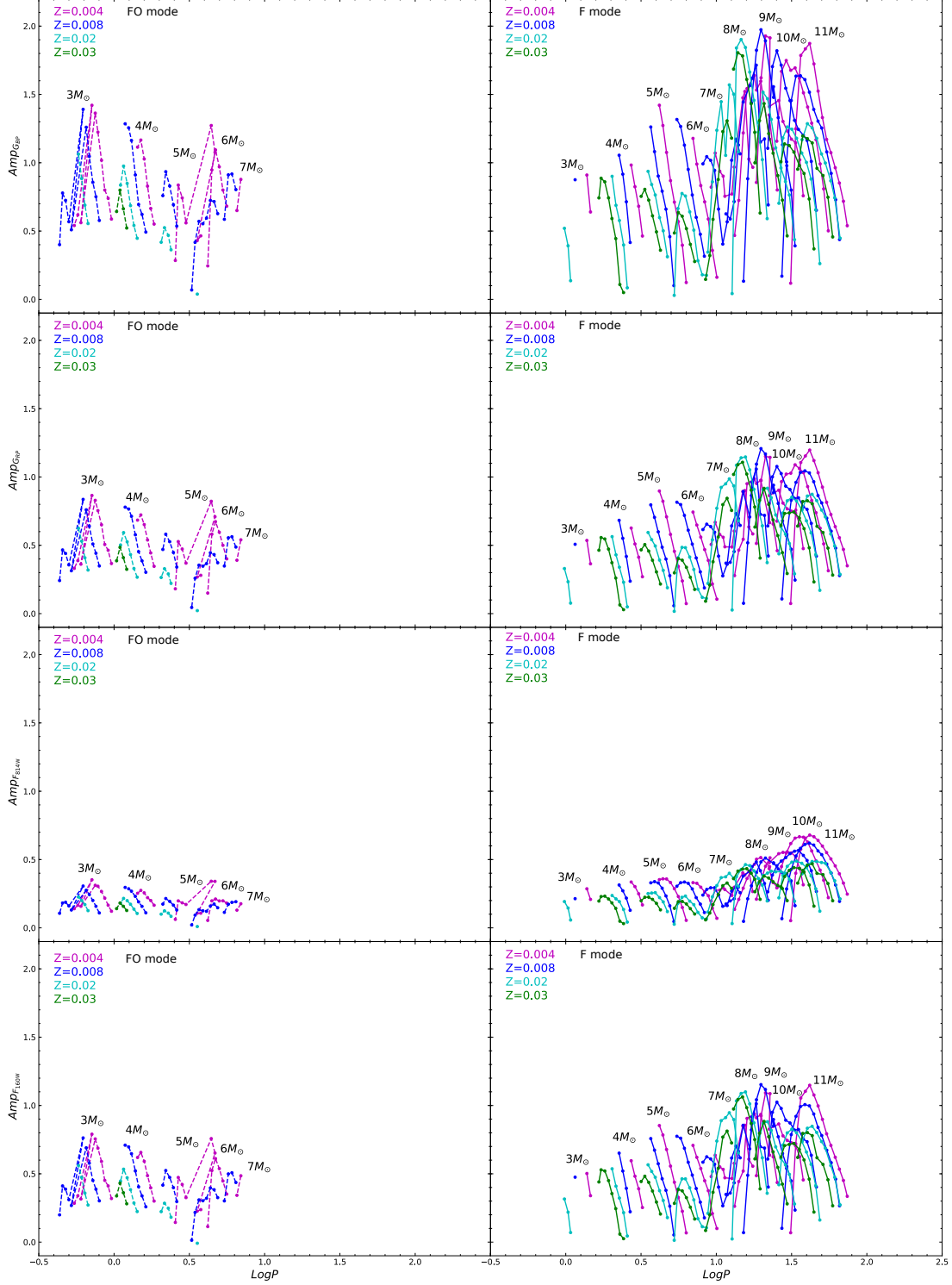
Figure 14. From top to bottom, the left panels show the FO-mode theoretical amplitudes for the G_{BP} and G_{RP} Gaia bands and the F814W and F160W HST-WFC3 bands for Z = 0.004 Y = 0.25 (dashed magenta line), Z = 0.008 Y = 0.25 (dashed blue line), Z = 0.02 Y = 0.28 (dashed cyan line) and Z = 0.03 Y = 0.28 (dashed green line) at fixed mixing length parameter \alpha_{ml} = 1.5 and ML relation case A. The right panels show the same plots but for F-mode models (solid lines with the same color-code as in the left panels).
