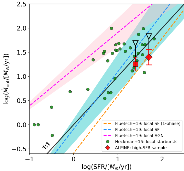
Fig. 10. Comparison of our results with a compilation of data at low z in the \log(M_{\text{out}}) – \log(\text{SFR}) diagram. The red square (diamond) indicates the average outflow rate for the atomic component obtained from the stacking of the full (high-SFR) sample, while red bars indicate the associated uncertainty ( \pm 1\sigma ). The black arrows show our estimate of the total \dot{M}_{\text{out}} (calculated adopting a correction for multi-phase outflows; see text). The orange (cyan) dashed line indicates the best fits for single-phase (three-phases, i.e., molecular, ionised, and atomic) \dot{M}_{\text{out}} observations in local star-forming galaxies, while the magenta dashed line represents the best fit from observation of local AGNs (from Fluetsch et al. 2019). Filled colored regions indicate the 2\sigma dispersion around the best fits. The green points show the distribution of a sample of local starbursts (Heckman et al. 2015). The blue solid line indicates the 1:1 relation ( \eta = 1 ).
