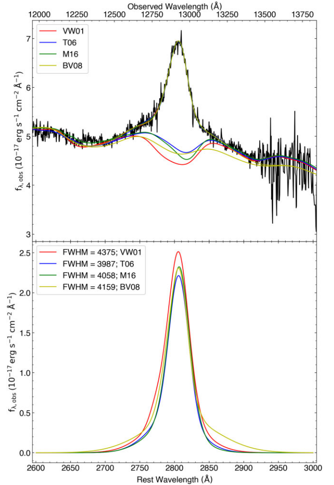
Figure 1. Example model of the Mg II emission feature of J110352+100403 with the combined pseudo-continuum from the power-law, Balmer, and Fe II components. The line models differ from one another by the applied Fe II template as indicated in the legend. The resulting continuum for each template is plotted in solid lines in the top panel and the continuum-subtracted line profile model is plotted in the bottom panel. In this example, the Mg II FWHM between models with different Fe II templates ranges from 4000 to 4400 km s −1 .
