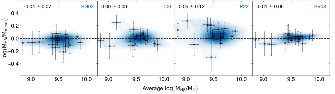
Figure B4. Black hole mass comparison, \log(M_{\text{H}\beta}/M_{\text{mean}}) , between different Fe II templates models for H \beta compared to the average H \beta -based mass estimate. The top-left value displays the mean residual and its standard deviation between mass measurements. The Fe II template is identified in the top-right corner of each panel. The blue shaded contours represent the two-dimensional continuous probability density distribution calculated with a kernel density estimator (Waskom 2021). Each subsequent contour level marks density iso-proportions increasing by an additional 10 per cent up to 90 per cent enclosed.
