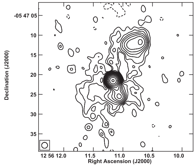
Figure B1. The 1665 MHz image of 3C 279. The radio contours are in percentage of peak surface brightness ( =10.2 Jy beam ^{-1} ) and increase in steps of 2, with the lowest contour being \pm 0.02\% . The jet points toward the south. Note the luminous radio lobe to the north and the diffuse halo type emission.
