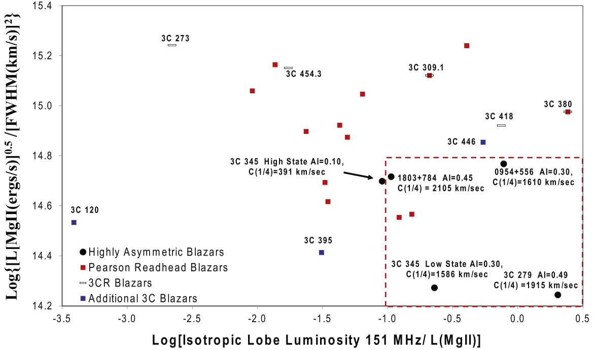
Figure 6. The scatter plot is empirical in nature. The RA blazars 3C 279, 0954+556, and 1803+784 are compared with the with two complete samples, the extreme blazars in the high-frequency-selected Pearson–Readhead sample and the low-frequency-selected 3CR sample. The horizontal axis is the large-scale isotropic low-frequency luminosity, \nu_e L_\nu(\nu_e = 151\text{MHz}) , normalized to the Mg II BEL luminosity. The vertical axis is [L(\text{MgII})]^{0.5}/\text{FWHM}^2 , which is indicative of the Eddington ratio based entirely on the Mg II line.
