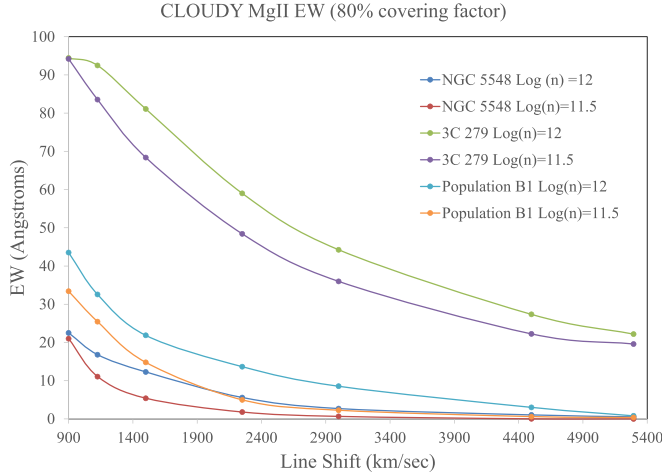
Figure 15. Comparison of the Mg II VBC rest frame EW as a function of line (red) shift computed from the 3C 279 SED, the Population B1 SED, and the low-state NGC 5548 SED in Figure 12. The figure shows that the 3C 279 SED in Figure 12 efficiently excites a dense BEL gas at large redshift, yet both the Population B1 SED and the low-state NGC 5548 SED seem to overionize the VBC region for efficient Mg II line emission to a similar degree. The NGC 5548 contrast with 3C 279, along with the input SEDs in Figure 12, shows that the steep EUV continuum associated with a powerful jet makes a profound difference on the VBC strength.
