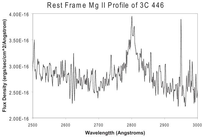
Figure 7. Symmetric Mg II BEL in the blazar 3C 446. Even though \nu_e L_\nu(\nu_e = 151\text{MHz})/LMgII is large for the isotropic lobe emission, there is no dramatic redward asymmetry in Mg II.
