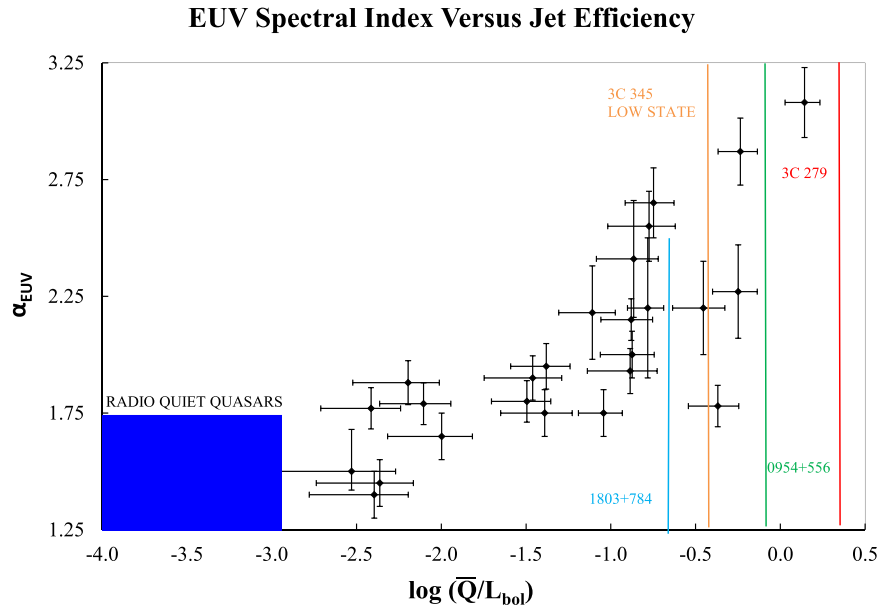
Figure 10. This scatter plot shows that the EUV deficit of RLQs is originally from Punsly & Kharb (2016). We superimpose the locations of the x -variable ( \bar{Q}/L_{\text{bol}} ) for the RA blazars for comparison purposes. The \bar{Q}/L_{\text{bol}} estimates for the RA blazars are from Tables 3 and 4.
