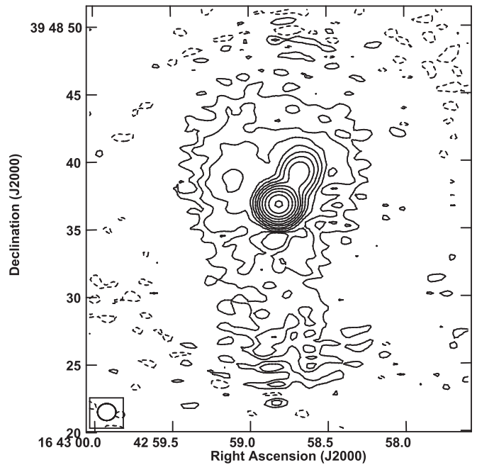
Figure B2. The 1552 MHz image of 3C 345. The radio contours are in percentage of peak surface brightness ( =7.7 Jy beam -1 ) and increase in steps of 2, with the lowest contour being \pm 0.042\% . Note the diffuse halo type emission that surrounds the core-jet structure.
