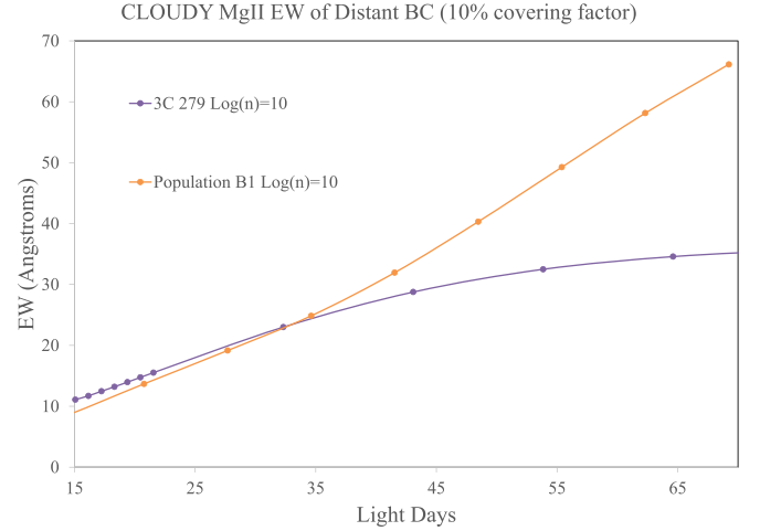
Figure 16. Comparison of the Mg II BC EW as a function of the number of light-days from the quasar computed from the 3C 279 SED and the Population B1 SED in Figure 12. From Equation (25), we estimate that the Mg II BC is \sim 70 lt-days from the quasar in 3C 279. The Population B1 SED induces much more efficient Mg II emission than the 3C 279 SED \sim 70 lt-days from the quasar. Apparently, the weak ionizing continuum of 3C 279 can underionize the distant BC gas for efficient Mg II emission.
