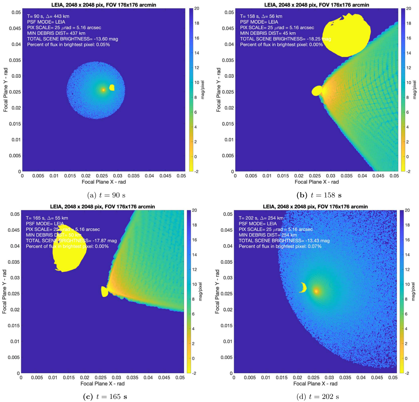
Figure 5. Simulated LEIA images for the nominal case, with LEIA PSF applied, at t = 90, 158, 165 , and 202 s ( t = 0 at the time of impact). Note that the color scale indicates magnitude per pixel (magnitude herein means the usual astronomical magnitude as a measure of brightness) and remains fixed at [-2, 20] for all frames. The distances from the camera to Dimorphos ( \Delta ) are about 443, 56, 55, and 254 km. The minimum distances from LICIACube to any ejecta are about 437, 45, 50, and 254 km.
