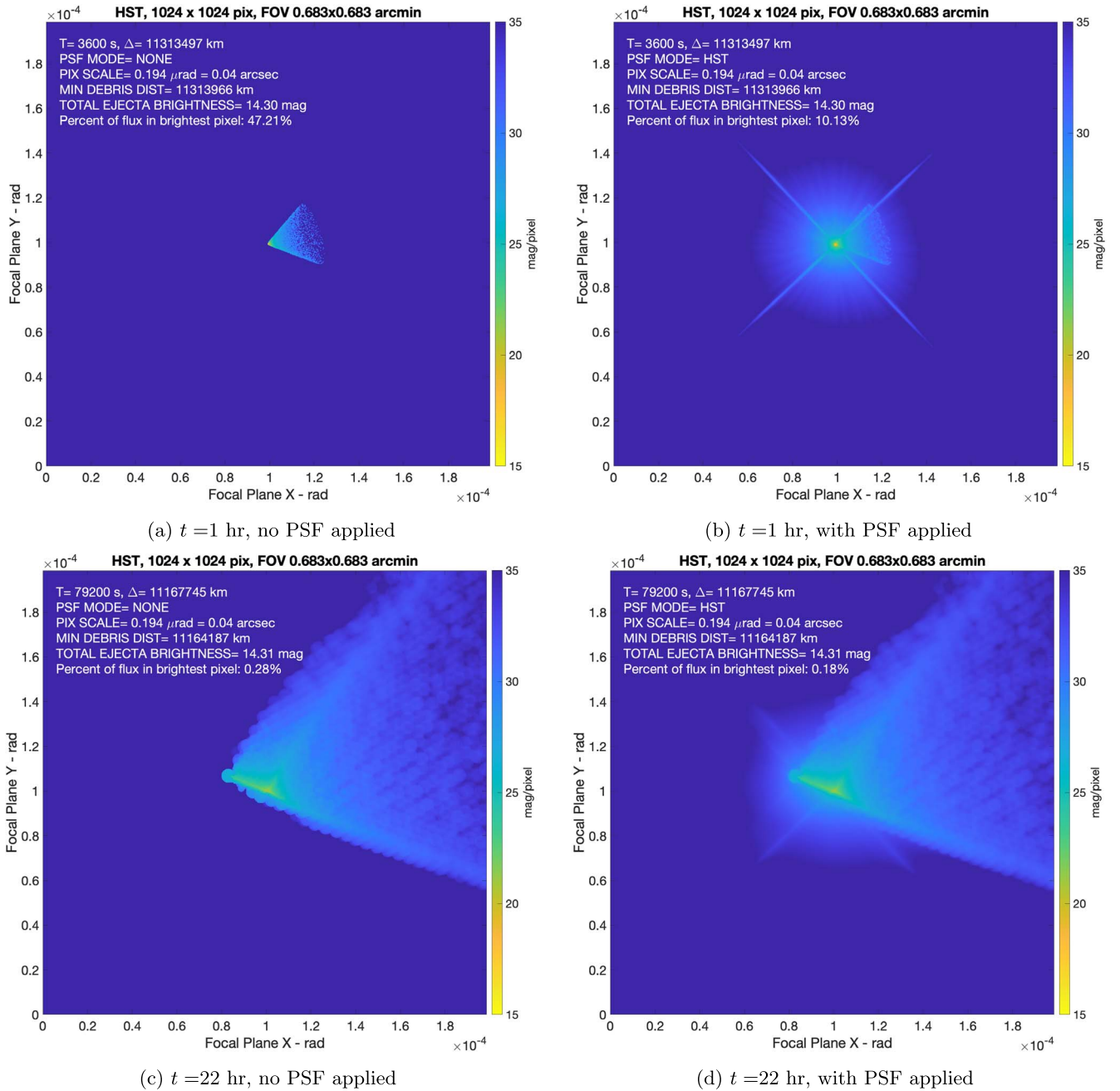
Figure 6. Simulated HST/WFC3-UVIS images for the nominal case, without (left) and with (right) the appropriate camera PSF applied, at t = 1 (top) and 22 (bottom) hr. Again, t = 0 at the time of impact. Note that the color scale indicates magnitude per pixel and remains fixed at [15, 35] for all frames. The total ejecta brightness integrated over the whole FOV remains nearly constant at 14.30–14.31 mag, but the percent of that brightness concentrated in the brightest pixel declines precipitously from 47.21% in panel (a) to 0.28% in panel (c) with no PSF applied and from 10.13% in panel (b) to 0.18% in panel (d) with PSF applied. See text for discussion of apparent structure.
