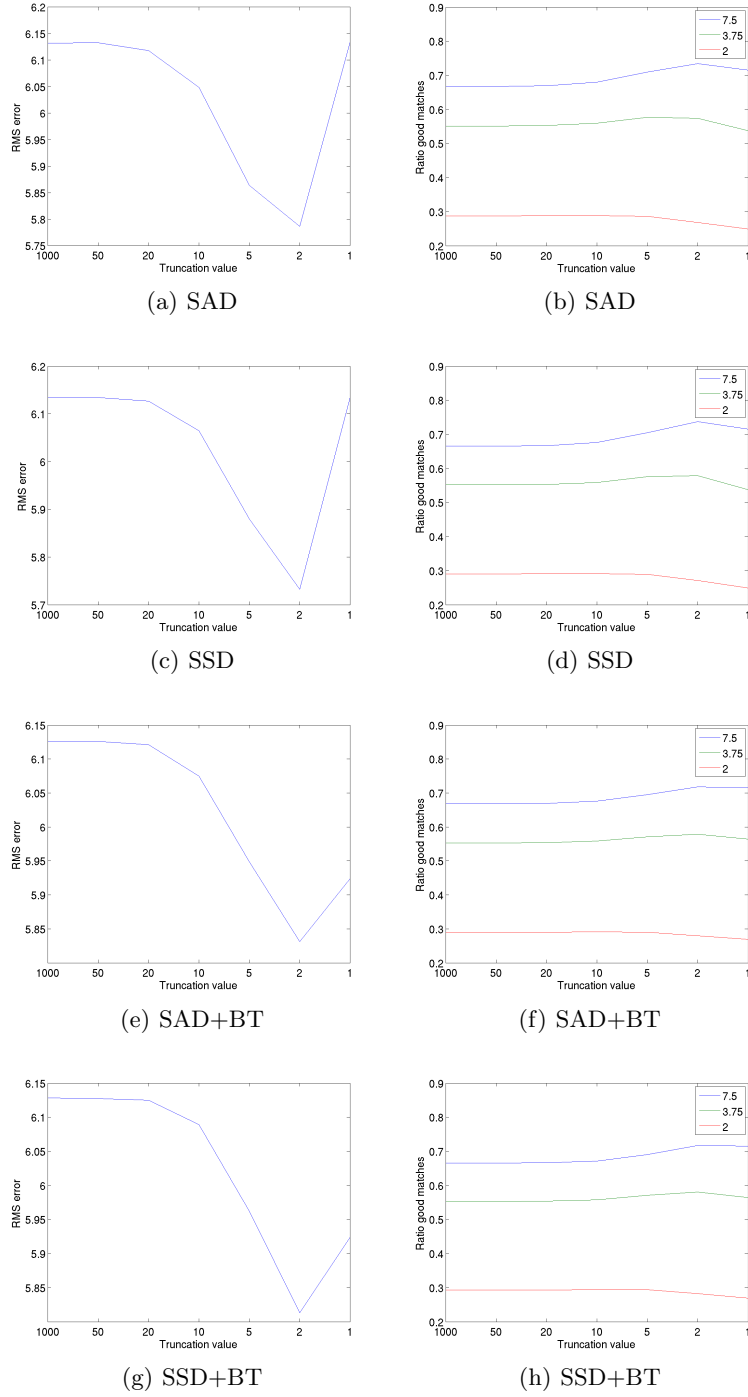
Figure 4. Experiment 1. Performance of different cost functions with a 9 \times 9 aggregation window. The two error measures are plotted against different truncation values. The left column shows the graphs relative to the RMS, while the G error is displayed on the right column.
