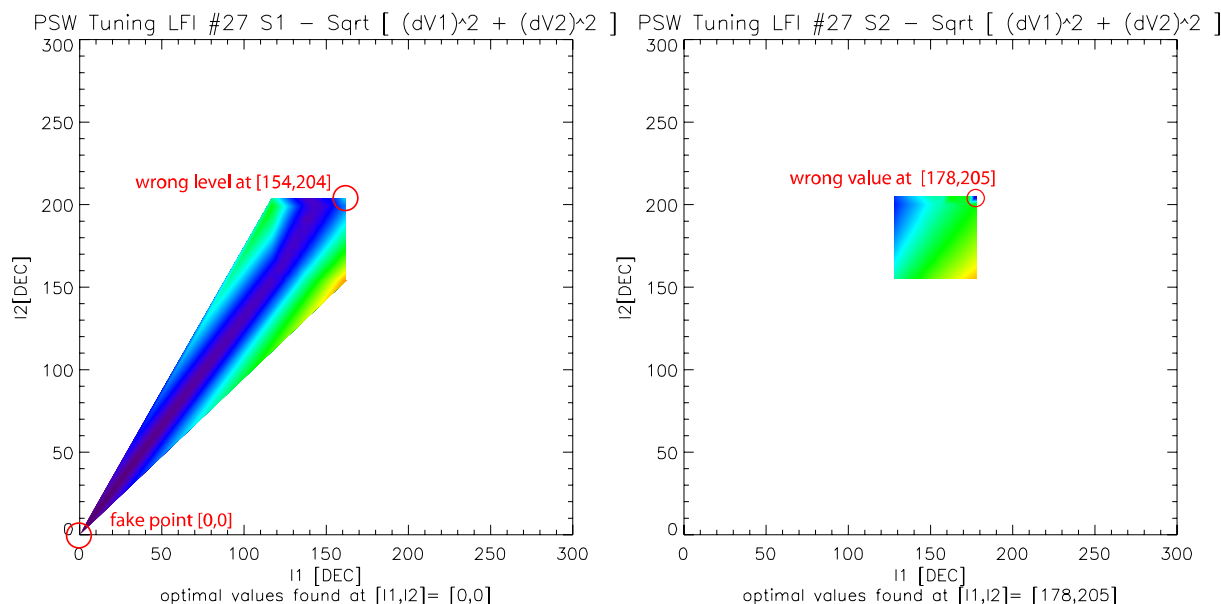
Figure 5: Typical contour plot of the phase switch tuning. Here the plot is “as it is” from the automatic routine. In some cases fake points appears (left plot) together with point with a wrong signal level (right plot)
