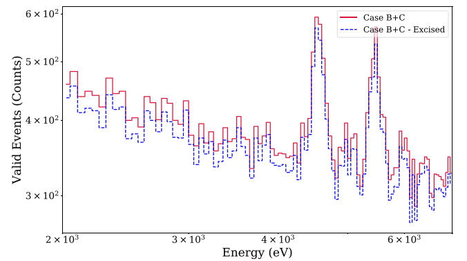
Figure 7. Pulse-height spectrum of valid events detected in Case B and C frames (in red). Rejecting valid events associated with a primary GCR by using SAC with a 30 pixels exclusion radius would reduce the particle-induced background level of the XMM-Newton EPIC-pn by \sim 10\% in the 2–7 keV energy band. The resulting background spectrum is shown in dashed blue.
