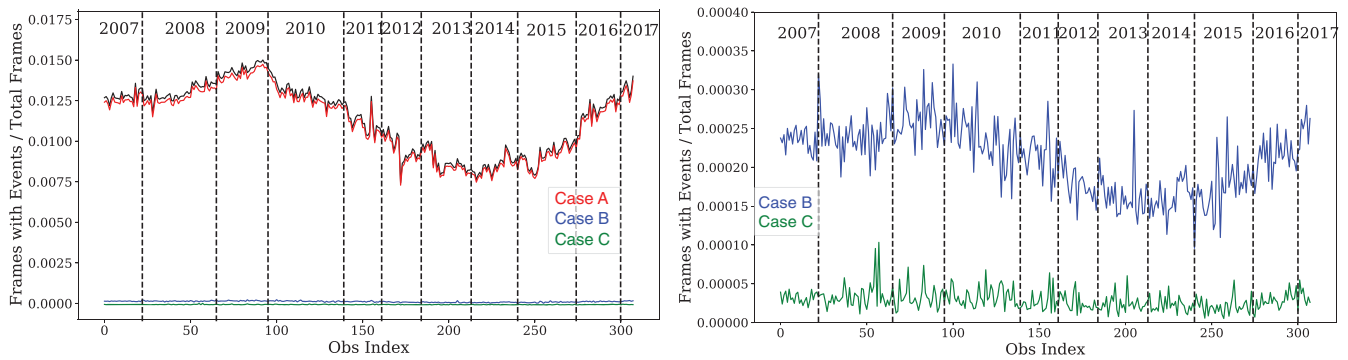
Figure 2. Left: the fraction of frames with just primary particle events (red: Case A), just secondary valid events (blue: Case B), and with both valid and particle events (green: Case C) as a function of time. Black curve shows the total rate of particle events. Strong modulation with the solar cycle observed for all the frames indicates that the XMM-Newton EPIC-pn unfocused background is dominated by Galactic cosmic rays. Right: zoom onto Case B and Case C frame to enhance the visibility of the solar modulation cycle.
