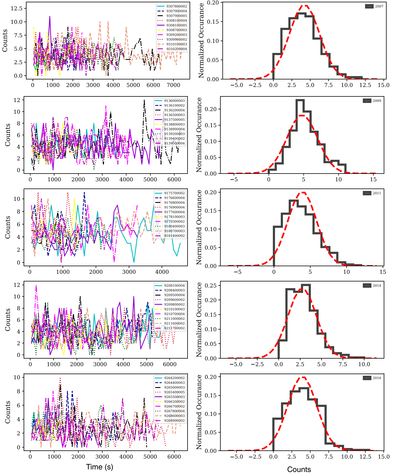
Figure 10. Light curves of valid events in 2–7 keV band detected in Case B frames per 200 s binning for five different epochs in the solar cycle are shown on the left panels. The dashed lines in the right hand panels show the expected Poisson distributions around the mean. The distributions of count rates of particle events in these observations in each epoch are shown on the right panels.
