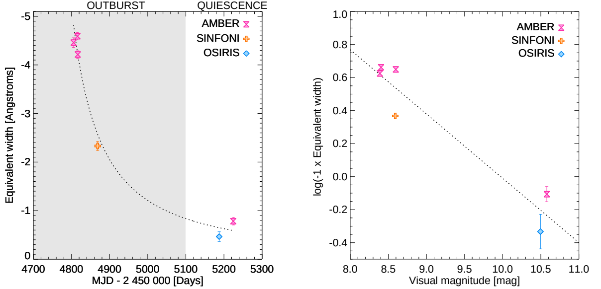
Fig. 15. Decline of the Br \gamma equivalent width with time (left) and with the system V-band magnitude (right).
