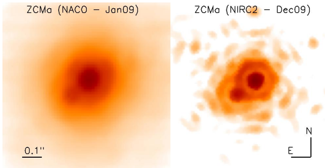
Fig. 2. Left: VLT/NACO K_s -band image of Z CMa on January 31, 2009. Right: Keck/NIRC2 K_{\text{cont}} image on December 7, 2009.
