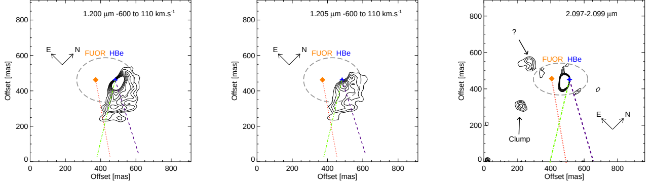
Fig. 18. Extended structures observed at 1.200, 1.205, and 2.098 \mu\text{m}
