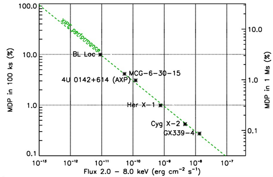
Figure 7. The Minimum Detectable polarization of XIPE taking into account a configuration of 3.5 m focal length and 27 shells.
