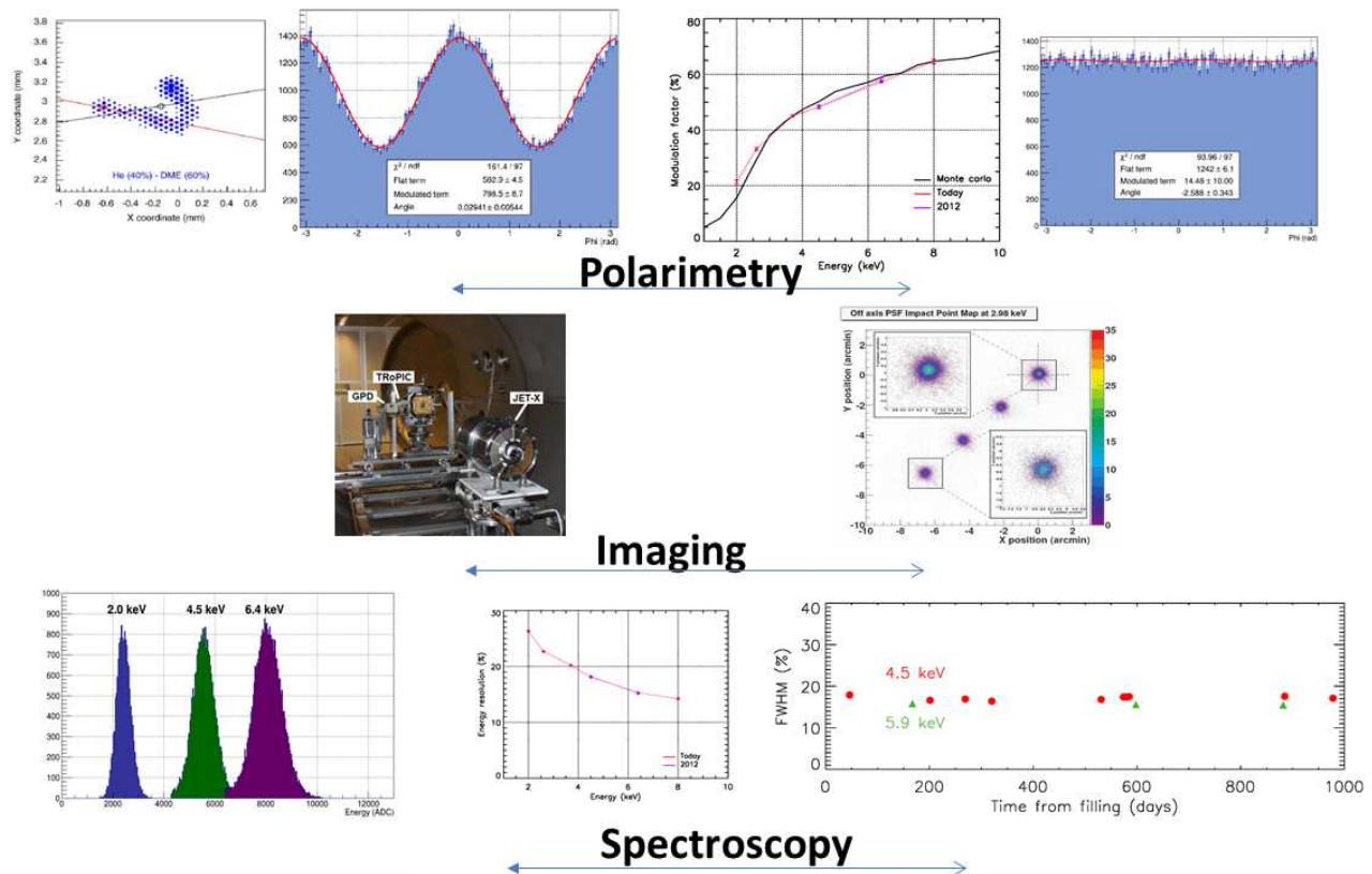
Figure 1. ( Top ) From left: an image of a photoelectron track; a modulation curve at 3.7 keV; the modulation factor as a function of energy; a modulation curve for an unpolarized ^{55}\text{Fe} source. Middle . From left: the GPD at the focus of a JET-X optics together with the CCD and the ROSAT PSPC; the on-axis and off-axis images. Bottom From left: the spectra of sources at 2.0, 4.5 and 6.4 keV; the behavior of the energy resolution with energy; the behavior of the energy resolution with time.
