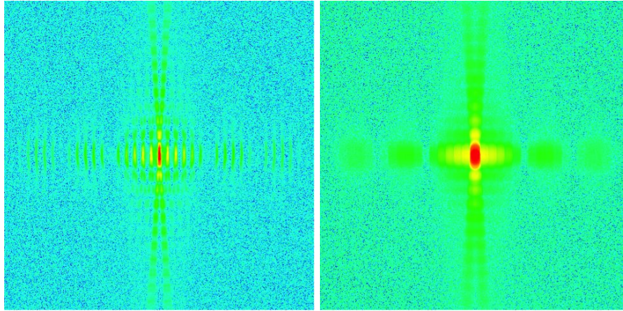
Figure 7. Best-focus configuration of two separated MMs, supposed to have perfect Wolter I surfaces. The simulated detector field is 2 mm and the pixel size is 2\ \mu\text{m} . Left: PSF of two MMs illuminated by a 0.25 arcsec source. Right: PSF of two MMs illuminated by a 1 arcsec dimension source.
