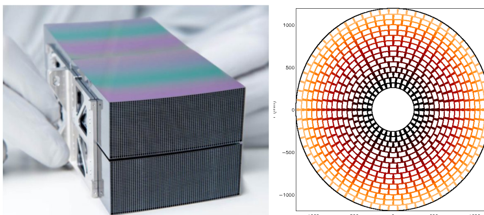
Figure 1. Left: A Wolter-I SPOs mirror module (image credits: ESA). The MM is realized as a double stack of 34 plates assembled in Wolter-I configuration. Right: Graphic representation of the MMs positions in the ATHENA telescope. The MMs are organized in 15 rows with hexagonal symmetry.
