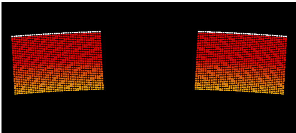
Figure 6. CPF model used to simulate the co-focality of two separated MMs. Two MMs are considered separated by a dark area, the variable shade of red represents the optical path distance variation through the layers.
