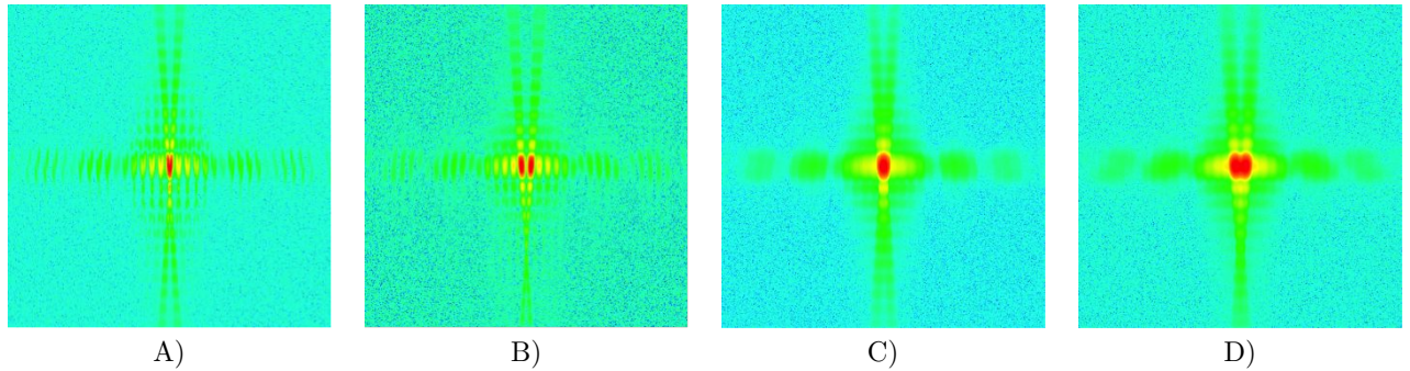
Figure 8. The same configuration shown in Figure 7: moving a 2 mm wide detector intra-focal by A) 3 mm and B) 1 cm, considering a source 0.25 arcsec wide. Moving a 2 mm wide detector intra-focal by C) 3 mm and D) 1 cm, considering a source 1 arcsec wide.
