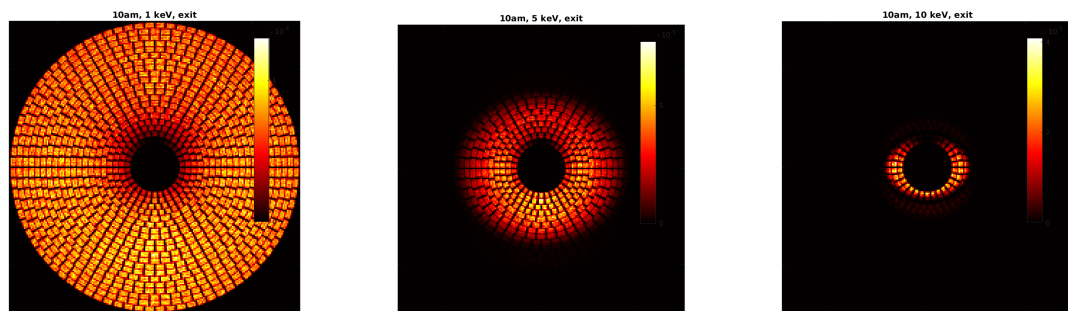
Figure 5. ATHENA optics through McXtrace ray-tracing. Example of simulated photons at exit of the optics for 10 arcmin off-axis exposure with energies of 1 keV (left), 5 keV (center) and 10 keV (right).
