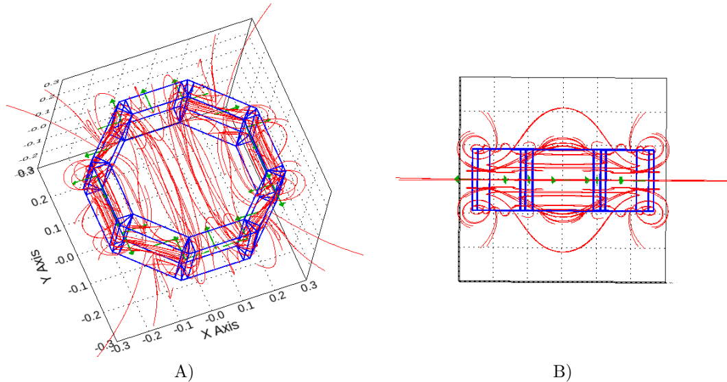
Figure 9. Some simulated magnetic induction field lines, in the updated design of the Halbach array. A) Tilted view. B) Viewed sideways.
