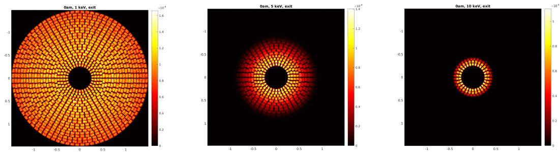
Figure 4. ATHENA optics through McXtrace ray-tracing. Example of simulated photons at exit of the optics for on-axis exposure with energies of 1 keV (left), 5 keV (center) and 10 keV (right).
