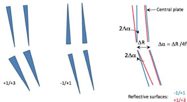
Figure 2. Different plate stacking in an SPO module, in radial section. Left: the +1/+3 wedge configuration requires manufacturing two different kinds of wedged plates. Center: the -1/+1 wedge configuration is obtained producing Silicon plates with the same wedge angle. Right: with respect to the +1/+3 wedge, the angle variation in the -1/+1 wedge configuration introduces an apparent source divergence \delta n = 2n\Delta\alpha for the n -th plate, counted from the central one.
