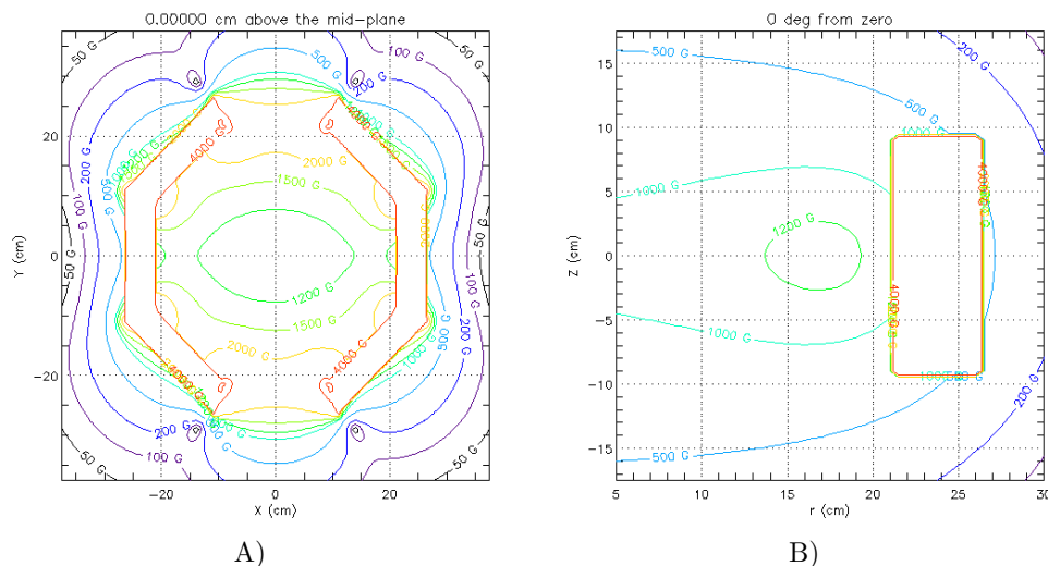
Figure 10. Isocontours of the magnetic induction intensity. A) Median section of the array. B) Radial section. We easily see that the field is above 500 G within all the internal volume of the Halbach array.
