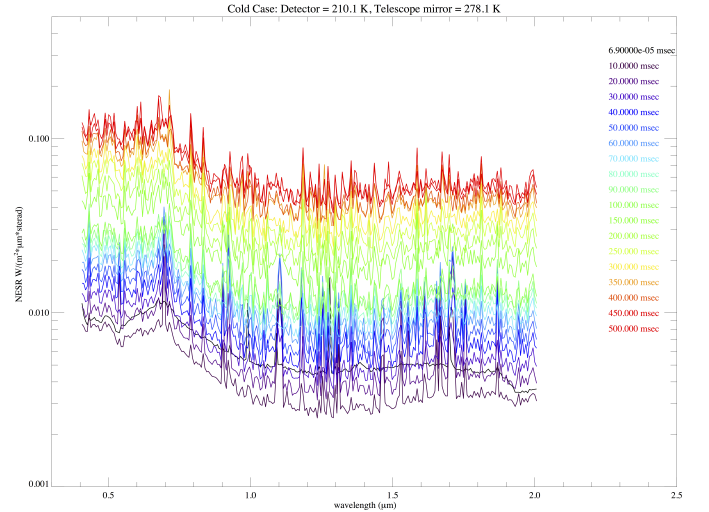
Fig. 2. VIHI NESR profiles for integration time between readout and 500 msec at detector's low temperature T_l=210 K.
