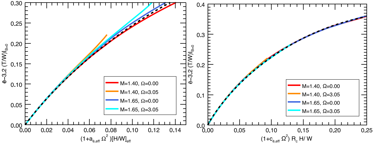
Figure 15. Deformation \bar{e} with respect to the unmagnetized model as a function of the effective mass energy ratio H/W in the left-hand panel or HR_c/W (where R_c is normalized to 14 km) in the right-hand panel for configurations with mass between 1.40 and 1.65 M_\odot and rotational frequency \Omega = 0.0\text{--}3.05 \times 10^3 \text{ s}^{-1} . The dashed black lines show equation (78) (left-hand panel) and equation (81) (right-hand panel).
