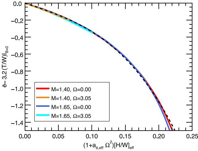
Figure 8. Deformation ratio \bar{e} with respect to the unmagnetized model in terms of the effective magnetic energy ratio [H/W]_{\text{eff}} for configurations having gravitational mass 1.40\text{--}1.65 M_\odot and rotational frequency \Omega = 0.0\text{--}3.05 \times 10^3 \text{ s}^{-1} . The black dashed line represents equation (66).
