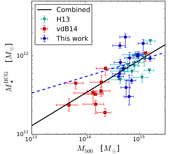
Figure 2. The BCG stellar mass ( M_{\star}^{\text{BCG}} ) versus cluster virial mass M_{500} for the SPT sample (blue), H13 (cyan) and vdB14 (red). The H13 sample is corrected to Chabrier IMF. The blue dashed line is the best fit for the SPT sample alone and the black solid line is the best fit for the combined sample (see equation 4).
