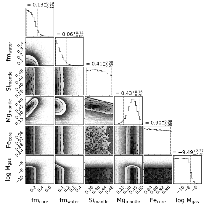
Fig. 3: Corner plot showing the posteriors of the main parameters of our internal structure analysis for TOI-732 b. The titles of each column correspond to the median of the distribution, with the 5 th and 95 th percentiles as the uncertainty values. From left to right, the depicted internal structure parameters are the mass fractions of the inner iron core and of the water layer (both calculated with respect to the condensed part of the planet without the H-He layer), the molar fractions of Si and Mg in the mantle, the molar fraction of Fe in the inner core, and the total mass of H-He in Earth masses on a logarithmic scale. The mass fractions of the inner core and the water layer add up to one, with the mass fraction of the mantle layer (not shown) by construction.
