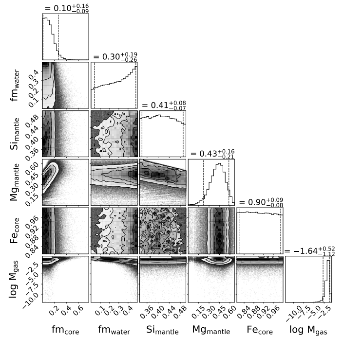
Fig. 4: Same as Figure 3, but for TOI-732 c.
