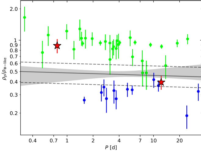
Fig. 9: Normalised density as a function of orbital period. The normalised density is the mean density of the planet divided by the density the planet would have if it had an Earth-like composition (same variable as introduced in L22 to display the density valley). The grey line and its shaded area indicate the density valley with its corresponding error, as in Fig. 6.
