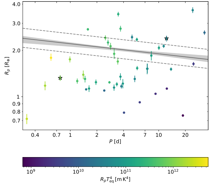
Fig. C.1: Same as Fig. 6, but with the markers colour-coded against R_p T_{eq}^4 , which correlates with the core-powered mass loss strength (Gupta & Schlichting 2019).
