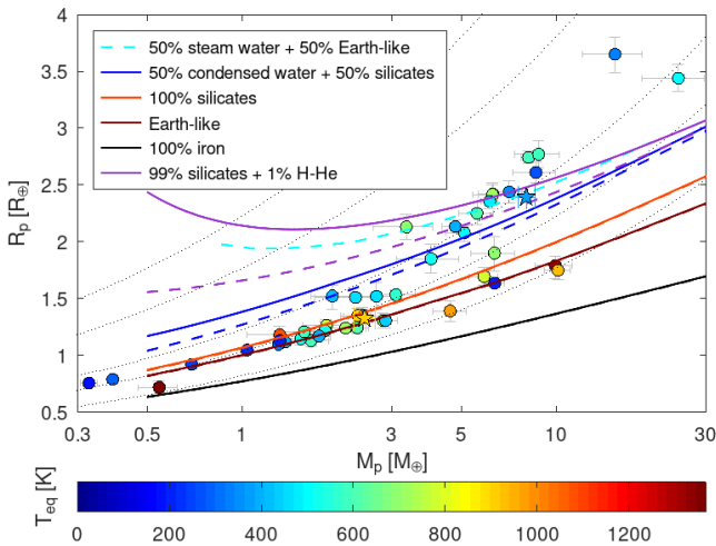
Fig. 5: Mass-radius diagram of M-dwarf planets with R_p < 4 R_\oplus and M_p < 30 M_\oplus whose R_p and M_p precision is better than 8% and 25%, respectively. All planets are colour-coded with respect to their equilibrium temperature ( T_{\text{eq}} ) and in particular, TOI-732 b and TOI-732 c are marked by a star. Following the colour scheme given in the legend, two different sets of planet composition models generated with BICEPS (Haldemann et al. 2023) are displayed. The solid and dashed lines are obtained for T_{\text{eq}} = T_{\text{eq},b} = 900 K and T_{\text{eq}} = T_{\text{eq},c} = 360 K, respectively. The 50% steam + 50% Earth-like line corresponds to the model of Aguichine et al. (2021) for T_{\text{eq}} = 400 K. An Earth-like composition implies a mixture of 32.5% iron and 67.5% silicates. The dotted black lines correspond to the loci of constant density, that is, 0.5, 1, 3, 5, and 10 \text{g cm}^{-3} (from top to bottom).
