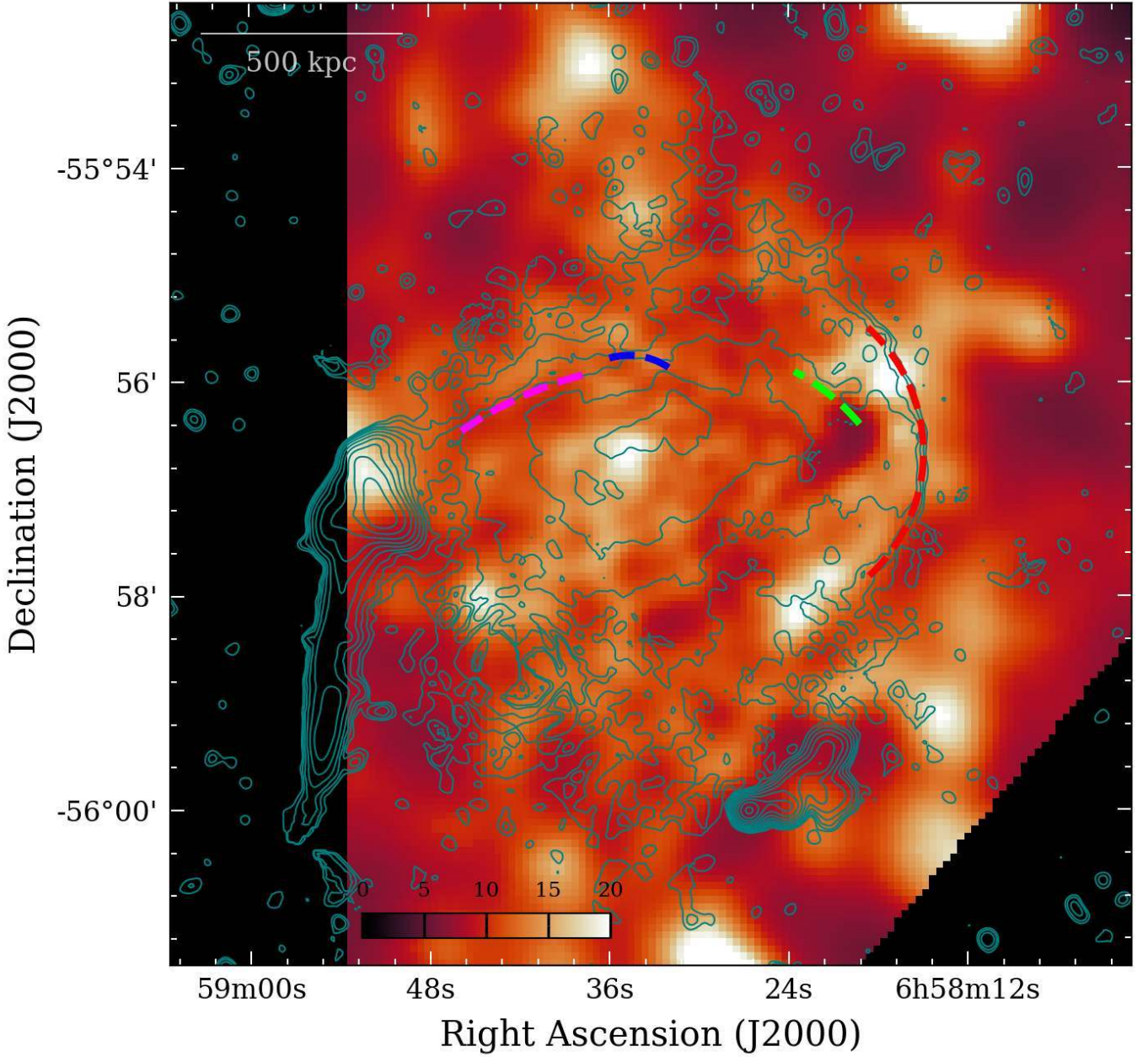
Fig. 6. Temperature map in keV units of the Bullet Cluster derived from the Chandra data following the method described in Markevitch et al. (2000) and Wang et al. (2016). Contours show the radio emission from the MeerKAT discrete source-subtracted image spaced by a factor of 2 starting from 3 \times \text{rms} . Dashed arcs mark the positions of the radio surface brightness discontinuities. The corresponding error map is reported in Appendix. A.
