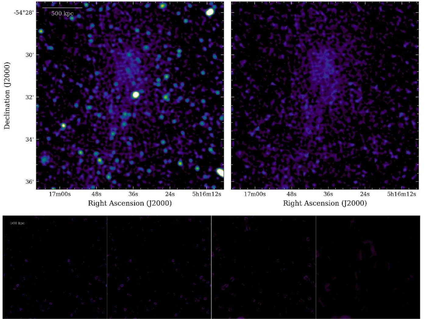
Fig. C.11. Same as Fig. 1 but for J0516.6-5430.
