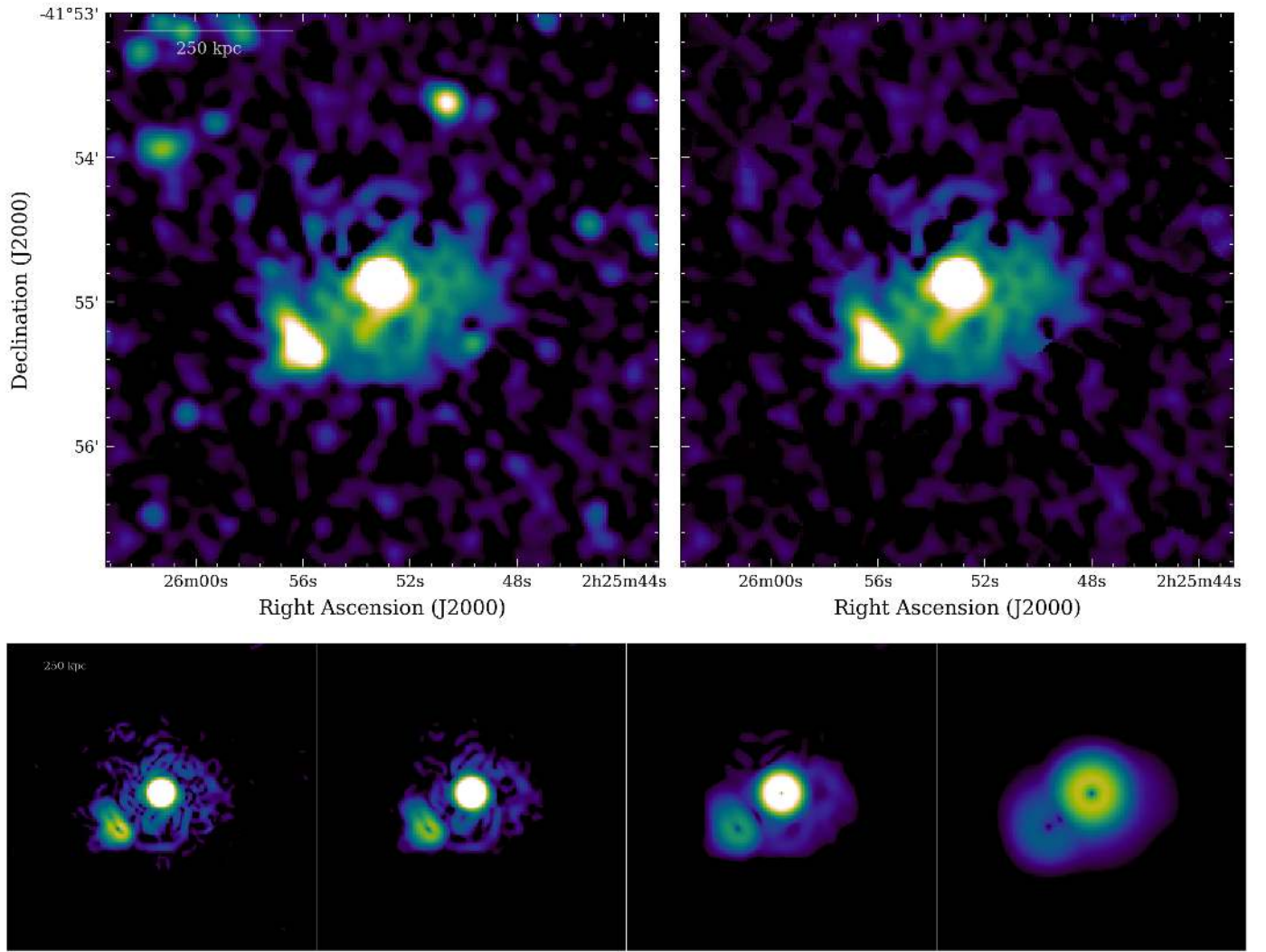
Fig. B.15. Same as Fig. 1 but for J0225.9-4154.
