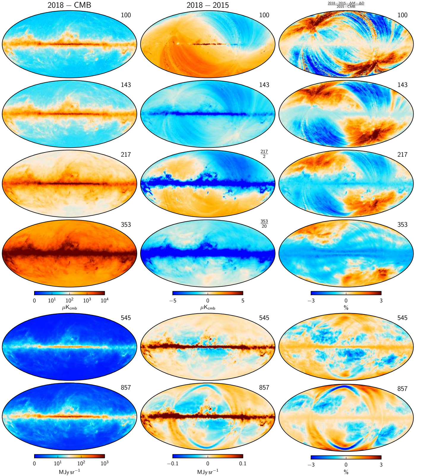
Fig. 3. Comparison of 2018 and 2015 HFI temperature maps, similar to Fig. 2 for LFI. Columns show, from left to right: (1) the difference between the 2018 intensity maps and the 2018 Commander CMB map; (2) the difference between the 2018 and 2015 frequency maps; and (3) the fractional difference between the 2018 and 2015 frequency maps. Note the different temperature scales. Rows indicate results for each of the six HFI frequency channels. All maps are smoothed to a common resolution of 1^\circ FWHM. Note that the 217- and 353-GHz difference maps have been scaled by factors of 1/2 and 1/20, respectively, to conform numerically to the same range as the 100- and 143-GHz maps.
