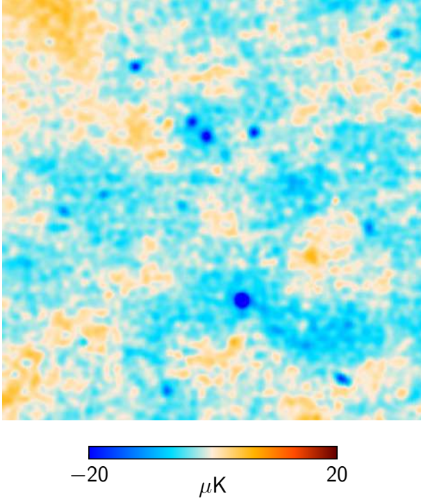
Fig. D.3. Difference between the SMICA CMB map and its SZ-free version. The patch shown is 20^\circ \times 20^\circ centered on (l, b) = (46^\circ, 53^\circ) .
