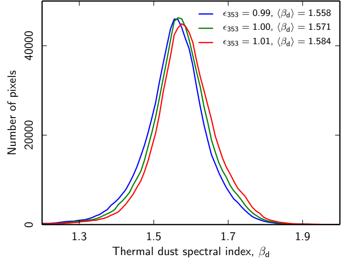
Fig. 30. Effect on the spectral index of polarized thermal dust emission, \beta_d , when changing the polarization efficiency correction at 353 GHz, \epsilon_{353} . A shift of \epsilon_{353} by 1 % translates into a change in \beta_d of 0.013.
