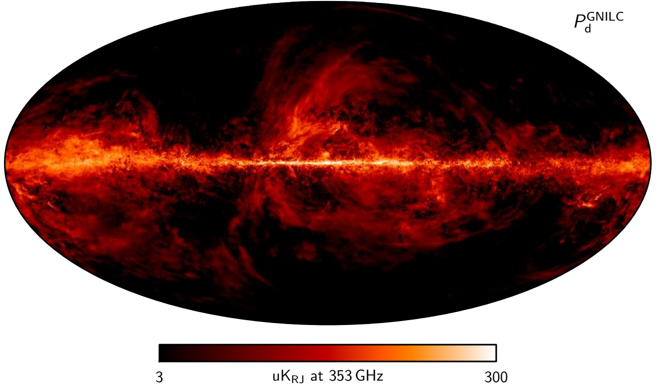
Fig. 27. GNILC 2018 polarized thermal dust amplitude map evaluated at 353 GHz. The angular resolution varies over the sky, as described in Remazeilles et al. (2011b). No colour corrections have been applied to this map.
