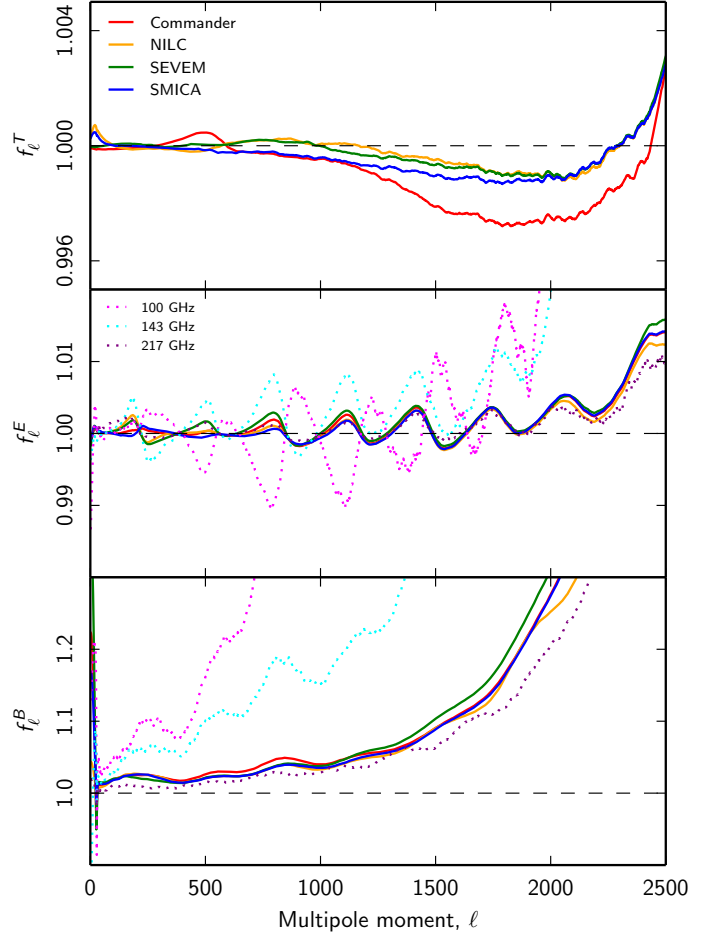
Fig. 11. Effective transfer functions f_\ell for each of the four pipeline CMB maps, after deconvolving a 5' FWHM Gaussian beam and N_{\text{side}} = 2048 HEALPix pixel window. From top to bottom, the panels show results for T , E , and B . In the two bottom panels, the dotted lines show the effective residual transfer functions for the three CMB-dominated HFI frequencies between 100 and 217 GHz, after deconvolving the azimuthally-symmetric QuickBeam-based transfer function and HEALPix pixel window in each case.
