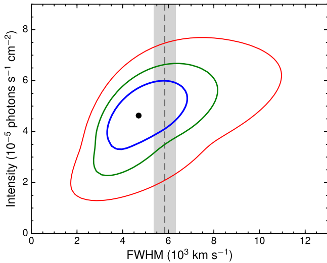
Figure 2. Intensity vs. velocity width contours at the nominal 68%, 90%, and 99% confidence levels ( \Delta C = 2.3 , 4.61, and 9.21, respectively) for the Fe K \alpha emission feature at \sim 6.4 keV. Energy, width, and normalization of the red and blue components on each side of the core were allowed to vary. For comparison, the dashed line and the shaded area indicate the FWHM of the optical H \beta line ( 5850 \pm 480 km s ^{-1} ; from Wandel et al. 1999).
