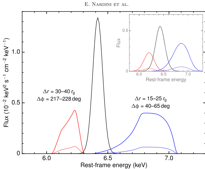
Figure 10. Fe K emission components in the quiescent, red flare, and blue flare spectral states for the hotspot model. The narrow, BLR-like K\alpha from neutral iron at 6.4 keV (in black) is constant, while the highest (solid) and lowest (dashed) intensities are shown for the red and the blue transient features. The radial and azimuthal coordinates of the relative active regions are also printed, for a^* = 0 , i = 30^\circ , and a rest energy of the line of 6.97 keV ( \phi = 0^\circ corresponds to the maximal approaching speed). The profiles are computed assuming an ideal response with linear resolution of 10 eV, while the inset shows their smearing after convolution with the EPIC/pn response (note that the vertical scale is compressed by a factor of two). The intrinsic asymmetry is almost completely lost at CCD resolution.
