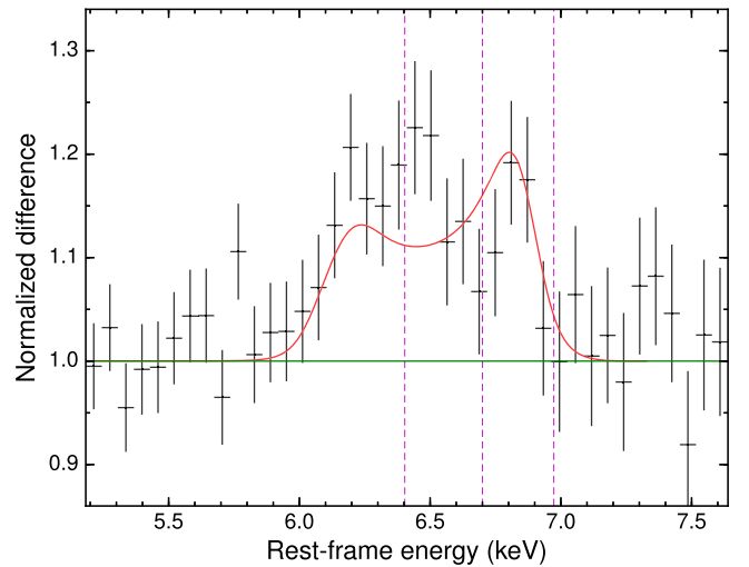
Figure 7. Zoom-in on the Fe K emission band of the “2014–2013” difference spectrum, normalized to take into account the different slopes of the hard X-ray continuum in the two epochs and rebinned for clarity. The correction for the relative energy calibration issues has also been applied. It stands out how the emission-line complex is more prominent in the high-flux state. The variations mainly involve the broad component, although an excess is also seen in proximity of the narrow 6.4 keV core. For comparison, the red curve shows the profile of a disk line with energy of 6.6 keV emitted between 60 and 120 r_g (for \alpha^* = 0 , i = 30^\circ , and q = 3 ; note that this is not a fit). The Fe I, Fe XXV, and Fe XXVI K \alpha positions are traced for guidance.
