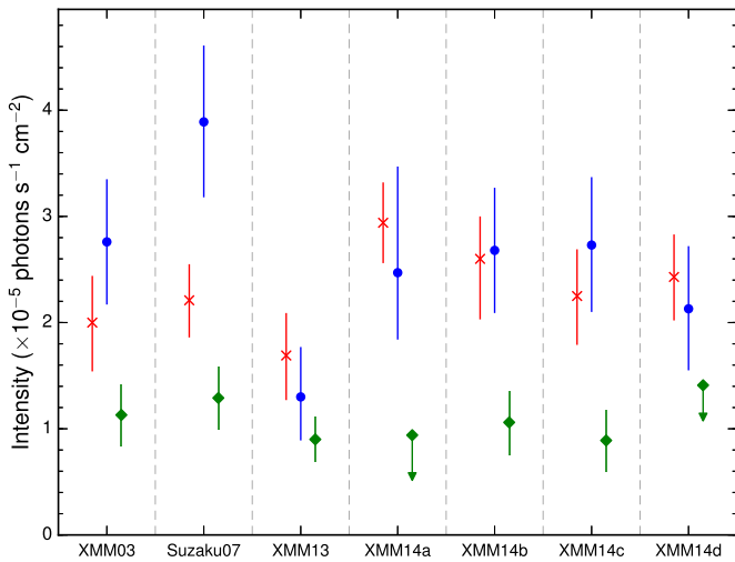
Figure 6. Intensity of the three Fe K \alpha emission features in the 2003, 2013, 2014 XMM-Newton , and 2007 Suzaku spectra of Ark 120: narrow Fe I (6.40 keV, red crosses), tentative Fe XXVI (6.98 keV, green diamonds), and disk line ( \sim 6.5 keV, blue dots). While the two narrow lines have a nearly constant flux, the broad component exhibits a marked drop in 2013, which is significant at the 5\sigma and 2.5\sigma levels compared to 2007 and 2014a, respectively (the plotted error bars correspond to the 90% confidence intervals). For simplicity, a cross-calibration of 1.00 is assumed between XMM-Newton /pn and Suzaku /XIS. This should be correct within 10% (Tsujiimoto et al. 2011).
