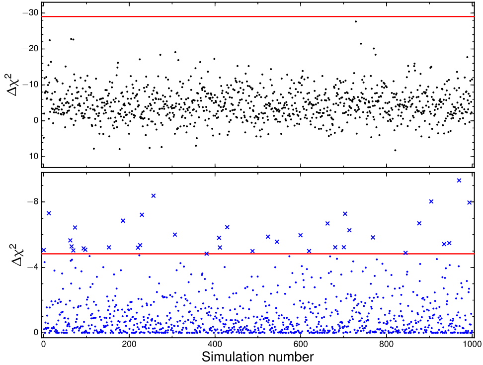
Figure 12. Distributions of \Delta\chi^2 with respect to the null-hypothesis fits obtained from Monte Carlo simulations. Top panel: the three fake spectra (with same exposure, background, and flux of the real quiescent, red flare, and blue flare states) are jointly fitted with both constant “disk line” and variable “hotspot” models. In a single case the statistical improvement is close to, yet still lower than the one found in the real data ( \Delta\chi^2 = -29.0 , red solid line), thus confirming the high significance of the short-term Fe K variability. Bottom panel: the simulated quiescent and red flare spectra are fitted with constant (null hypothesis) and variable intensity of the red Fe K excess. The number of false positives (37/1000) sets a conservative confidence level for the observed variability of the individual transients to 96.3% (see text).
