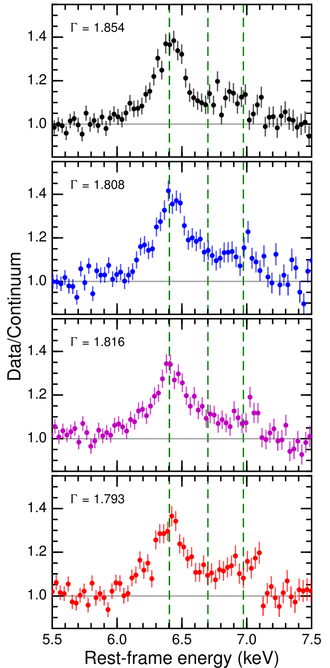
Figure 3. Fe K emission complex in the four consecutive XMM-Newton observations of 2014 March, again obtained as the ratio between the data and the power-law continuum fitted at 3–5 plus 7–10 keV (the best value of the photon index is reported in the left-hand top corner). Compared to the simultaneous, high-resolution Chandra spectrum, the 6.4 keV feature is of course much broader and less prominent, yet the red and blue excesses are still clearly present. Differently from the HEG case, the latter extends with no discontinuity up to at least 7 keV, not only due to the much better signal-to-noise of the XMM-Newton spectra, but also to variability (see Section 4). The data are rebinned to a constant 30 eV resolution, and that the energies are gain-corrected.
