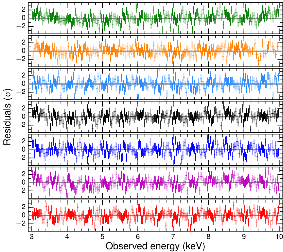
Figure 11. Best-fit residuals (in units of \sigma ; error bars have size 1) for the relline model applied to all the 3–10 keV spectra of Ark 120 (Section 4.1), showing that the continuum can be always well reproduced by a simple power law. In chronological order, from top to bottom: XMM-Newton 2003, Suzaku 2007, XMM-Newton 2013, 2014a, 2014b, 2014c, and 2014d (the same color code of Figures 3 and 5 is used).
