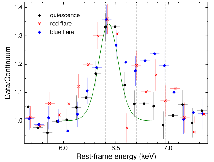
Figure 9. Different profiles of the Fe K emission complex in three 30 ks intervals selected after a visual inspection of the excess emission map in Figure 8, and corresponding to quiescent (dots; 10–40 ks), red flare (crosses; 75–105 ks), and blue flare (diamonds; 253–283 ks) states. Significant changes on short timescales are seen on both sides of the narrow 6.4 keV line (drawn in green), conclusively locating the origin of the broad component(s) from the inner accretion disk. The data are binned by a further factor of three over the adopted 30 eV resolution for visual purposes.
