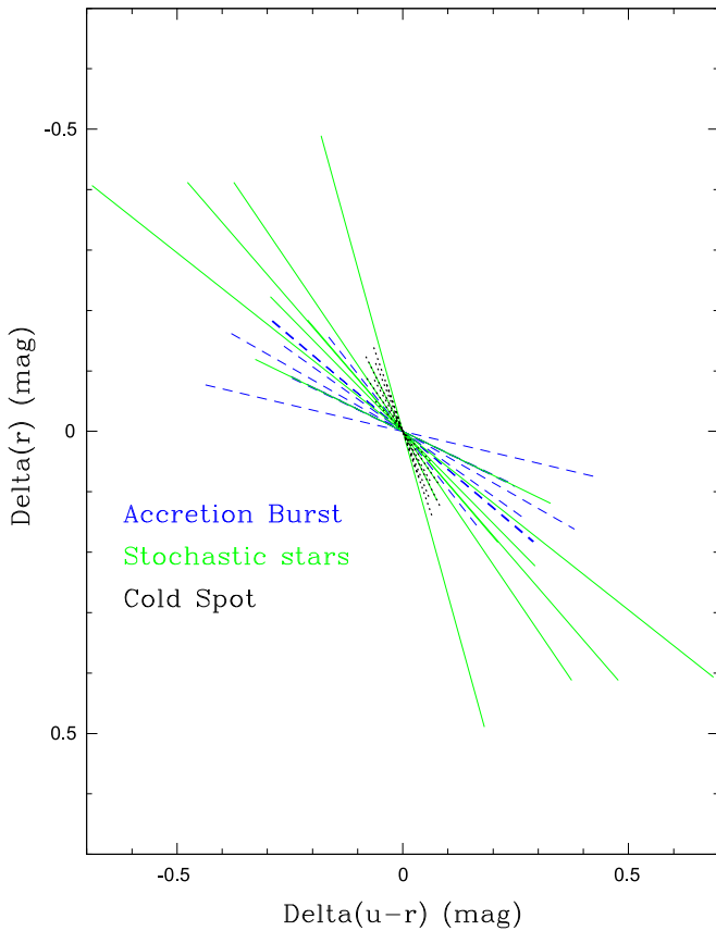
Figure 11. Comparison of the color-slopes ( \Delta r/\Delta(u-r) ) derived from multi-epoch CFHT photometry of NGC 2264 for stars whose CoRoT light curves have stochastic light curves to those that are either dominated by short-duration accretion bursts or by cold photospheric spots. The stochastic stars show very similar slopes to the accretion burst dominated sample, whereas the stars with cold spots have systematically higher slopes (because the spots are very red, leading to little change in (u-r) color for a given change in r magnitude). We have plotted the data for the largest amplitude cold spot light curves in order to be able to derive as accurate a slope as possible. Most stars with cold-spot light curves have significantly smaller amplitudes.
