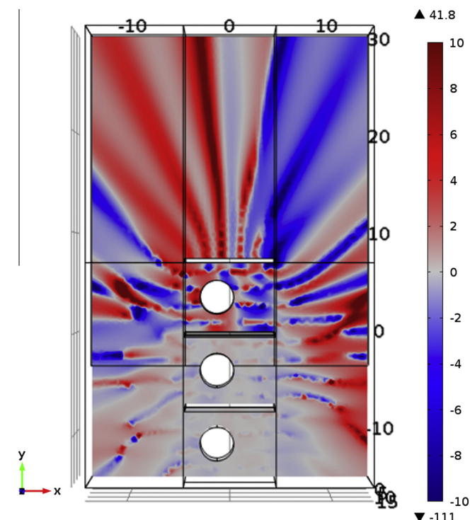
Fig. 14. Noise gain (in dB) after the activation of the ANC system (at 1.5 m from the ground): numerical simulation of a scenario similar to the second experimental tests setting.
