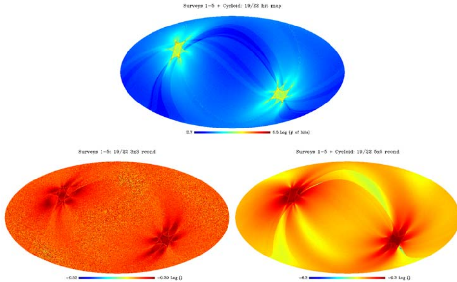
Fig. 3: The hits map (upper), the IQU inverse condition number (bottom left), and the IQUSS inverse condition number (bottom right) for the horn pair 19/22. The sixth survey improves the polarisation mapping in regions of sky which suffer from nearly parallel scanning (cf. IQUSS inverse condition number map in Fig. 2).
