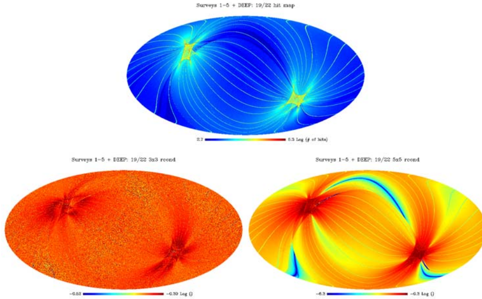
Fig. 4: The hits map (upper), the IQU inverse condition number (bottom left), and the IQUSS inverse condition number (bottom right) for the horn pair 19/22..
