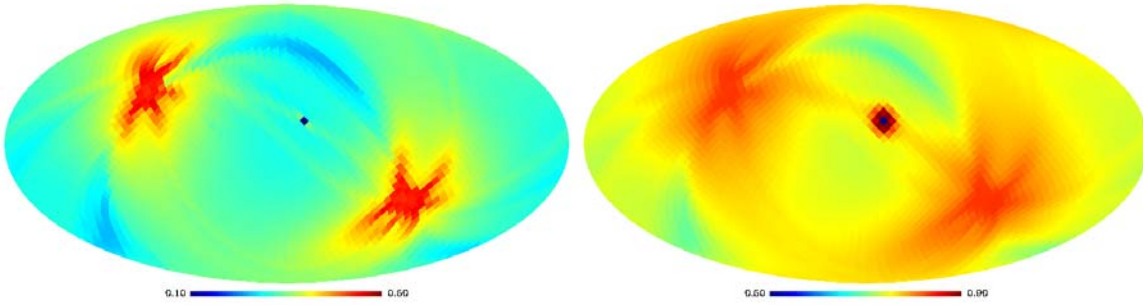
Fig. C3: The TT -covariance for reference pixel 1248 for the 70GHz frequency channel. On the left-hand side is the unsmoothed matrix, while on the right-hand side is the smoothed matrix (beam FWHM of 440 arcmin).
