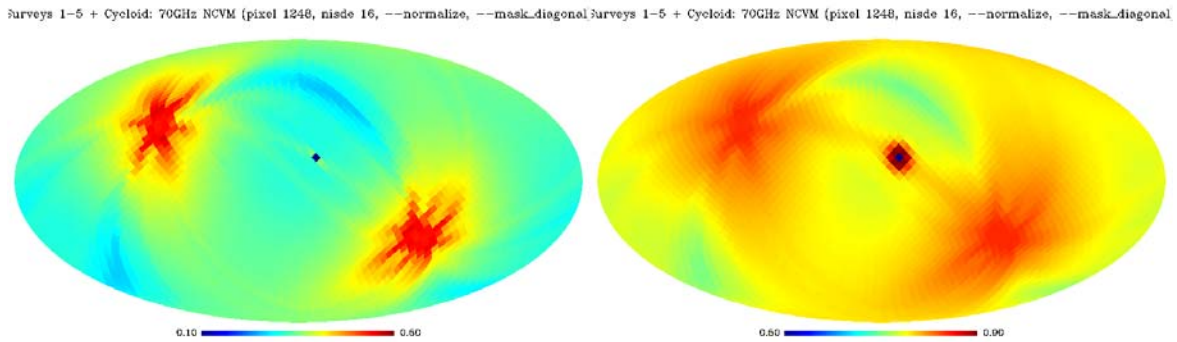
Fig. C5: The TT -covariance for the reference pixel 1248 for the 70GHz frequency channel. On the left-hand side is unsmoothed matrix, while on the right-hand side is the smoothed matrix (beam FWHM of 440 arcmin).
