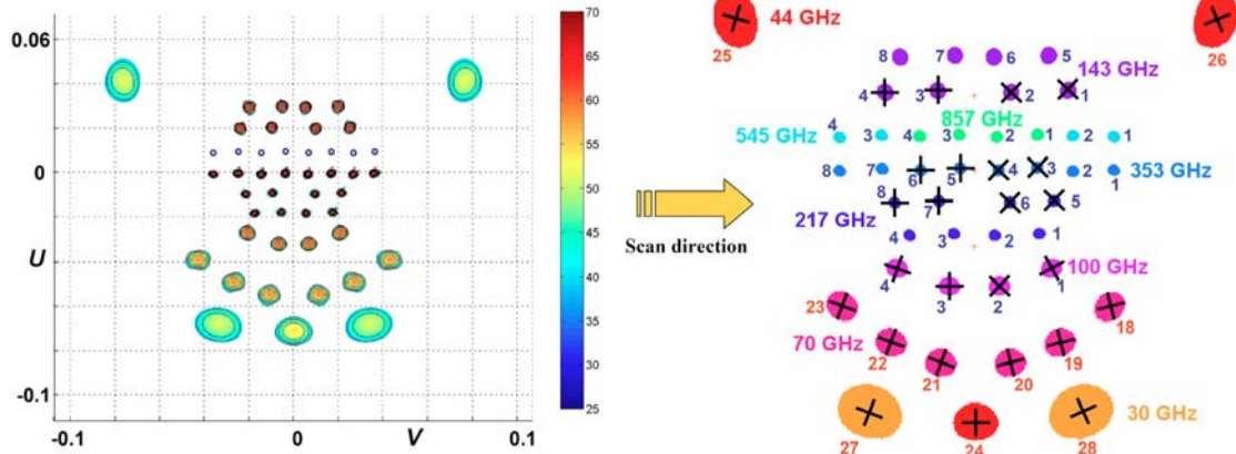
Fig. 5: The PLANCK field of view with beam contour plots (left panel) at the different frequencies (right panel). From Tauber et al. 2010b.
