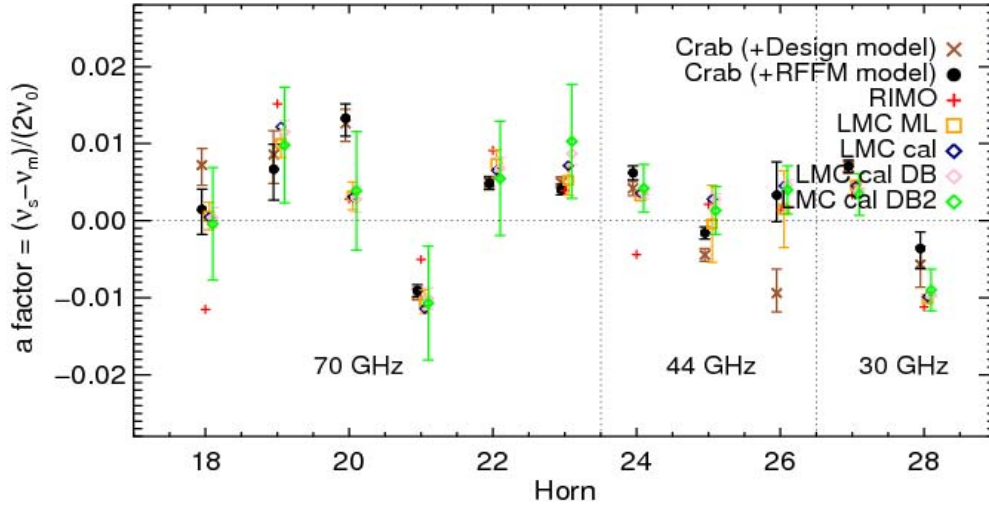
Fig. 1: The a -factors derived using nearly three surveys of data. Values from several different methods are plotted, showing the general agreement, with the LMC “Maximum Likelihood” ML method currently being favoured. The “RIMO” values are based on pre-launch measurements of the bandpass shape and are not expected to be accurate (see Leahy et al 2010).
