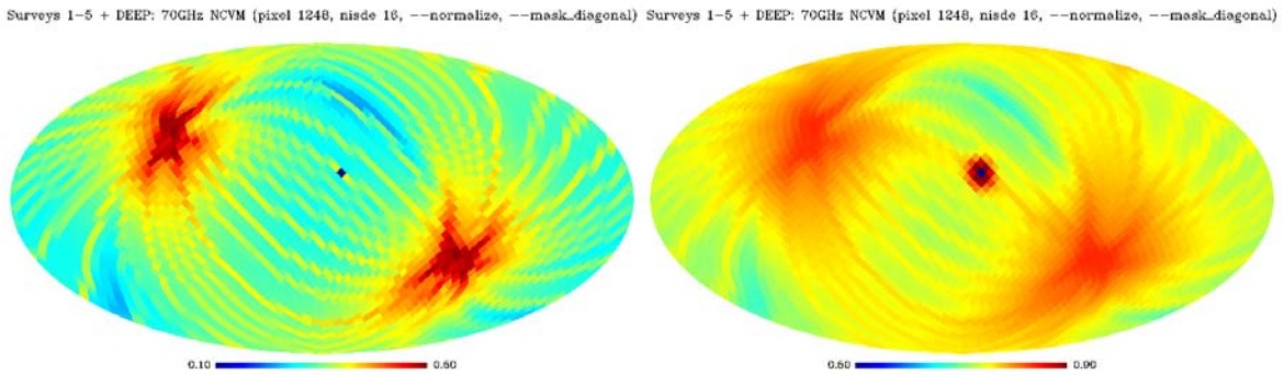
Fig. C7: The TT -covariance for the reference pixel 1248 for the 70GHz frequency channel. On the left-hand side is the unsmoothed matrix, while on the right-hand side is the smoothed matrix (beam FWHM of 440 arcmin).
