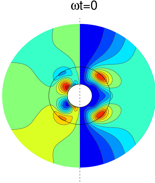
Figure 2. Same as model J, but with a convection zone that extends from x = 0.5 . In this case, C_\alpha = 7.86 , C_\omega = 49.5 , and E_T/E_{\text{tot}} = 0.90 .
