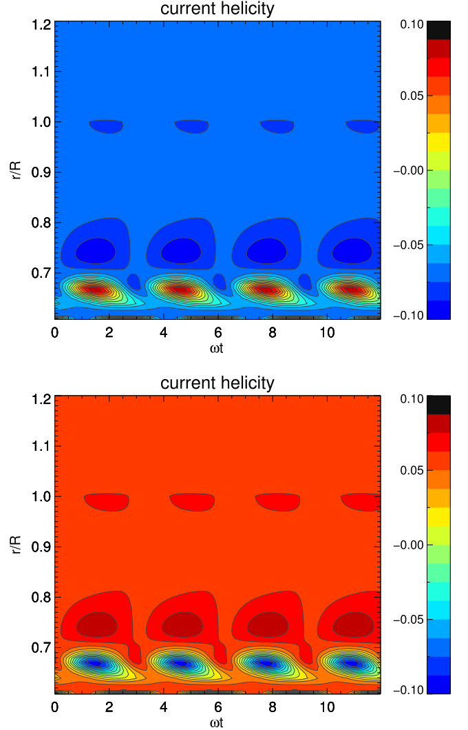
Figure 3. Upper panel: evolution of \mu_0 R \mathbf{J} \cdot \mathbf{B} / \langle B^2 \rangle computed at +30^\circ latitude for an \alpha^2\Omega advection-dominated solar dynamo model with kR = 0.1 , C_\alpha = 3.03 , C_\Omega = 3 \cdot 10^4 , C_u = 400 , and the cycle period is 32 years. Lower panel: same model as in the upper panel, but the opposite hemisphere. Note that the helicity changes sign from the turbulent zone in the interior to the exterior.
