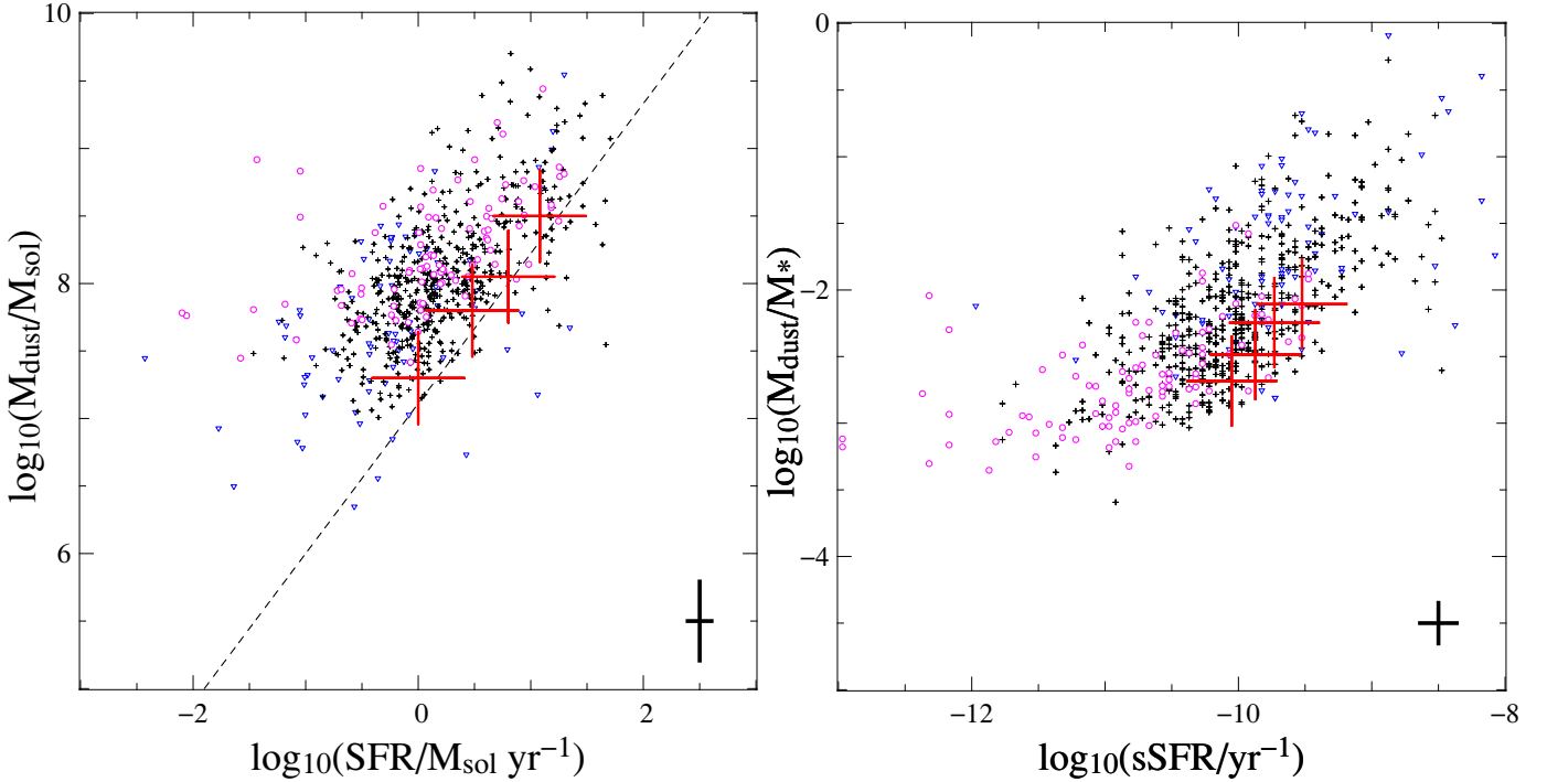
Fig. 11. Dust mass ( M_{\text{dust}} ) vs. SFR for the main sample. Red crosses show the results of Smith et al. (2012) for a sample of \sim 1400 objects selected at 250\ \mu\text{m} from the H-ATLAS survey (Eales et al. 2010) at z < 0.5 . The dashed line shows the best fit obtained in da Cunha et al. (2010) from a sample of about \sim 1700 low redshift galaxies. Blue triangles and the magenta circles show two subsamples of approximately the same size with M_* < 5 \times 10^9 M_\odot and M_* > 5 \times 10^{10} M_\odot , respectively. The cross in the bottom right corner shows the average error.
