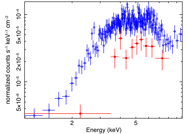
Figure 5. XRT spectra corresponding to the high (blue open circles) and low (red solid circles) states shown in upper panels of Fig. 3.
