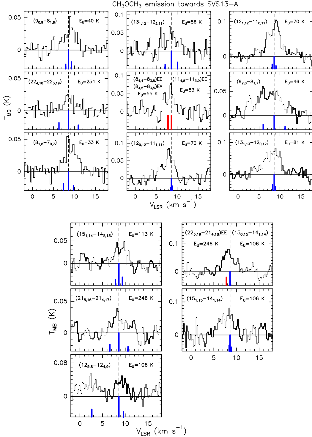
Figure C4. \text{CH}_3\text{OCH}_3 line profiles in T_{\text{MB}} scale (not corrected for the beam dilution); transitions are reported. The vertical dashed line stands for the ambient LSR velocity ( + 8.6 \text{ km s}^{-1} , Chen et al. 2009). The blue lines indicate transitions with the same upper level energies and quantum numbers. The different length is related to the different spin statistical weight of each transitions (see also Subsection 3.2). Red lines indicate transitions with different upper level energies and quantum numbers. Gaussian fit is not performed given the asymmetric line profiles.
