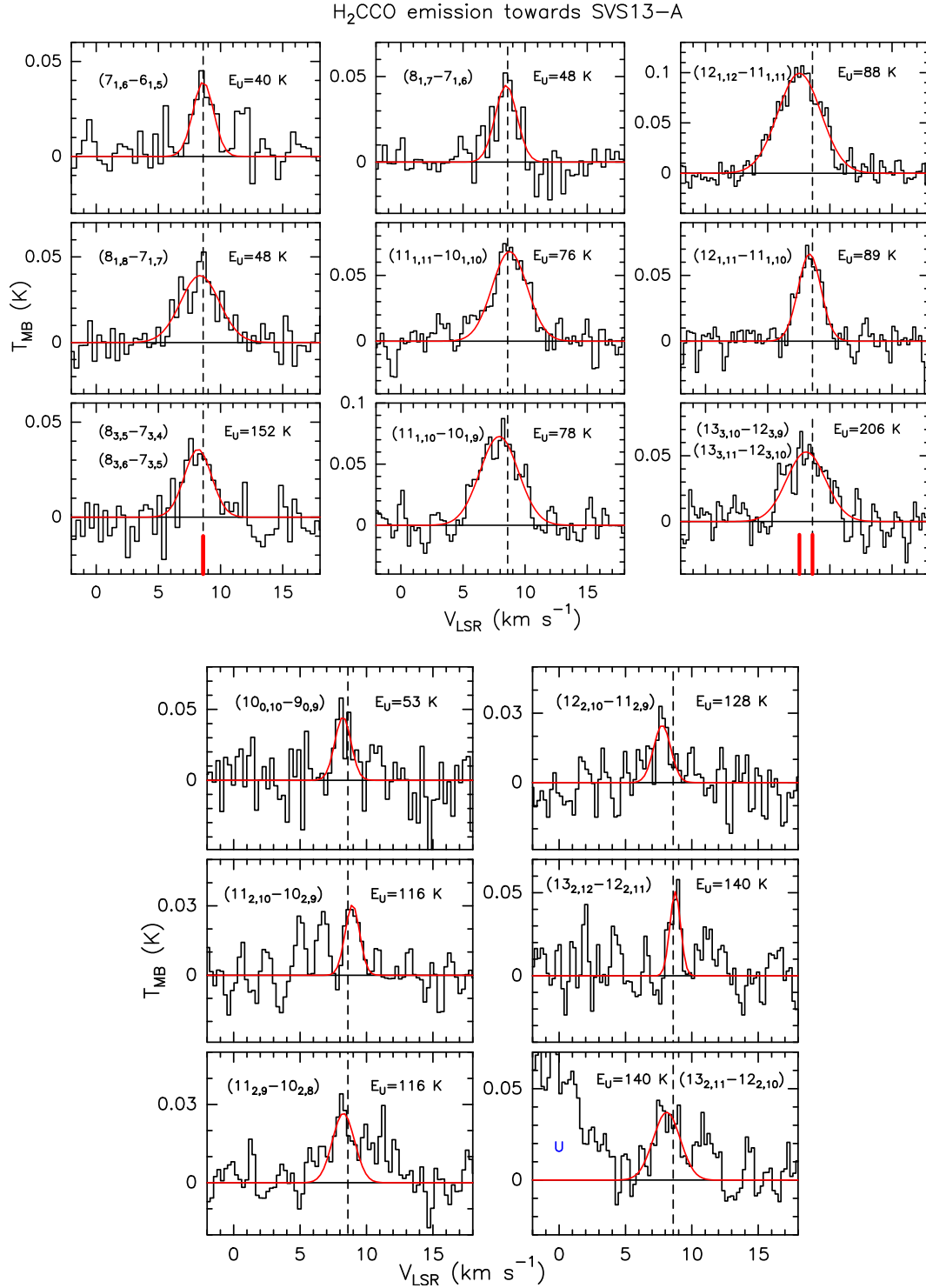
Figure C1. \text{H}_2\text{CCO} line profiles in T_{\text{MB}} scale (not corrected for the beam dilution); transitions are reported. The vertical dashed line stands for the ambient LSR velocity ( +8.6 \text{ km s}^{-1} , Chen et al. 2009). For blended lines, the vertical red solid lines indicate the different transitions. In the upper and lower panel are reported the ortho and it para transitions respectively. Note that the intensity of the para transitions is lower than the ortho ones, consistently with the ratio 1:3 of the statistical weights in the high temperature limit ( T \gg 15 \text{ K} ).
