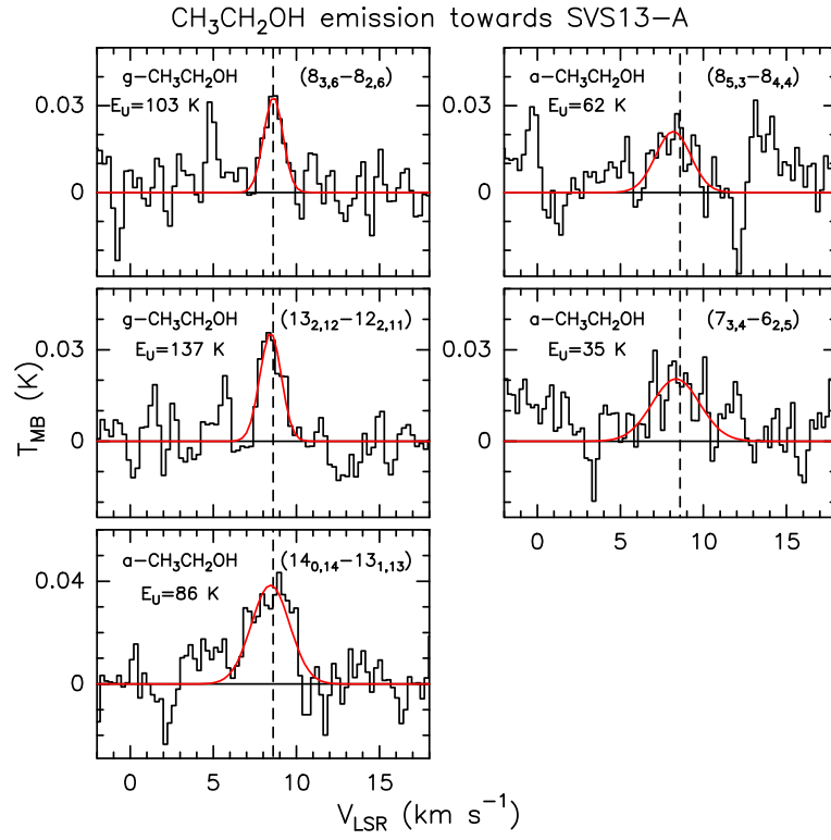
Figure C5. \text{CH}_3\text{CH}_2\text{OH} line profiles in T_{\text{MB}} scale (not corrected for the beam dilution); transitions are reported. The vertical dashed line stands for the ambient LSR velocity ( +8.6 \text{ km s}^{-1} , Chen et al. 2009).
