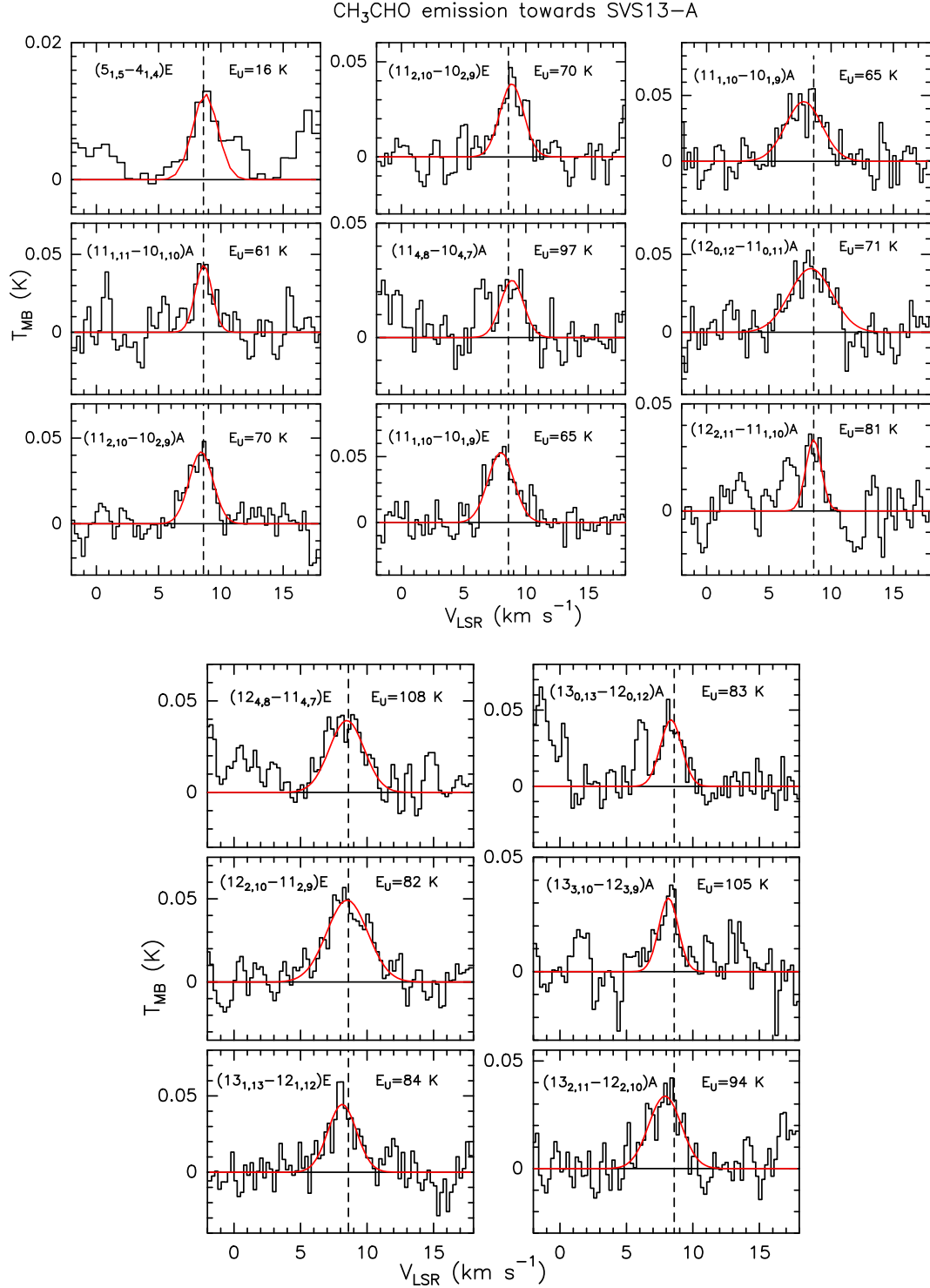
Figure C2. CH 3 CHO line profiles in T_{\text{MB}} scale (not corrected for the beam dilution); transitions are reported. The vertical dashed line stands for the ambient LSR velocity (+ 8.6 Km s -1 , Chen et al. 2009). The 5_{1,5}-4_{1,4} E transition at frequency 93.5953 GHz and the 12_{4,8}-11_{4,7} E transition at 231.4844 GHz are contaminated by unidentified lines and thus excluded from the further analysis.
