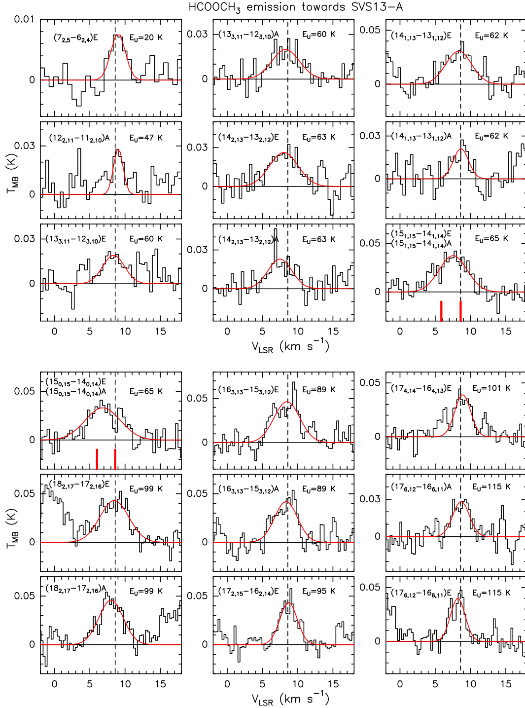
Figure C3. \text{HCOOCH}_3 line profiles in T_{\text{MB}} scale (not corrected for the beam dilution); transitions are reported. The vertical dashed line stands for the ambient LSR velocity ( +8.6 \text{ km s}^{-1} , Chen et al. 2009). For blended lines, the vertical red solid lines indicate the different transitions. All the line profiles due to several transitions with different upper level energies are excluded from the analysis (see text).
