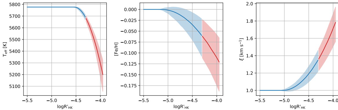
Figure 4. The three panels describe how the stellar parameters T_{\text{eff}} , [\text{Fe}/\text{H}] , and \xi vary as a function of the stellar activity based on the model described in Eq. 2 and the posteriors' distributions obtained through the MCMC simulation. The blue areas represent the 90% confidence intervals within the range of \log R'_{\text{HK}} indexes covered by the stars in our sample, while the red areas are the extrapolations of the same model at higher \log R'_{\text{HK}} values. The solid lines represent the maximum a posteriori estimates. No variation is expected for \log g .
