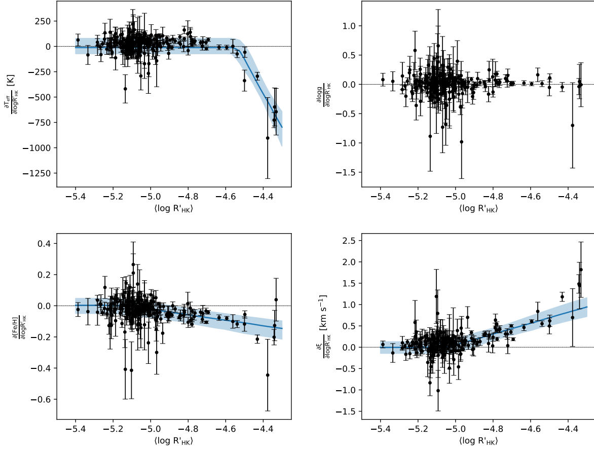
Figure 3. The four panels show the sensitivity of the stellar parameters T_{\text{eff}} , \log g , [\text{Fe}/\text{H}] , and \xi to the chromospheric activity for all the stars in our sample as a function of their typical \log R'_{\text{HK}} index. Blue areas and the blue solid lines represent the posterior-probability 90% confidence intervals of MCMC simulation and the maximum posterior density estimates, respectively.
