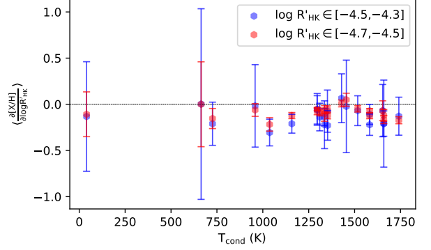
Figure 6. The plot shows the binned-averaged \partial[X/H]/\partial\log R'_{\text{HK}} values and standard deviations calculated for the intervals \log R'_{\text{HK}} \in [-4.7, -4.5] (red) and \log R'_{\text{HK}} \in [-4.5, -4.3] (blue) as a function of the condensation temperature T_{\text{cond}} of the X-element.
