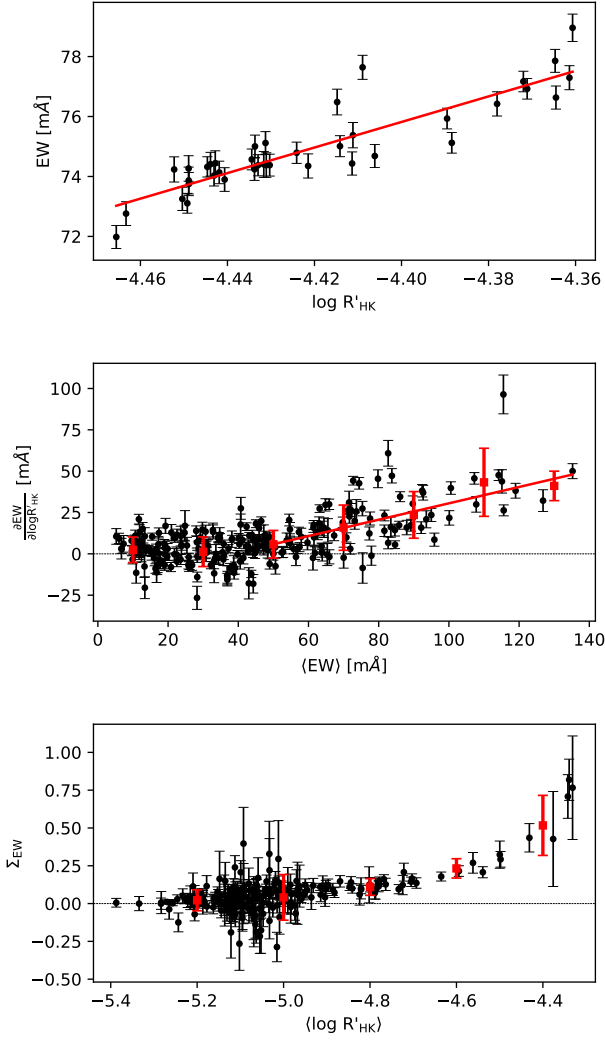
Figure 1. Top. - Equivalent width of the Ba II line at 5853 Å measured from the HARPS spectra acquired for HD59967 as a function of the stellar \log R'_{\text{HK}} index. The EW increases as a function of the stellar activity. The red solid line represents the linear fit of the distribution. Middle. - Black dots are the EW- \log R'_{\text{HK}} slopes (see top panel) of all the lines measured in HD59967 spectra as a function of the median line's EWs (i.e., \langle \text{EW} \rangle ). The averaged values of these slopes at different bins of \langle \text{EW} \rangle are plotted as red squares, while their error bars represent the standard deviations within the bin. Lines with \langle \text{EW} \rangle \gtrsim 50 mÅ have EW- \log R'_{\text{HK}} slopes that increase with \langle \text{EW} \rangle . The linear fit of the distribution traced by absorption featured with \langle \text{EW} \rangle > 50 mÅ is plotted as a red solid line. We refer to its slope value as \Sigma_{\text{EW}} . Bottom. - Black dots are the \Sigma_{\text{EW}} for all stars in our sample as a function of their median \log R'_{\text{HK}} index. Red squares and their error bars represent the binned-averaged \Sigma_{\text{EW}} values the standard deviations at different intervals of \langle \log R'_{\text{HK}} \rangle .
