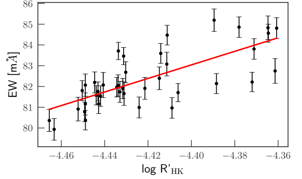
Figure 2. Same of Fig. 1-Top, but here Voigt profiles have been used to measure the EWs of the Ba II line instead of Gaussians.
