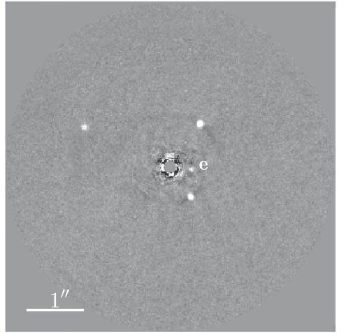
Figure 4. Demonstration of the functionality of our LEECH data processing pipeline on an HR 8799 data set. We detect all four directly imaged planets at high significance even though the data were collected using only one side of the telescope under poor conditions (seeing \gtrsim 1.5'' ). The innermost planet “e” (labeled) is separated by less than 0.4'' and is detected with a signal-to-noise ratio of 7.5.
