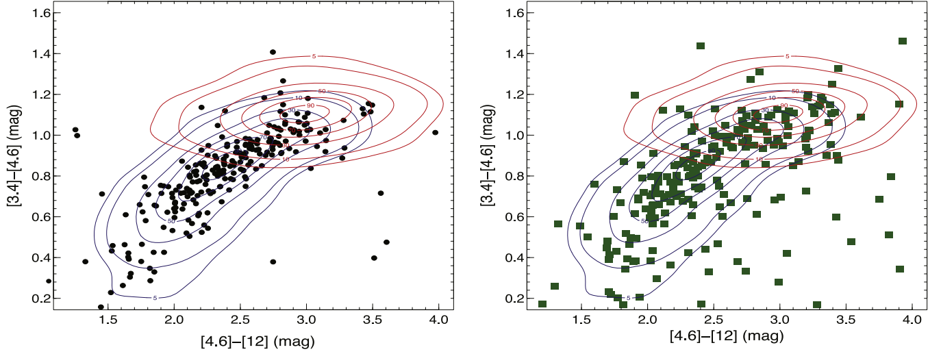
Figure 7. Isodensity contours drawn from the KDE technique for the Fermi -Roma-BZCAT blazars (i.e., training sample) that constitute the WISE \gamma -ray Strip (Massaro et al. 2011a) in the [3.4]-[4.6]-[12] \mu\text{m} color-color plot. Blue contours were computed from the infrared colors of the BZBs while the red ones were derived from the BZQs. The infrared colors of the sources classified as BCN (top—black circles) and unc (bottom—green squares) are also reported to show their consistency with the WISE \gamma -ray Strip. The numbers appearing close to each contour correspond to the values of \pi_{\text{KDE}} in both panels. The last contour correspond to 95% confidence level (see Section 7 for details). A similar analysis for the active galaxies of uncertain type listed in 2FGL was already performed in Massaro et al. (2012a). Here this study has been repeated for both 1FGLR and 2FGLR, and the refined association list of the Fermi catalogs.
