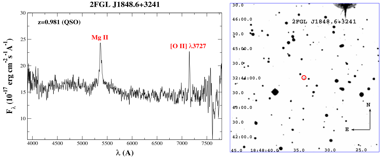
Figure 12. (Upper panel) Optical spectra of the counterparts associated with 2FGL J1848.6+3241 observed at OAN in San Pedro Mártir (México) on 2014 July 2. The emission lines marked allowed us to estimate their redshift. The source has been classified as a QSO. (Lower panel) 5' \times 5' finding chart from the Digitized Sky Survey (red filter). The potential counterpart of 2FGL J1848.6+3241 is indicated by the red circle.
