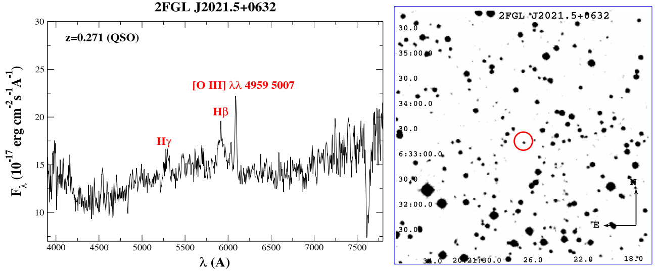
Figure 13. (Upper panel) Optical spectra of the counterparts associated with 2FGL J2021.5+0632 observed at OAN in San Pedro Mártir (México) on 2014 July 2. The emission lines marked allowed us to estimate their redshift. The source has been classified as a QSO. (Lower panel) 5' \times 5' finding chart from the Digitized Sky Survey (red filter). The potential counterpart of 2FGL J2021.5+0632 is indicated by the red circle.
