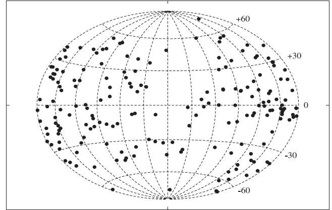
Figure 21. All-sky distribution of the remaining UGSs with no \gamma -ray analysis flags in the refined association list of the Fermi catalogs.
