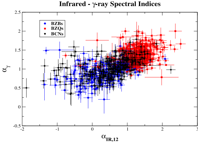
Figure 19. Scatter plot of the infrared spectral index evaluated using the first two WISE bands vs. the \gamma -ray index for the blazar-like sources in our merged list of refined Fermi associations. Spectroscopically confirmed BZBs and BZQs are shown in blue circles and red squares, respectively, while BCN sources are black diamonds.
