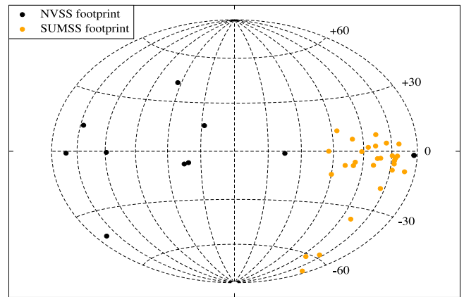
Figure 22. All-sky distribution of the 40 UGSs that do not have any NVSS and/or SUMSS radio source within their positional uncertainty regions at 95% level of confidence and do not present any \gamma -ray analysis flag. We show those lying in the NVSS footprint (i.e., decl. greater than -40^\circ ) as black circles while the others in the Southern hemisphere are indicated as orange circles.
