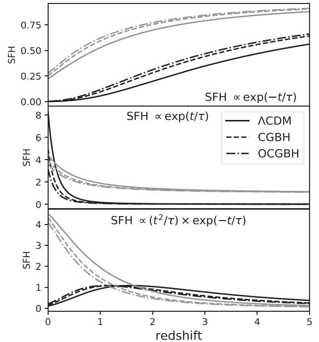
Figure 7. Three different parametrizations for the SFH in the standard and LTB models versus redshift. Each panel represents one of the following SFHs: exponentially decreasing law (top panel), inverted- \tau law (middle panel) and delayed SFH (bottom panel). The black and grey lines respectively represent two values for \tau , 2 and 9 Gyr. \tau is the time-scale related to when the star formation began. The cosmological models are indicated by the line types: solid for \Lambda CDM, dashed for CGBH and dash-dotted for OCGBH.
