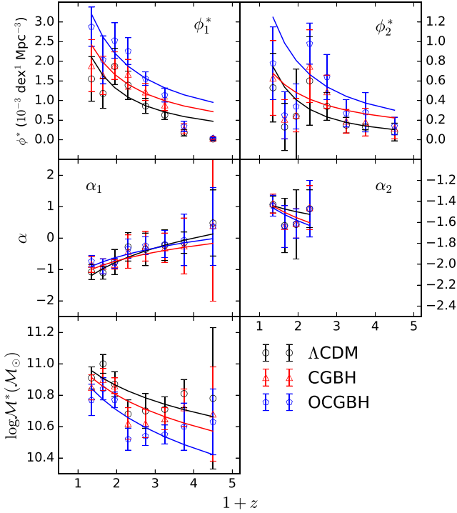
Figure 9. Redshift evolution of the five parameters of the double-Schechter function, \phi_1^* , \phi_2^* , \alpha_1 , \alpha_2 and \log \mathcal{M}^* of this work. Note that \alpha_2 only has four points, because after z = 2 this parameter is no longer well-constrained and its value is fixed to -1.6 .
