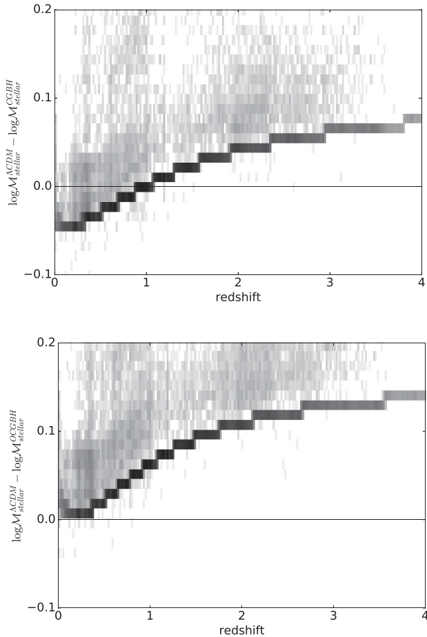
Figure 6. Average variation on the stellar masses from the CGBH model (up panel) and the OCGBH one (down panel) versus redshift. The solid line simplifies the correlation with Fig. 2. The darker region is where most of the galaxies are located. Note that this plot is a result of the output from Le Phare , so no completeness cut was applied.
