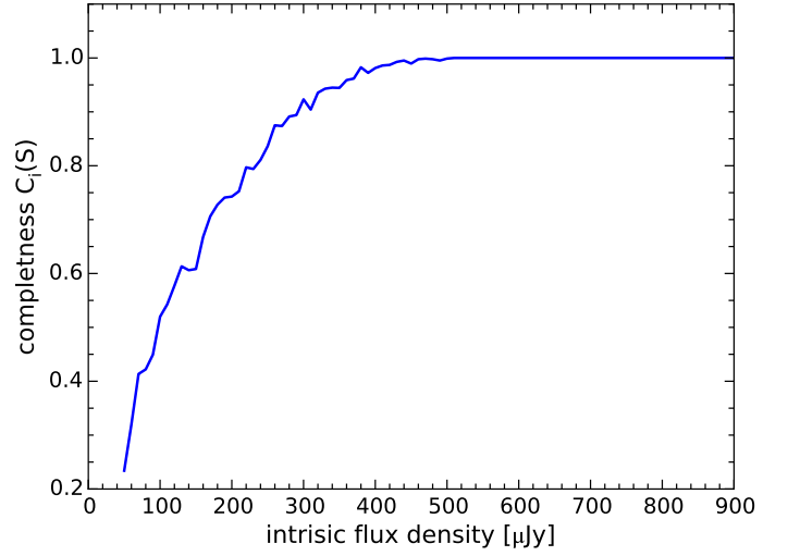
Fig. 3. Completeness C_i(S) as a function of the flux density S , estimated from simulations. The solid curve is the result for field a with \text{rms} = 7.8 \mu\text{Jy/beam} .
