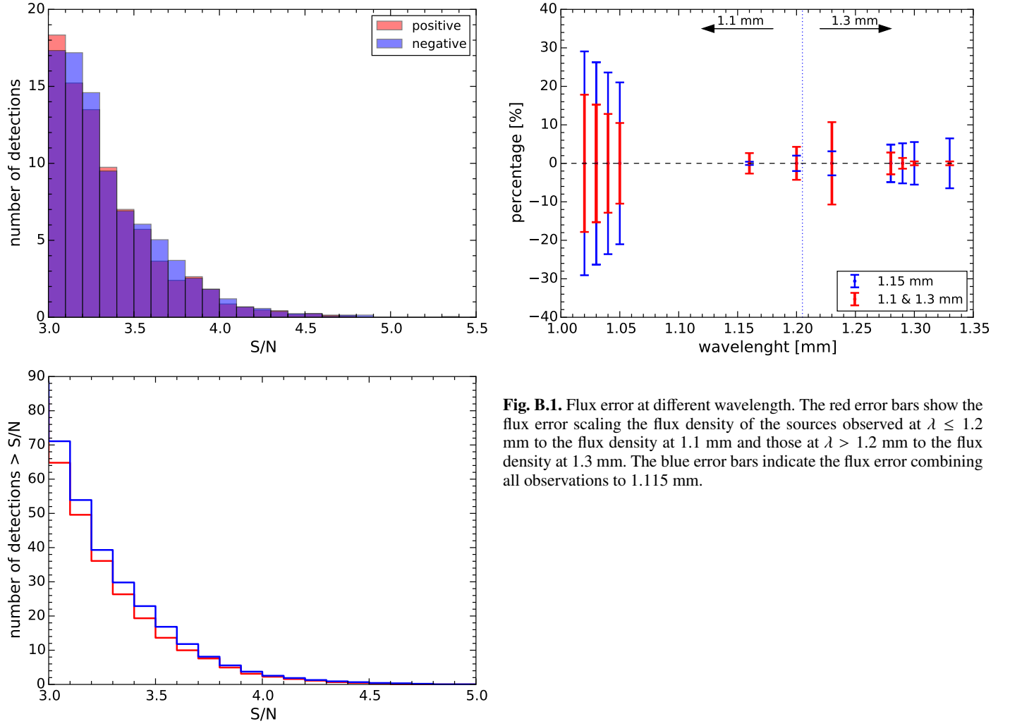
Fig. A.1. Top: number of positive (red) and negative (blue) sources detected in 300 continuum pure noise maps and normalised for 18 continuum maps. Bottom: cumulative distribution of positive (red) and negative (blue) detections.
