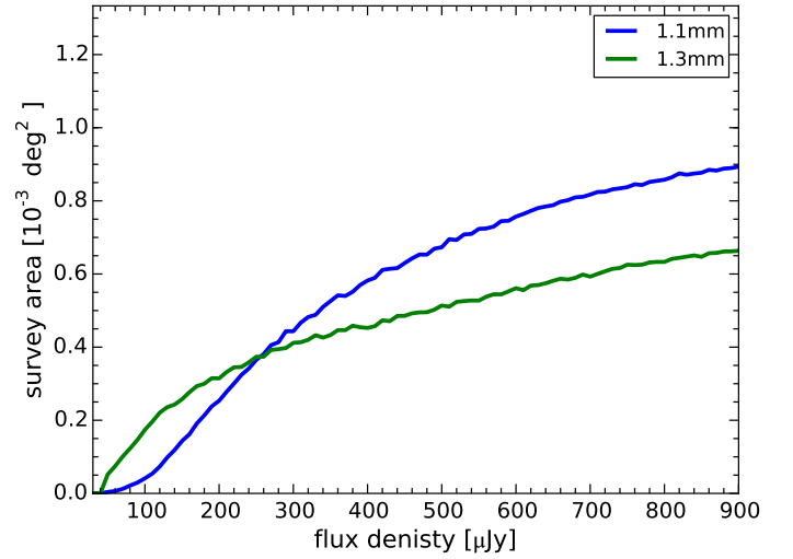
Fig. 4. Effective survey area as a function of intrinsic flux density. This is the area over which a source with an intrinsic flux density S can be detected with S/N > 3.5\sigma . The blue and green curves are the survey areas for the maps at 1.1 mm and 1.3 mm, respectively.
