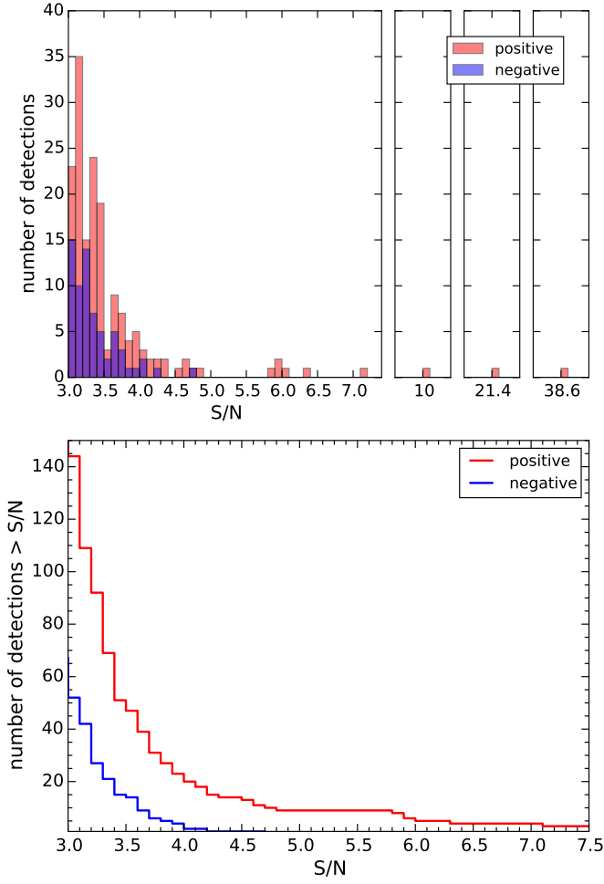
Fig. 2. Top : number of positive (red) and negative (blue) sources detected in the 18 continuum maps, as a function of S/N. Bottom : cumulative distribution of positive (red) and negative (blue) detections.
