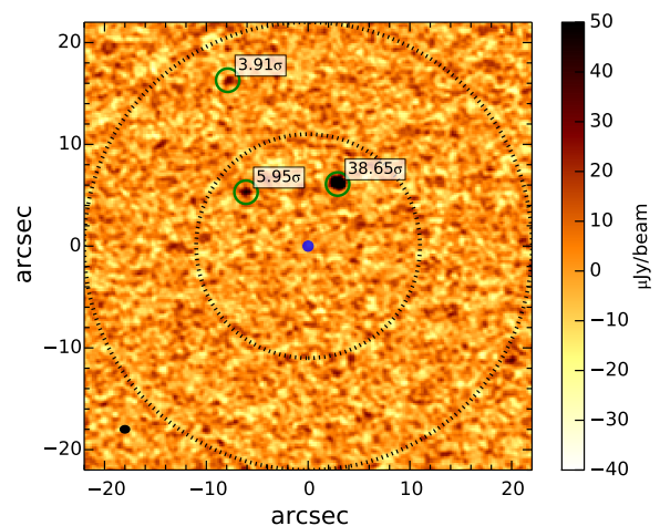
Fig. 1. Example of a Band 6 continuum map obtained with ALMA (Field a Table 1). The green circles represent the sources detected with S/N > 3.5\sigma that also fulfil the requirement of having a size consistent with the beam (or marginally resolved). The inner black dotted circle indicates the primary beam and the outer circle shows twice the primary beam. The blue filled circle shows the masked region. The synthesised beam is indicated by a filled black ellipse in the lower left corner of the plot.
