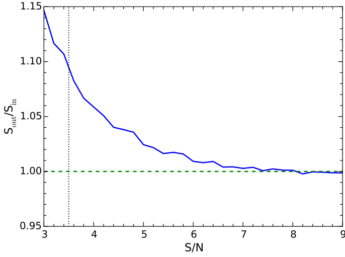
Fig. 5. Flux-boosting factor as a function of S/N, estimated from simulations. The horizontal dashed line corresponds to S_{\text{out}} = S_{\text{in}} . The vertical dashed line corresponds to the detection threshold, S/N = 3.5 .
