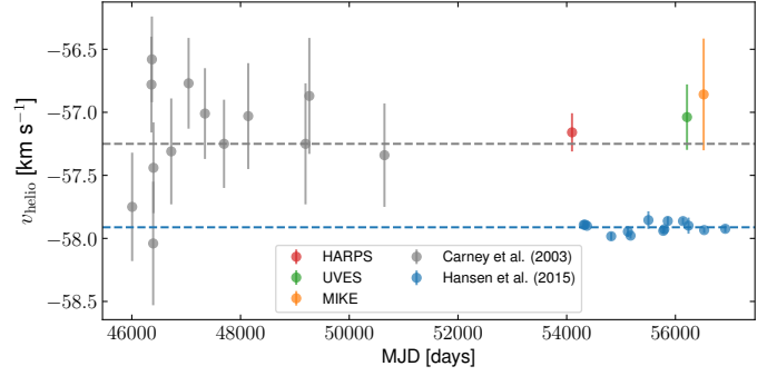
Fig. 2. Comparison of literature time series for v_{\text{helio}} by Carney et al. (2003, gray-filled circles) and Hansen et al. (2015, blue-filled circles) to measurements from the three spectra employed throughout this study (see legend). The gray and blue dashed lines resemble the median values for the two reference samples.
