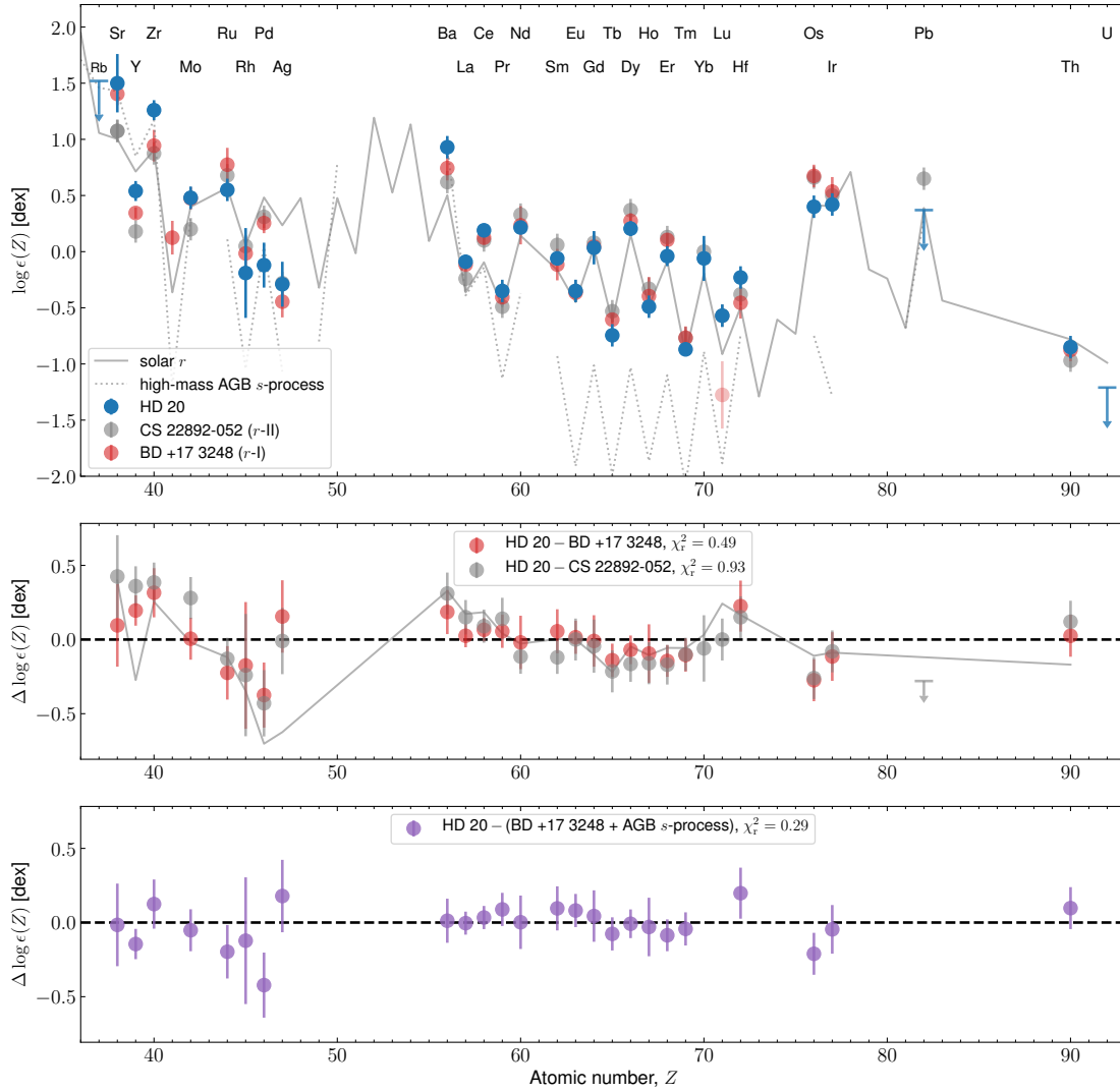
Fig. 18. Neutron-capture abundance pattern in LTE. Upper panel: HD 20’s heavy element abundances are indicated in blue. Shown in gray and red are abundances of the r -II star CS 22892–052 by Snedden et al. (2003) and the r -I star BD +17 3248 by Cowan et al. (2002) with updates from Cowan et al. (2005) and Roederer et al. (2010) . The omitted Lu abundance for BD +17 3248 (see main text) is depicted in light red. Both patterns were scaled to achieve the overall best match to HD 20 in the entire considered range. The gray solid line denotes the solar-scaled r pattern from Snedden et al. (2008) and the best-fit AGB model (see text) is represented by dotted lines. Middle panel: residual pattern between HD 20 and the solar r pattern (gray line), CS 22892–052 (gray), and BD +17 3248 (red). Lower panel: residual pattern after mixing a contribution from BD +17 3248 with s -process material from the AGB yield model.
