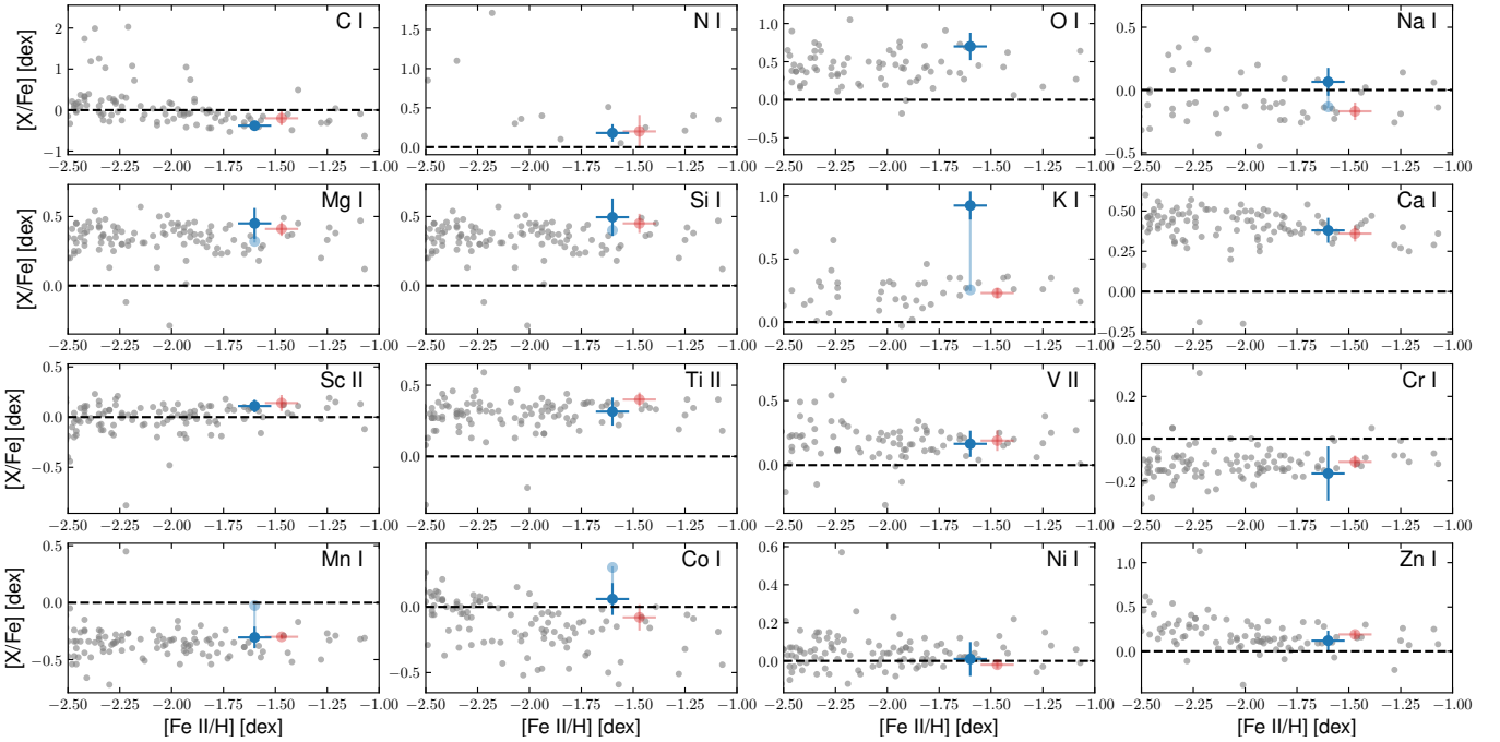
Fig. 16. Comparison of HD 20 (blue circle) to the metal-poor field star compilation (gray dots) by Roederer et al. (2014) and the red horizontal branch star HD 222925 (Roederer et al. 2018b, red circle). Dark blue circles and error bars indicate the result in LTE while the light blue circles indicate the NLTE-corrected ones. In the reference samples, corrections have been applied to O I, Na I, and K I. On the abscissa we show abundances from Fe II since these are less prone to departures from the LTE assumption (Sect. 3.3).
