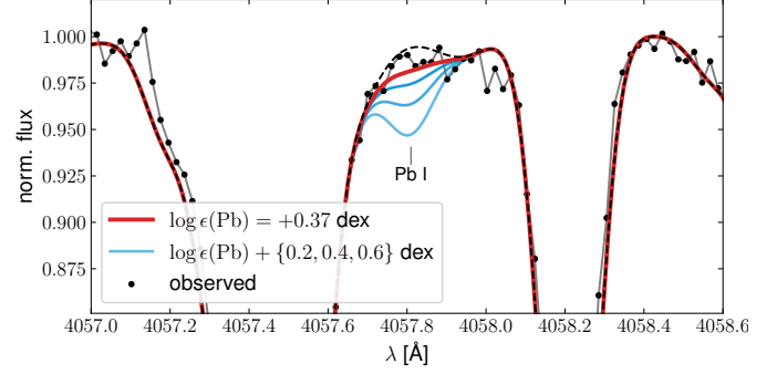
Fig. 12. Same as Fig. 11 but for the Pb I transition at 4057.8 Å and an upper limit of +0.37 dex.
